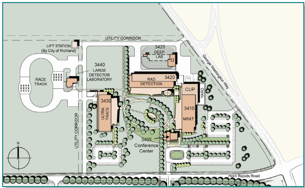
Figure 3. PSF New Construction Site Plan
