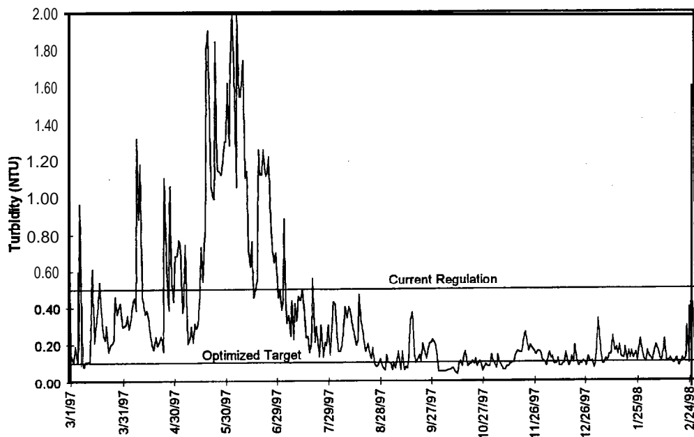
FIGURE 4. Daily maximum finished water turbidity.
