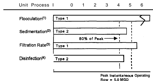
FIGURE 4-10. Performance potential graph for Plant A.
