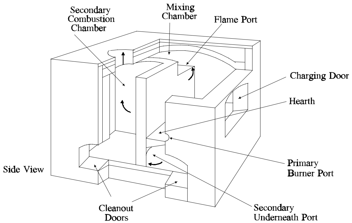
Figure 2.3-2. Excess Air Incinerator
