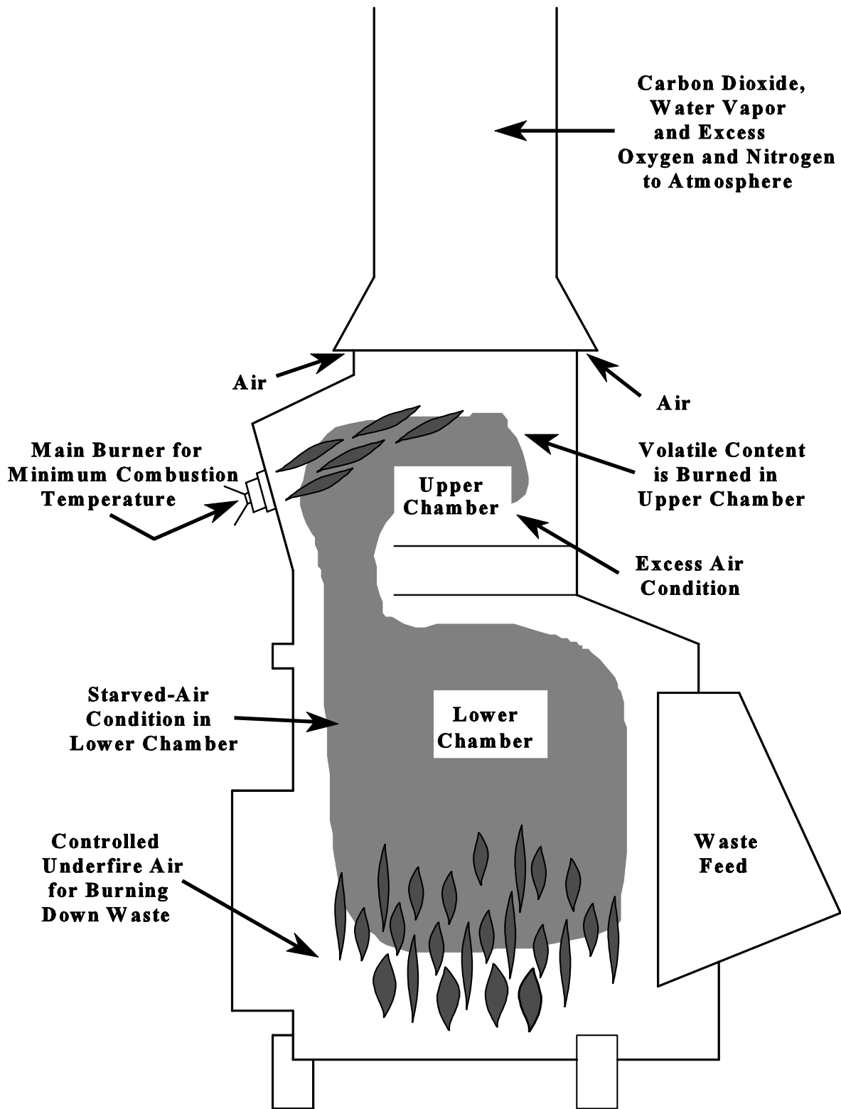
Figure 2.3-1. Controlled Air Incinerator
