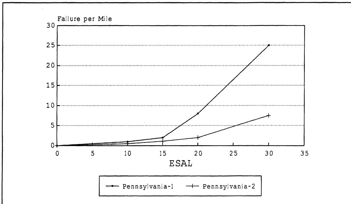
Figure 116. Performance prediction for sample sections in Pennsylvania.
