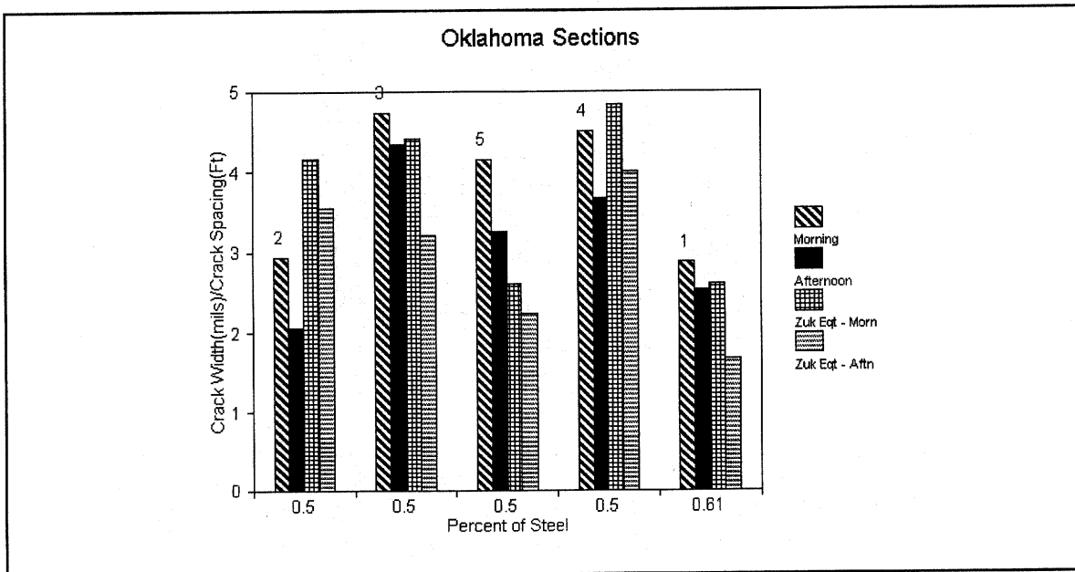
Figure 104. Variation in crack width/crack spacing ratio with percent reinforcement for Oklahoma sample sections.
