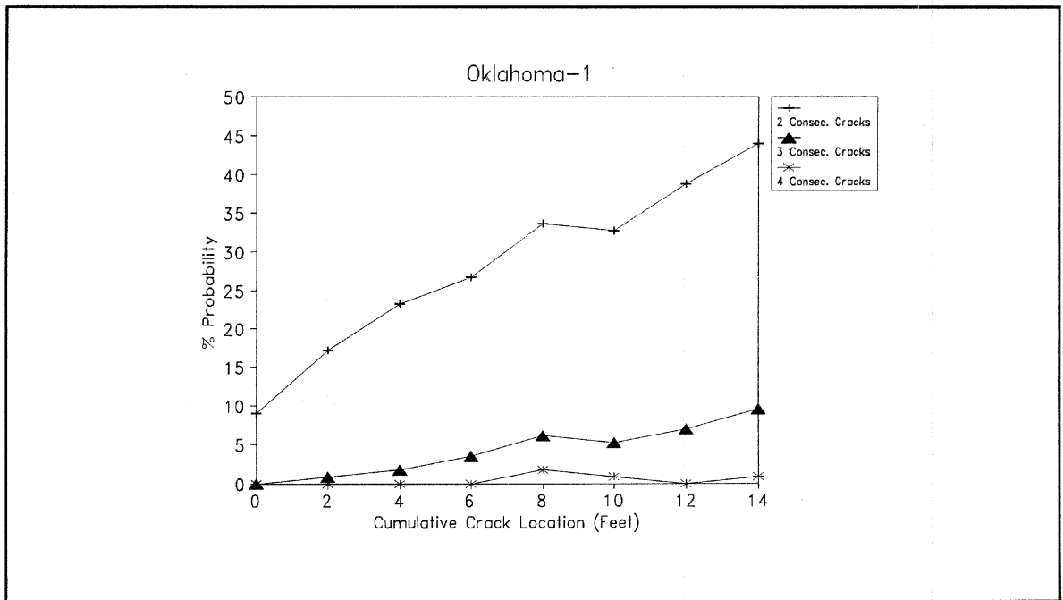
Figure 86. Probability of cluster cracking: sample section Oklahoma-1.
