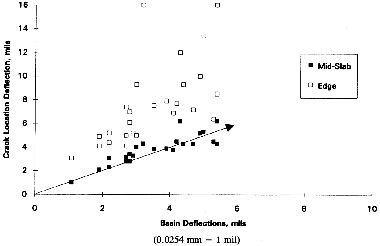
Figure 3. Comparison of basin and crack location deflections.
