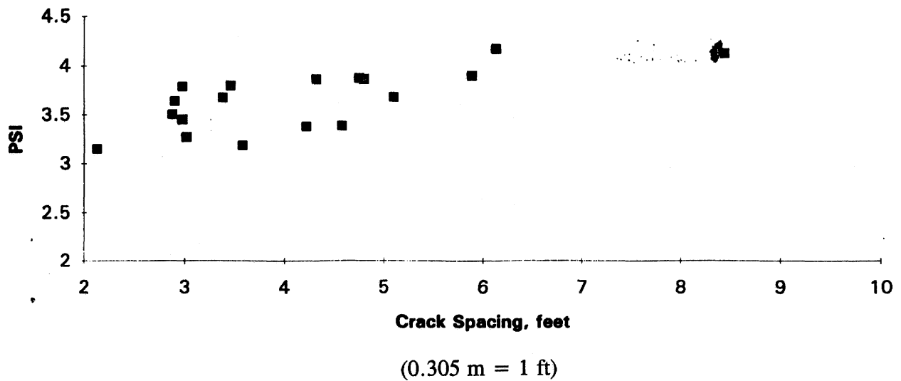
Estimated PSI as a function of average crack spacing.
