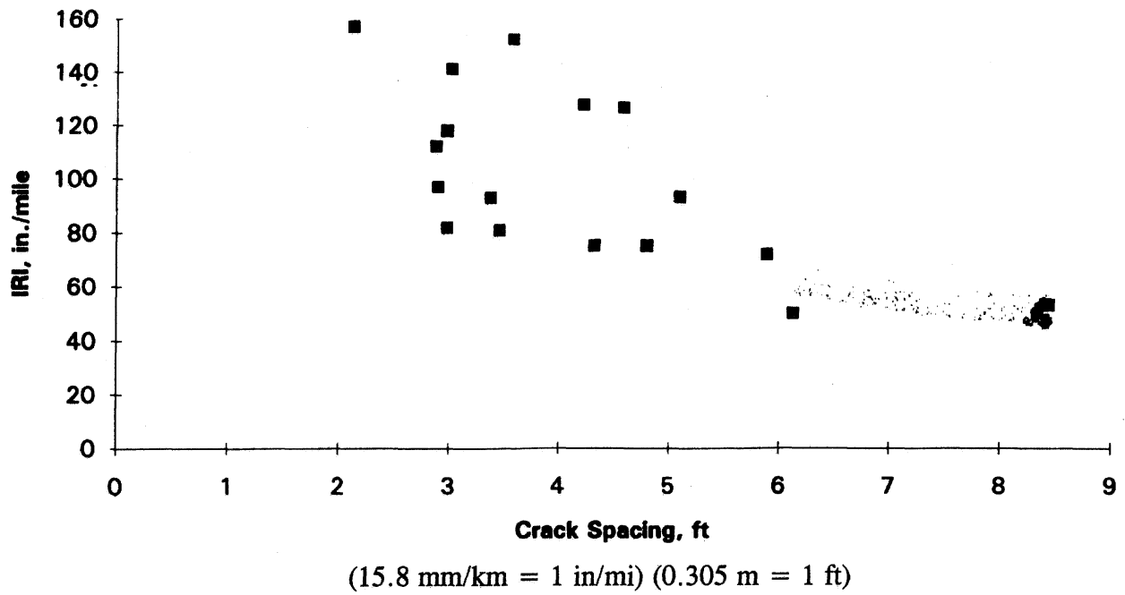
Ride quality (IRI) as a function of average crack spacing.
