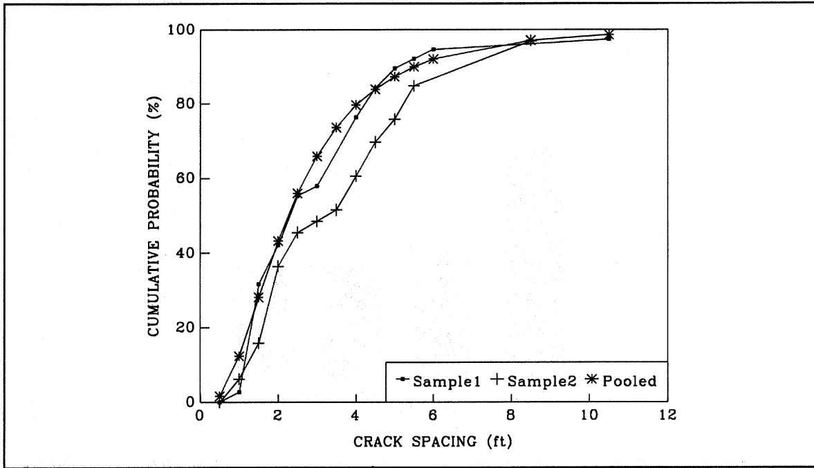
Figure 74. Field cracking distribution data: sample section Iowa-2.
