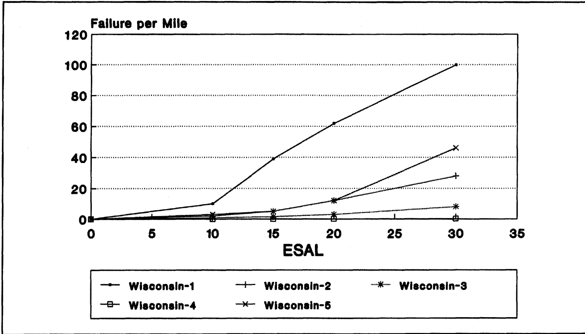
Figure 141. Performance prediction for sample sections in Wisconsin.
