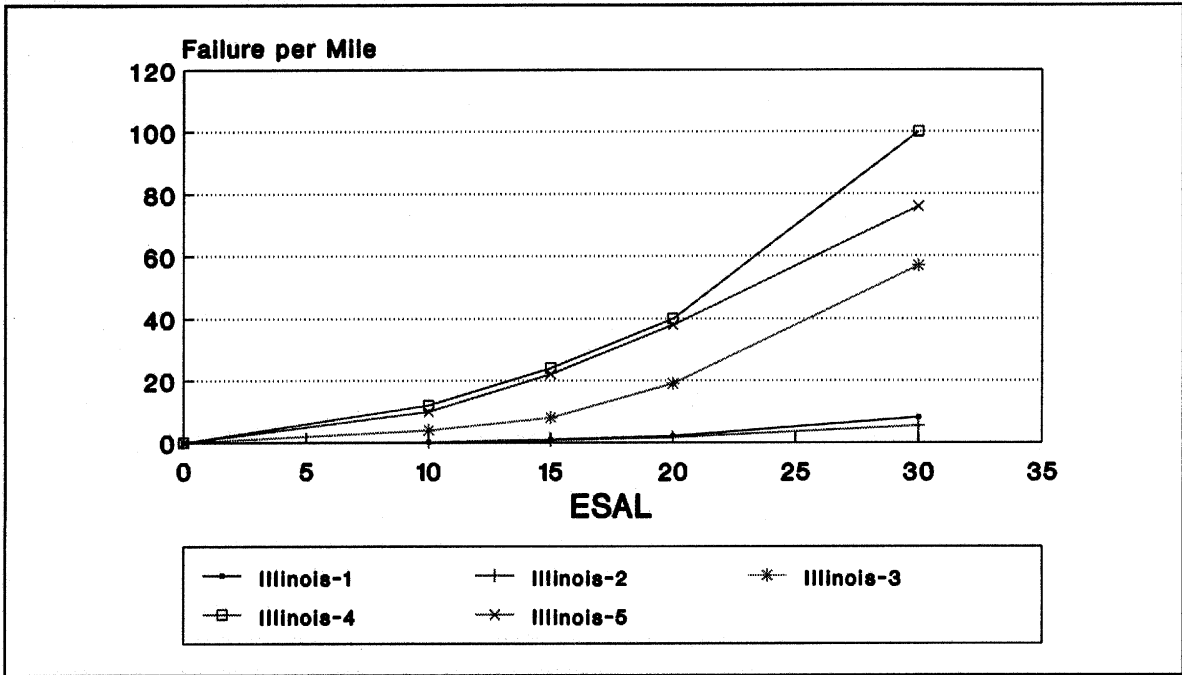
Figure 69. Performance prediction for sample sections in Illinois.
