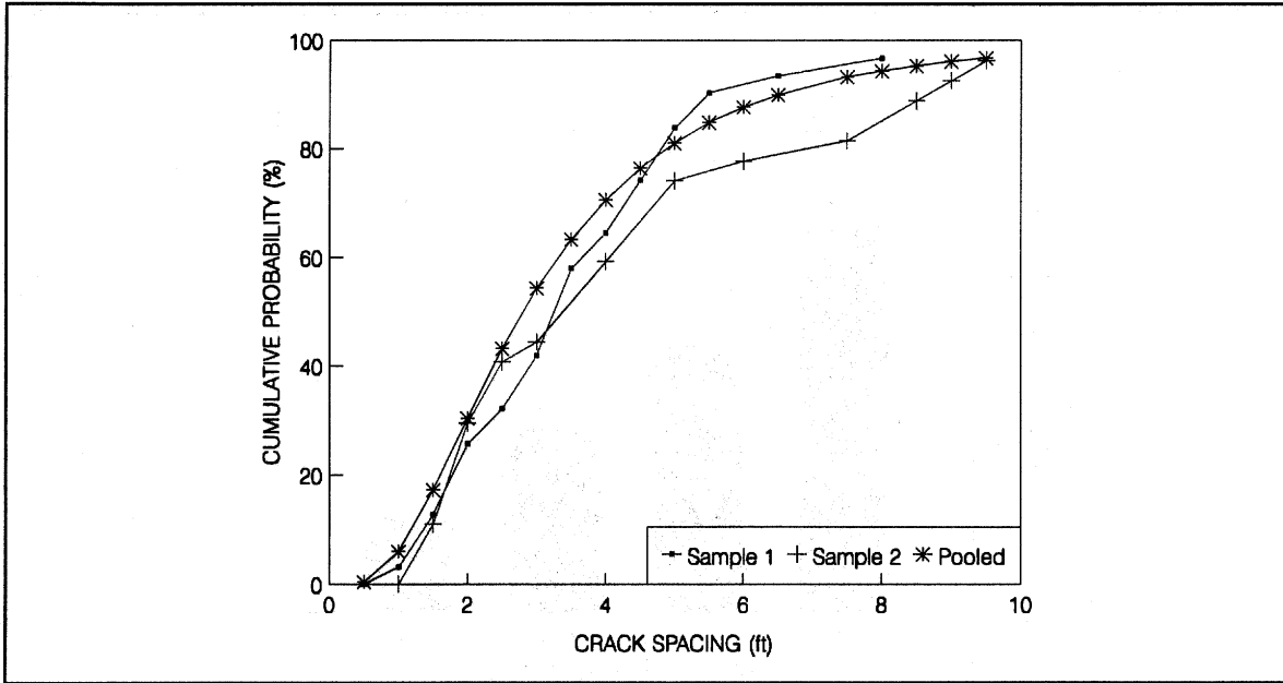
Figure 61. Field crack spacing distribution data: sample section Illinois-5.
