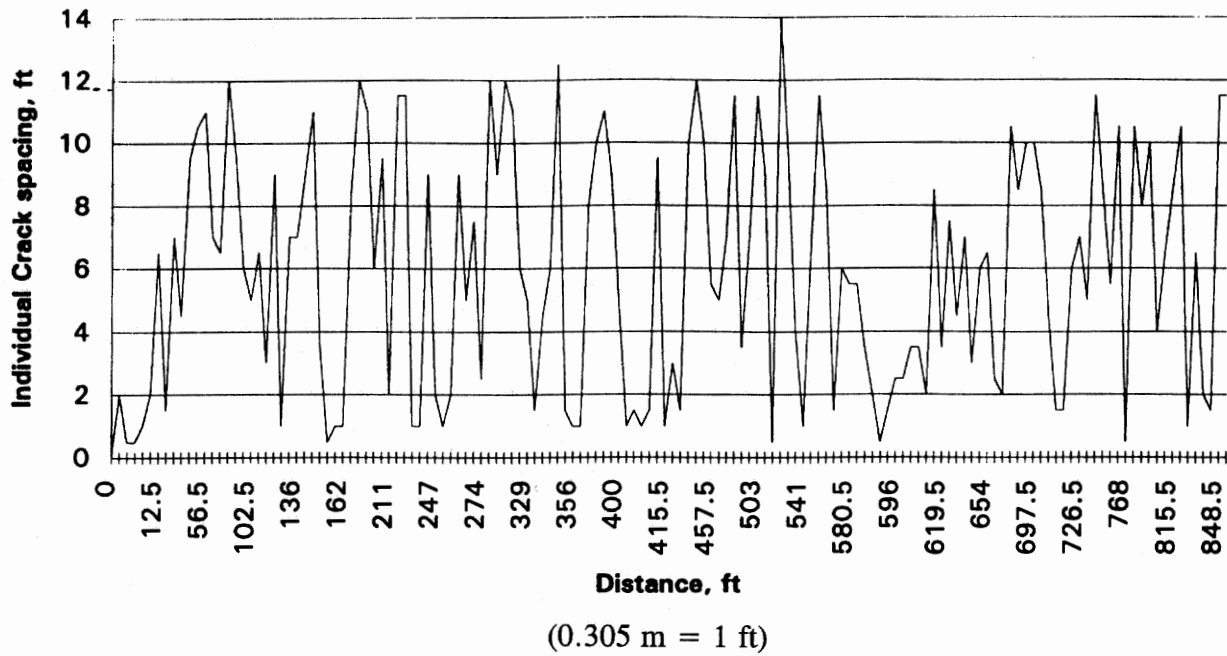
Figure 10. Crack spacing pattern for IA-1 - individual crack spacings.
