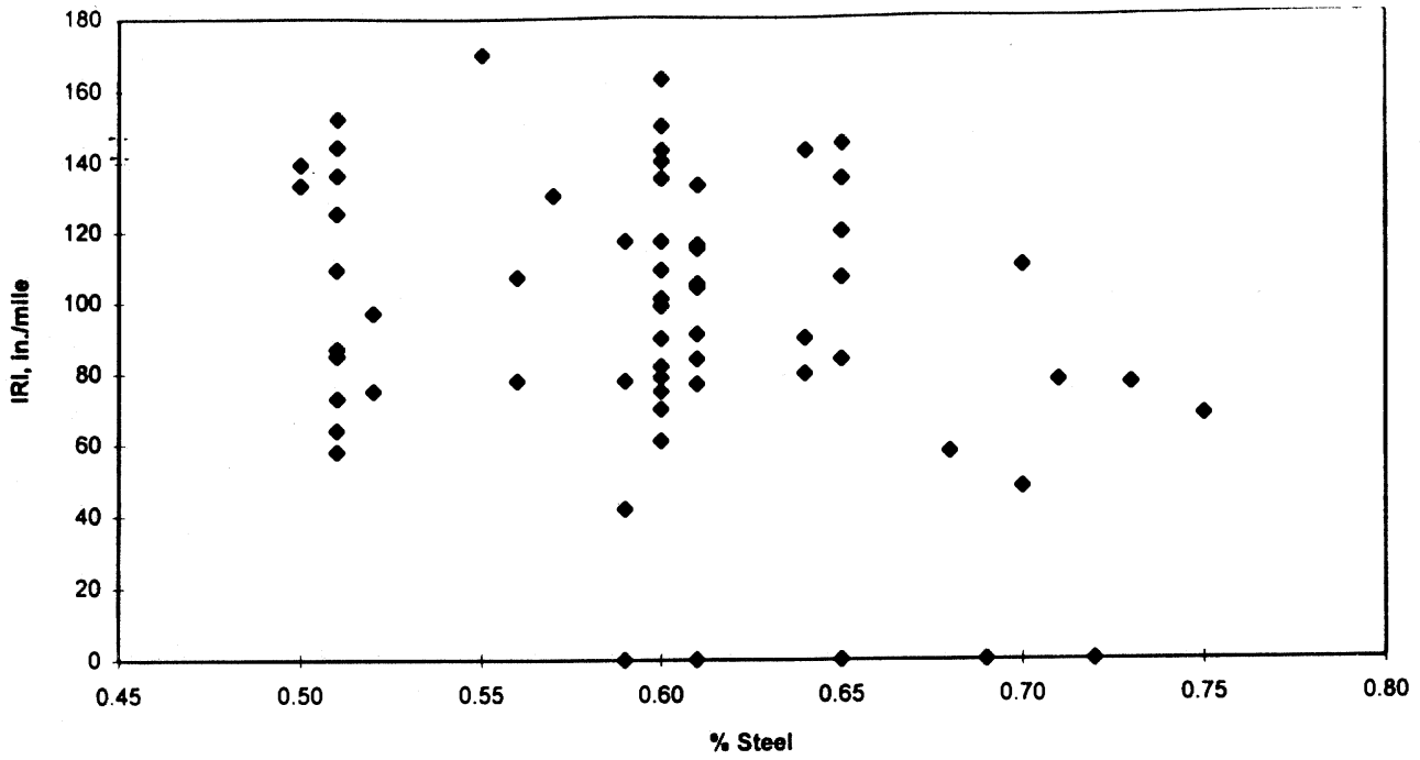
Figure 43. IRI versus percent steel.
