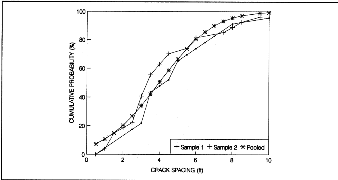
Figure 49. Field crack spacing distribution: sample section Illinois-2.
