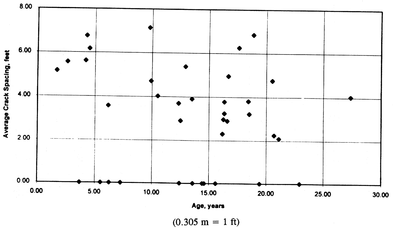
Figure 38. Crack spacing versus age - no-freeze sections.
