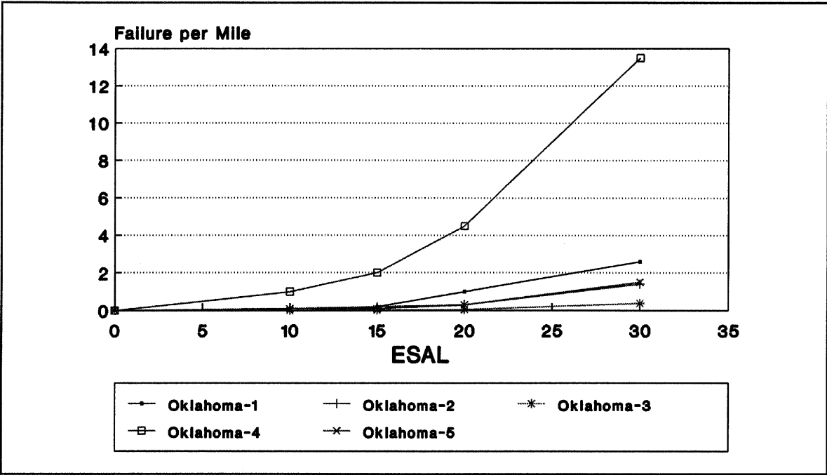
Figure 107. Performance prediction for sample sections in Oklahoma.
