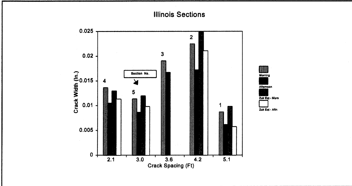
Figure 65. Variation in crack width with crack spacing for Illinois sample sections.
