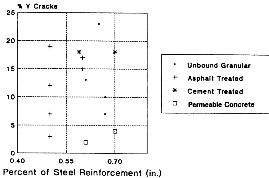
Figure 151. Y cracking versus percent of steel for different subbase types.
