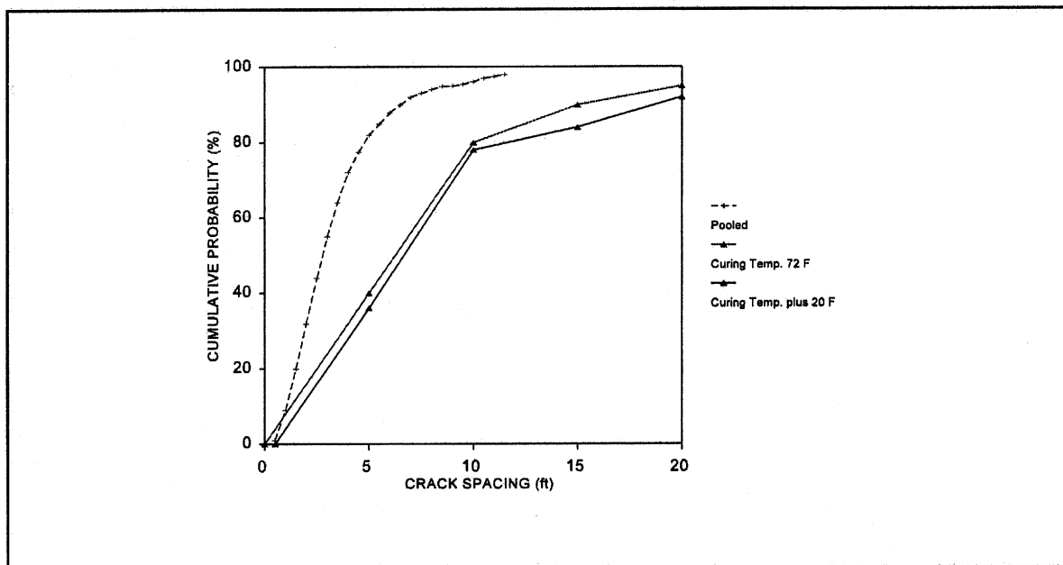
Figure 54. CRCP-5 crack distribution analysis for two curing temperatures from sample section Illinois-3.
