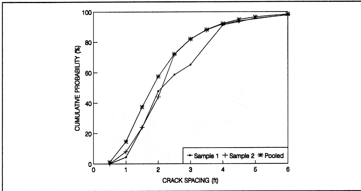
Figure 53. Field crack spacing distribution data: sample section Illinois-3.
