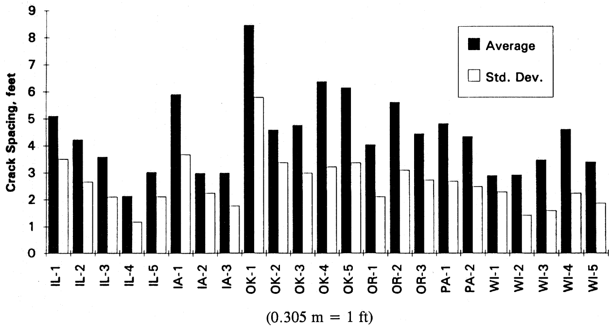
Figure 7. Crack spacing summary.
