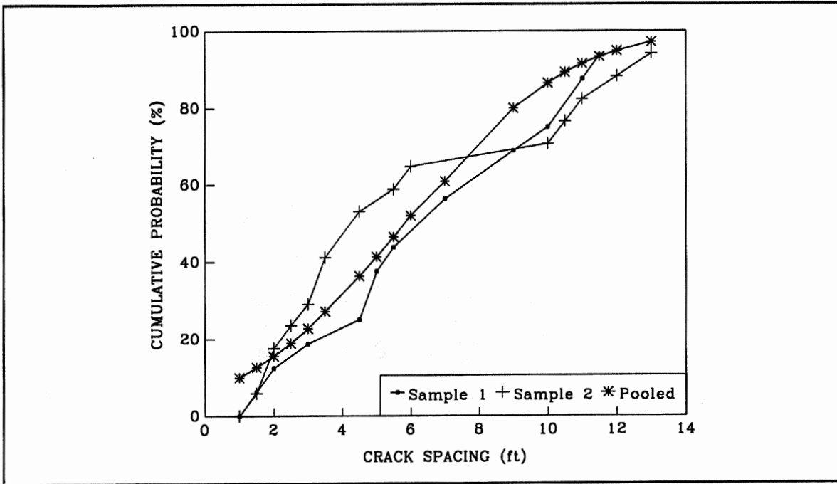
Figure 99. Field cracking spacing distribution data: sample section Oklahoma-5.
