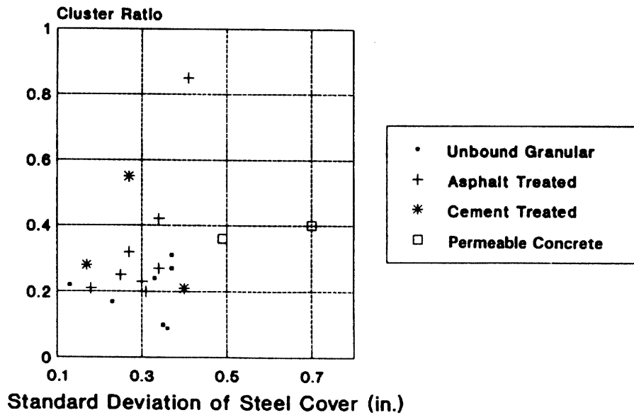
Figure 145. Cluster ratio versus the standard deviation of steel cover for different subbase types.
