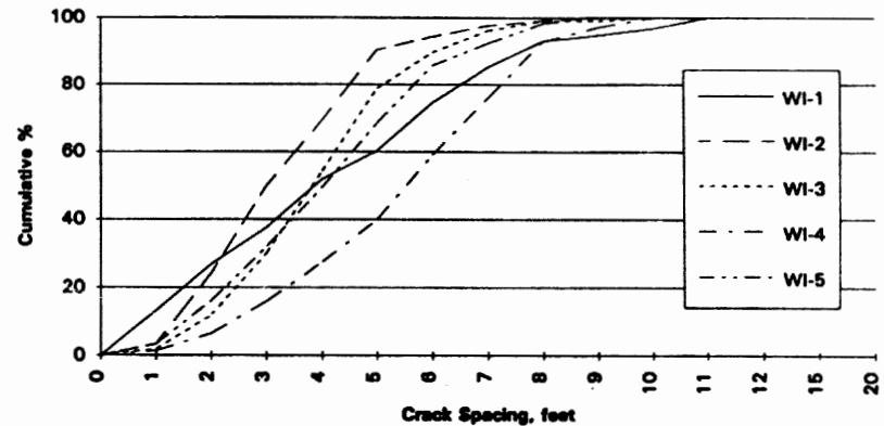
Figure 9. Crack spacing distribution (by length of paving)
