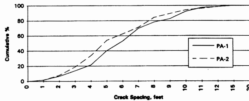
Figure 9. Crack spacing distribution (by length of paving)
