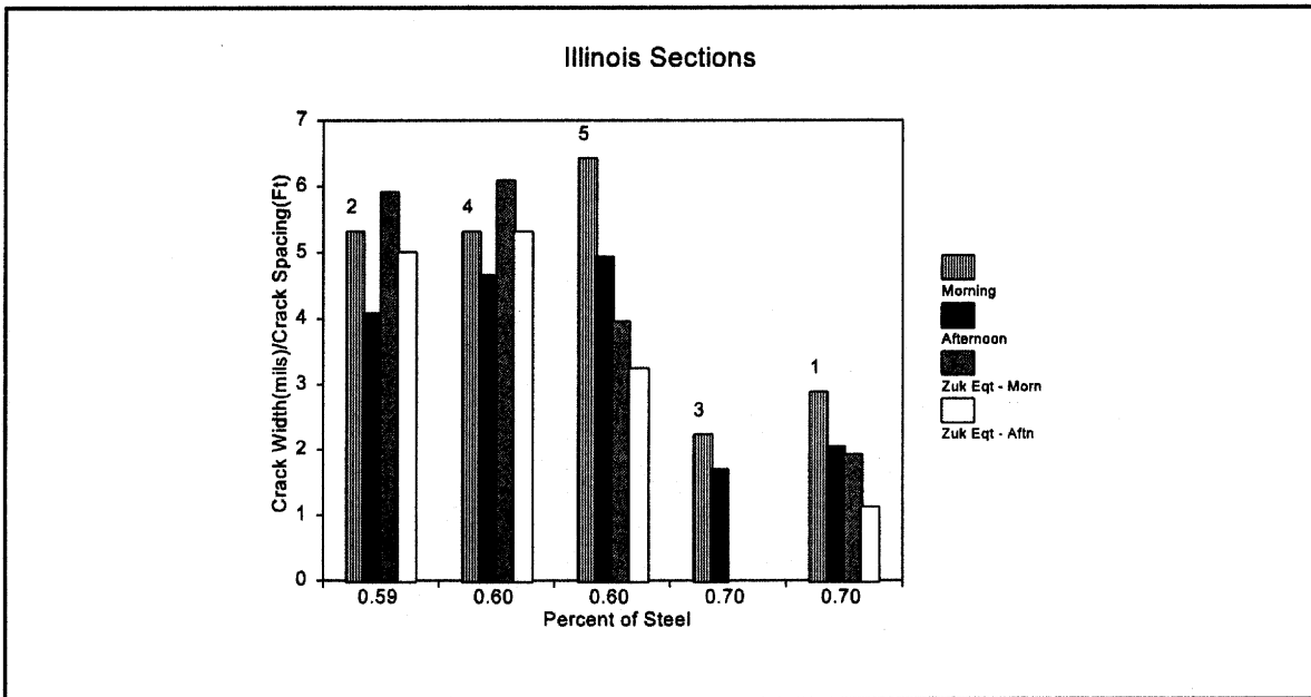
Figure 66. Variation in crack width/crack spacing ratio with percent reinforcement for Illinois sample sections.
