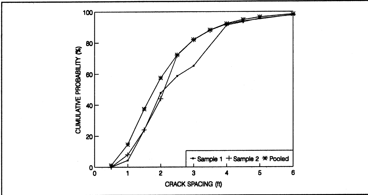
Figure 57. Field crack spacing distribution: sample section Illinois-4.
