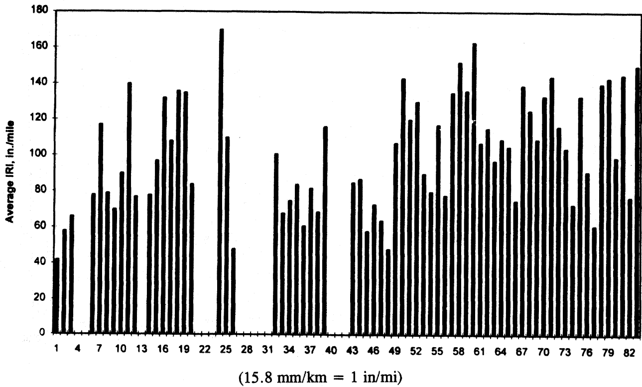
Figure 36. Average IRI summary.
