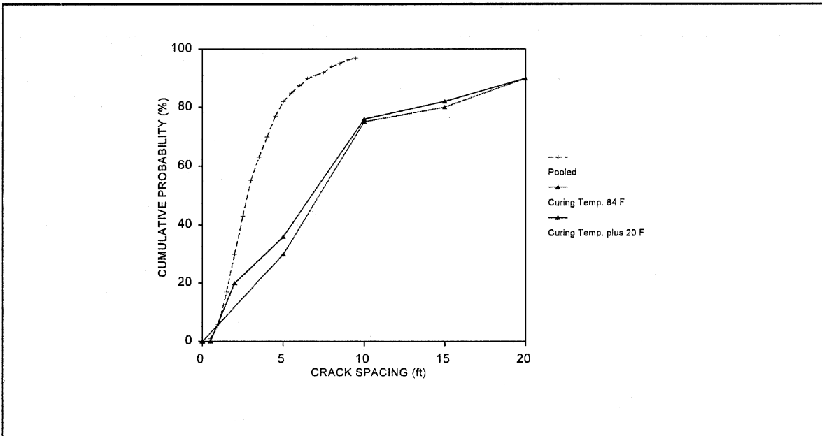
Figure 62. CRCP-5 crack distribution analysis for two curing temperatures from sample section Illinois-5.
