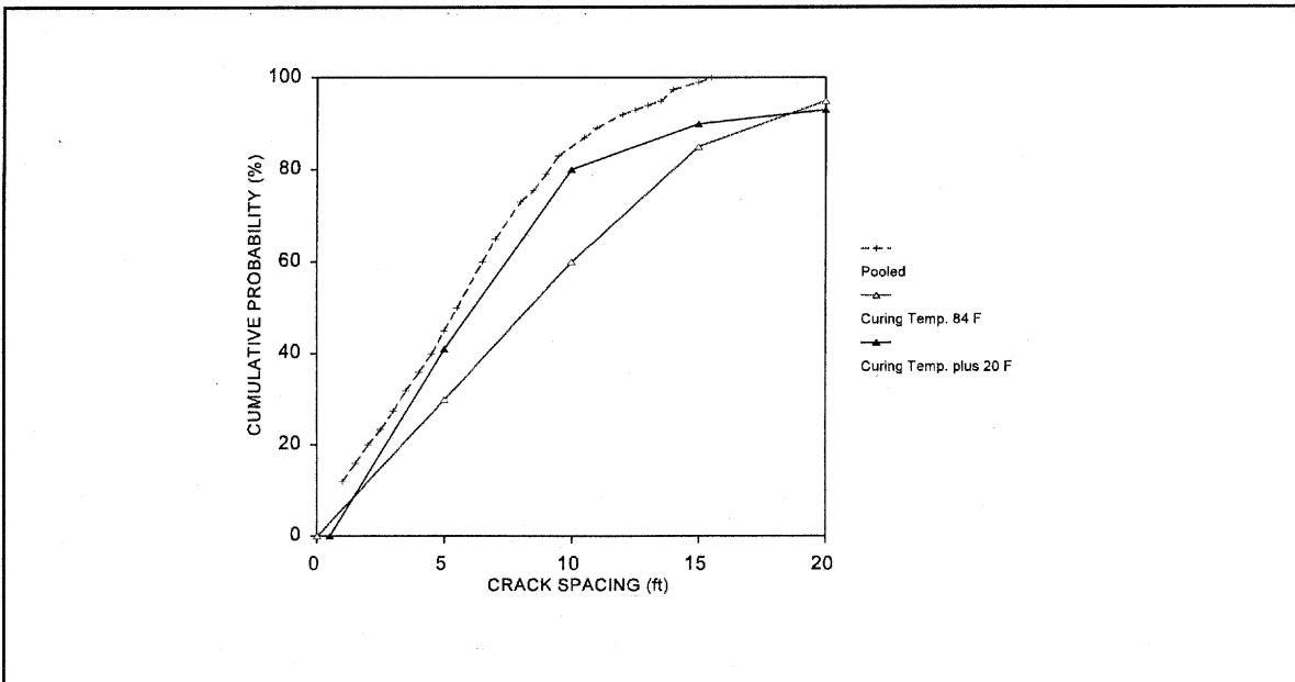
Figure 46. CRCP-5 crack distribution analysis for two curing temperatures from section Illinois-1.
