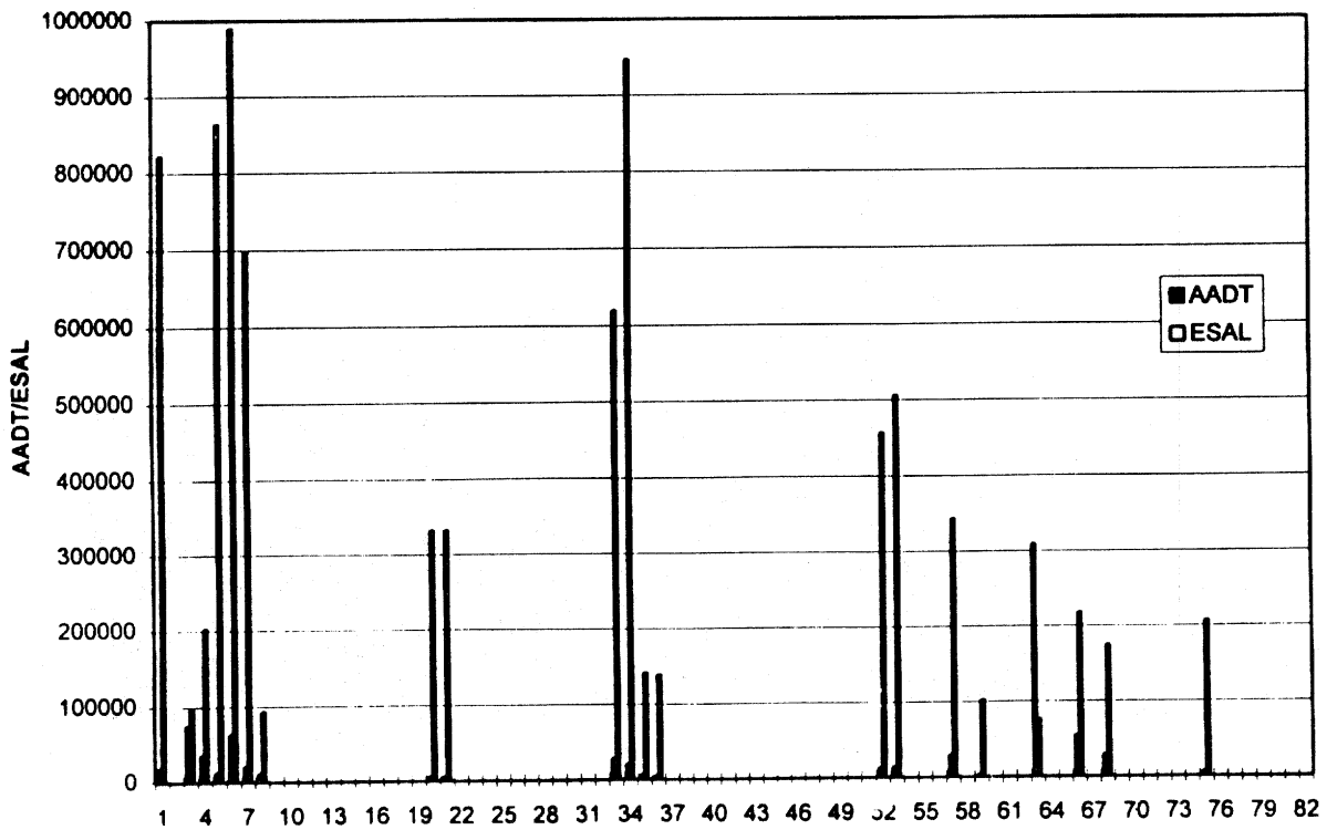
Figure 34. 1989 AADT (2-way) and ESAL.
