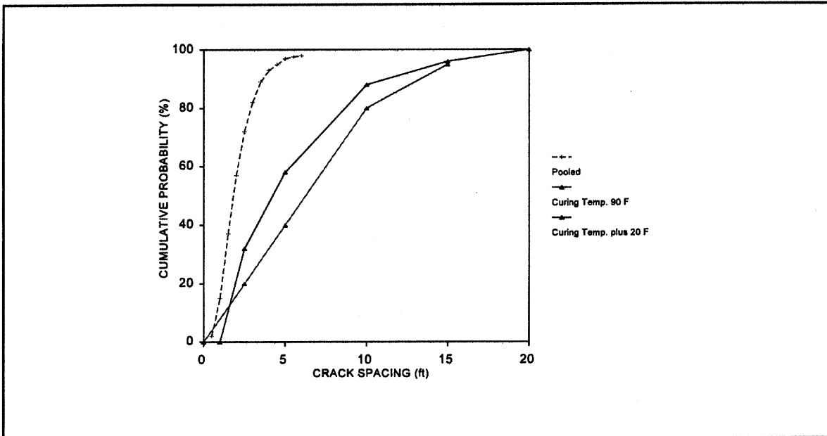
Figure 58. CRCP-5 crack distribution analysis for two curing temperatures from sample section Illinois-4.
