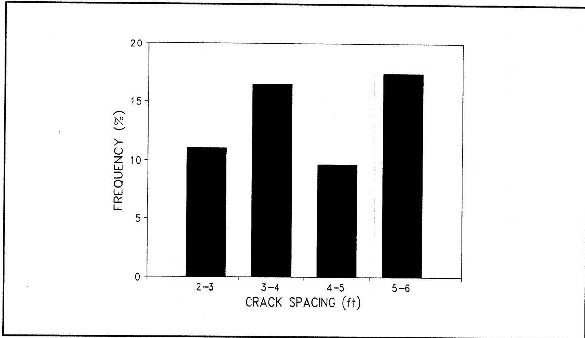
Figure 131. Crack spacing frequency: sample section Wisconsin-4.
