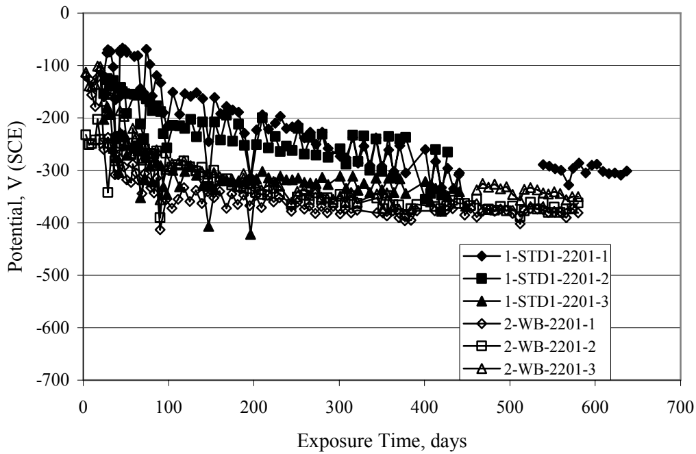
Figure 4.92. Graph. Plot of potential versus exposure time for STD1 concrete specimens with wire brushed (WB) 2201 bars compared to ones with as-received 2201 bars.
