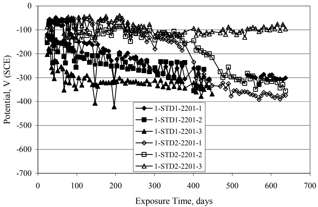
Figure 4.90. Graph. Plot of potential versus exposure time for STD1 and STD2 concrete specimens with 2201 reinforcement.
