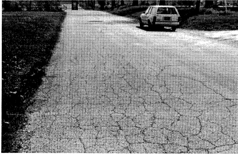
Figure 2-7. Example of typical alligator cracking pattern. (1)
