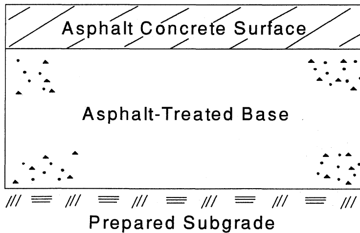
Figure 3-1. Typical full-depth asphalt pavement cross-section.
