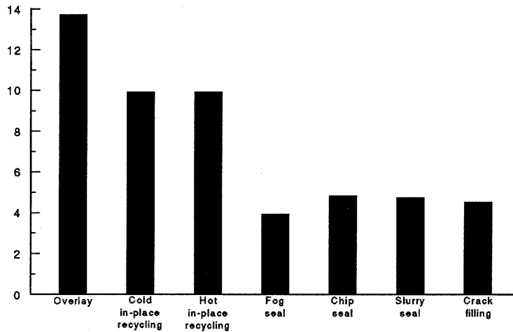
Figure 7-5. Expected life of various rehab methods. (5)
