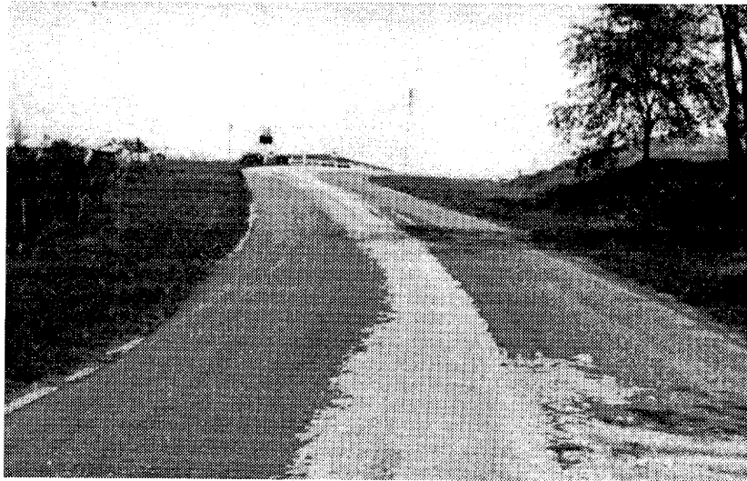
Figure 2-8. Example of edge wedging. (1)
