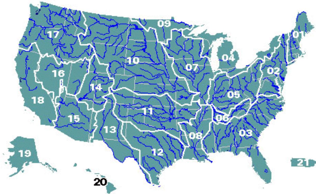
Figure E2-1. U.S. Hydrologic Regions
