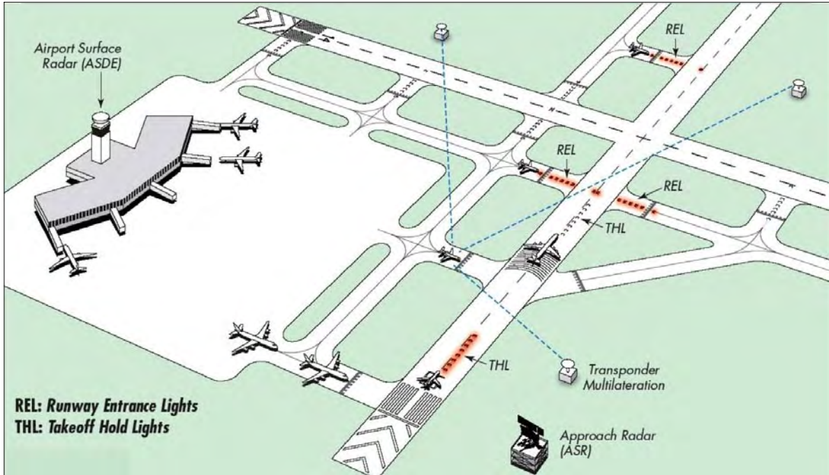
FIG AD 1.1-52 Runway Status Light System
