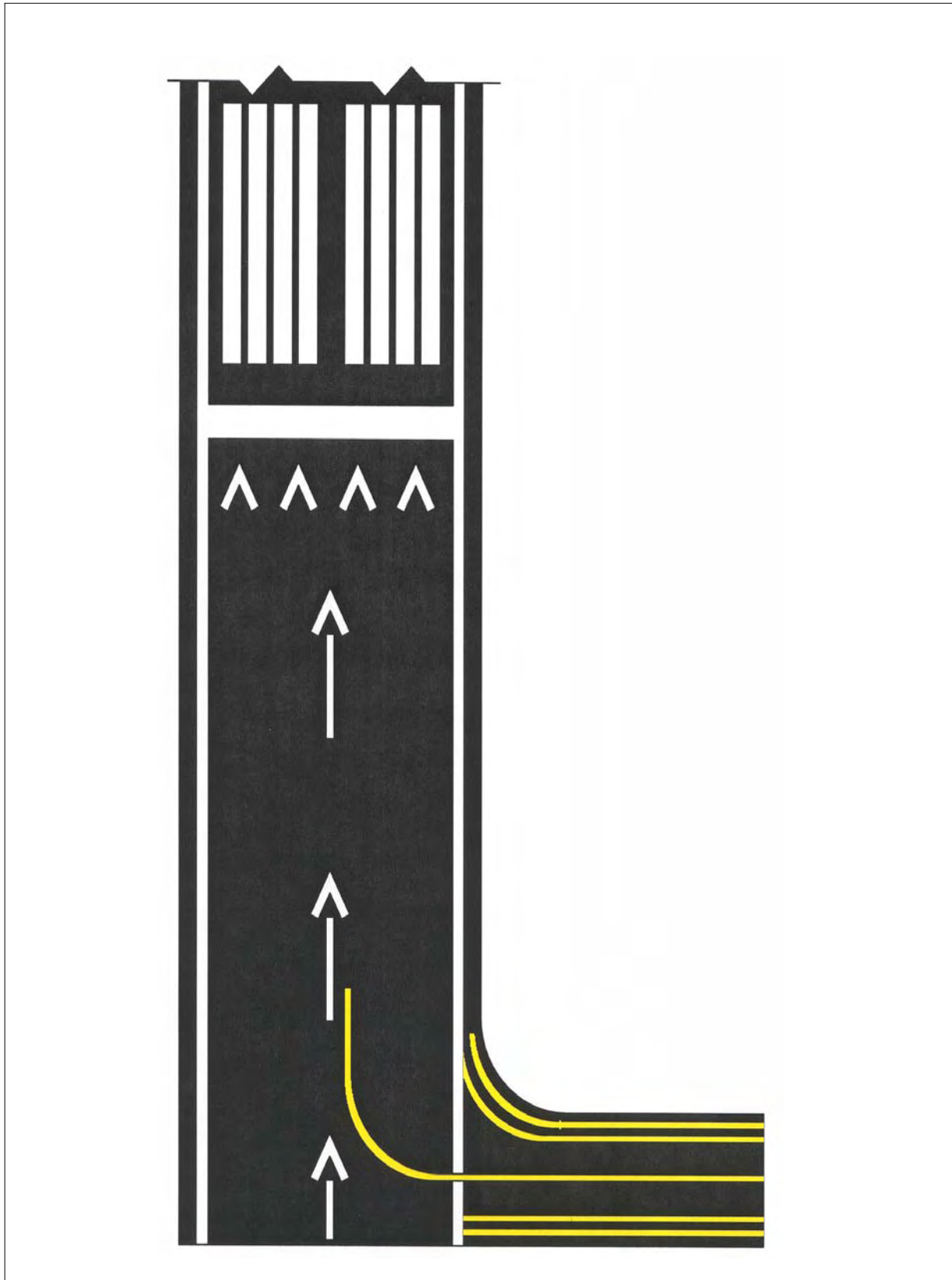
FIG AD 1.1-14 Displaced Threshold Markings
