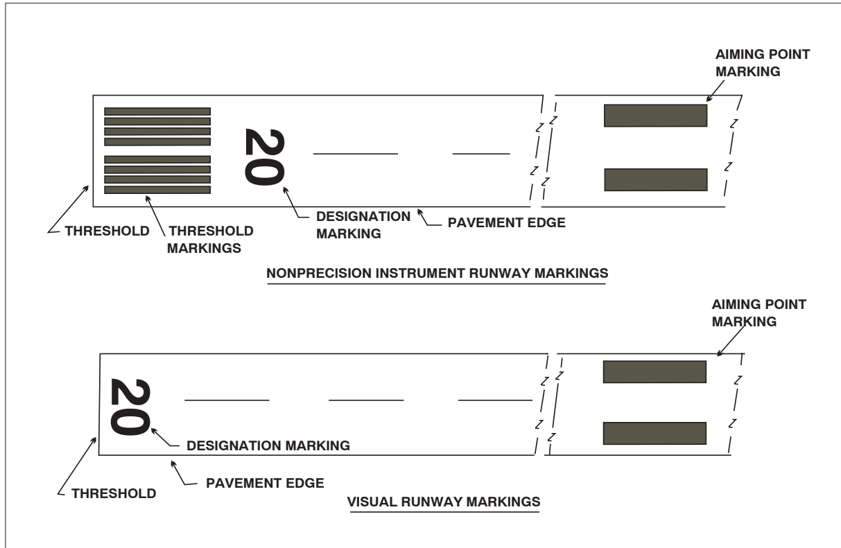
FIG AD 1.1-11 Nonprecision Instrument Runway and Visual Runway Markings
