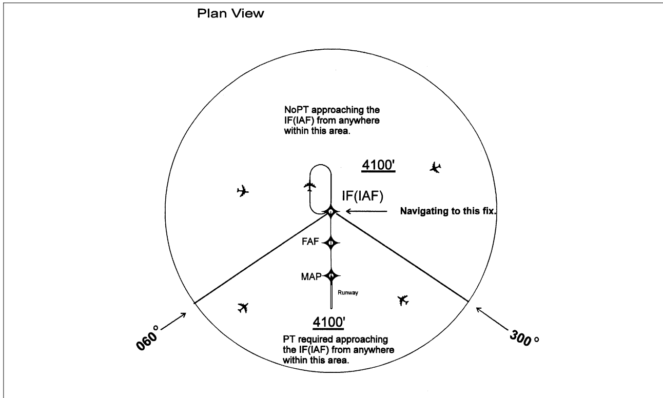
FIG ENR 1.5-21 TAA with Left and Right Base Areas Eliminated
