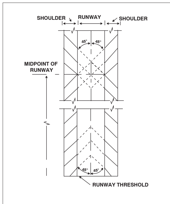
FIG AD 1.1-12 Runway Shoulder Markings
