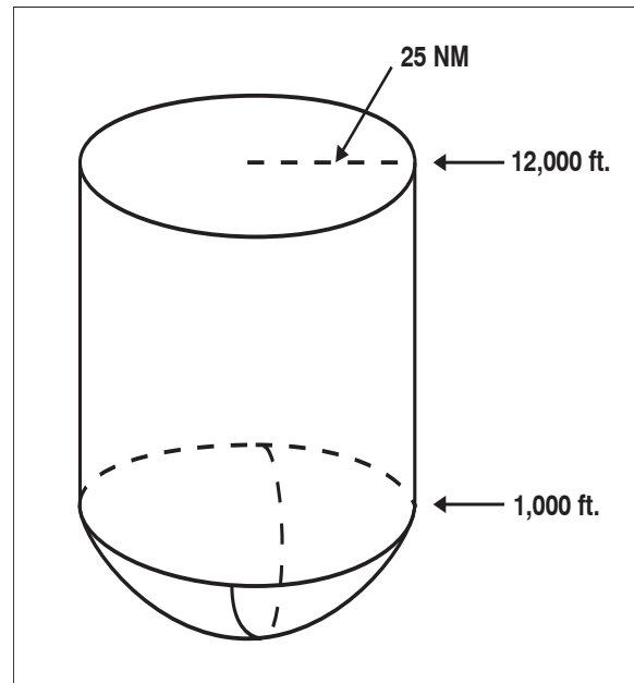
FIG GEN 3.4-3 Standard Terminal Service Volume (See FIG GEN 3.4-4 for altitudes below 1,000 feet.)
