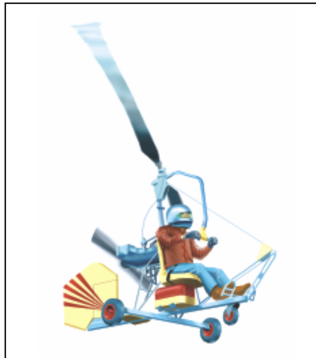
Figure 17-2. The direct overhead stick attachment has been used for control of the rotor disc on some gyroplanes.
