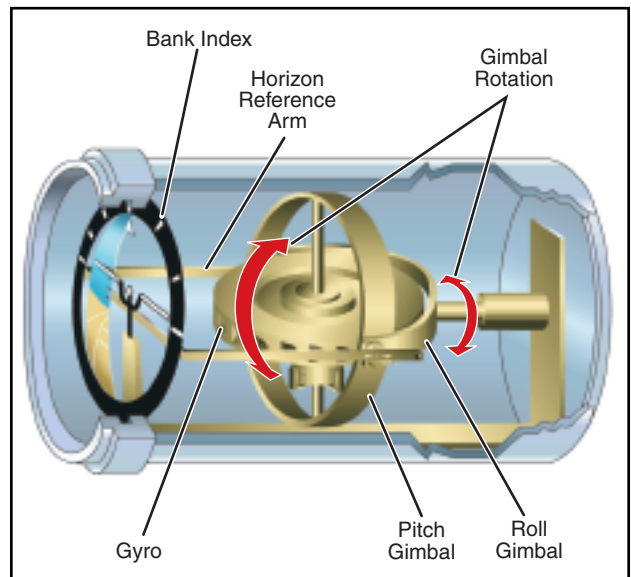
Figure 12-5. The gyro in the attitude indicator spins in the horizontal plane. Two mountings, or gimbals, are used so that both pitch and roll can be sensed simultaneously. Due to rigidity in space, the gyro remains in a fixed position relative to the horizon as the case and helicopter rotate around it.
