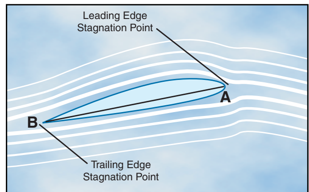
Figure 2-8. Air circulation around an airfoil occurs when the front stagnation point is below the leading edge and the aft stagnation point is beyond the trailing edge.
