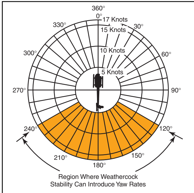
Figure 11-11. Weathercock stability.
