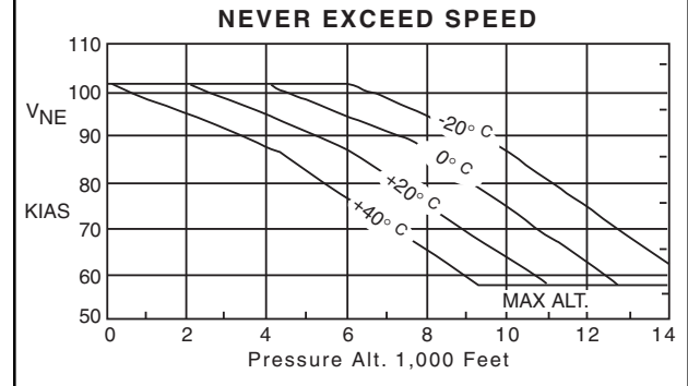
Figure 6-6. Various V_{NE} placards.
