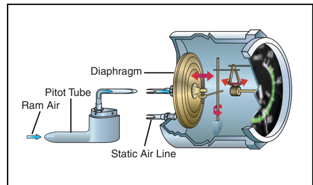
Figure 12-2. Ram air pressure from the pitot tube is directed to a diaphragm inside the airspeed indicator. The airtight case is vented to the static port. As the diaphragm expands or contracts, a mechanical linkage moves the needle on the face of the indicator.
