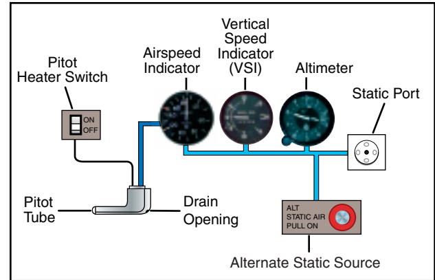
Figure 12-1. Ram air pressure is supplied only to the airspeed indicator, while static pressure is used by all three instruments. Electrical heating elements may be installed to prevent ice from forming on the pitot tube. A drain opening to remove moisture is normally included.
