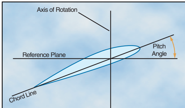
Figure 2-4. Do not confuse the axis of rotation with the rotor mast. The only time they coincide is when the tip-path plane is perpendicular to the rotor mast.
