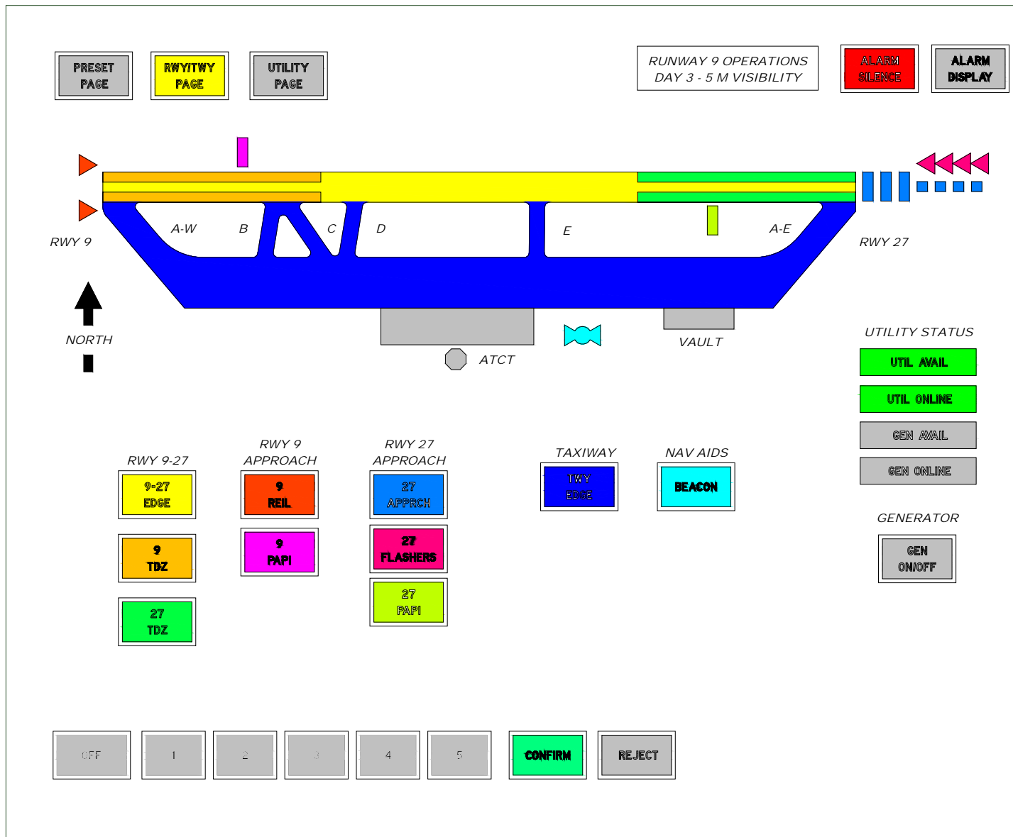
Figure 9. ALCMS Test System Touchscreen GUI: RWY/TWY Page
