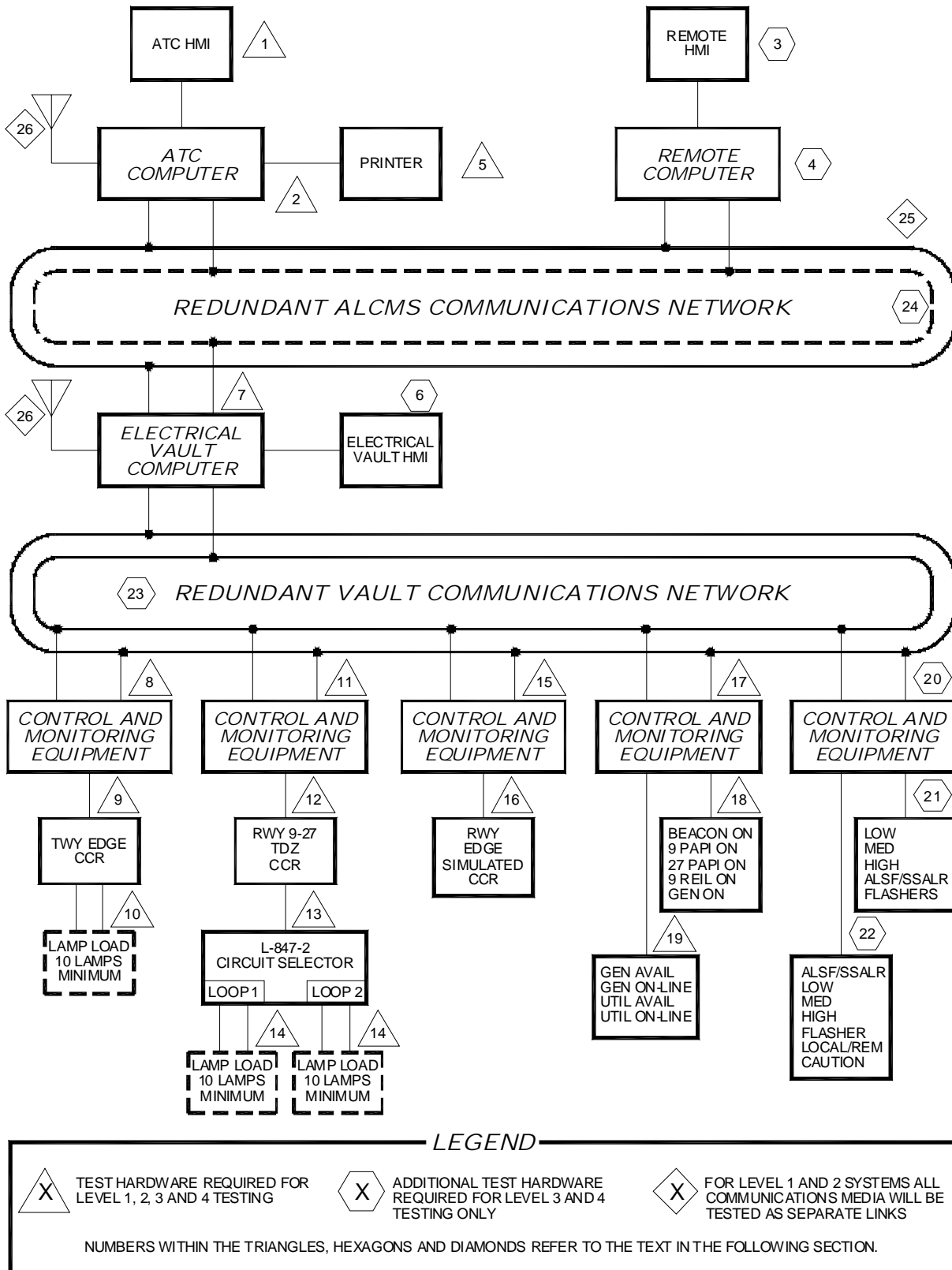
Figure 7. ALCMS Test System Hardware Design
