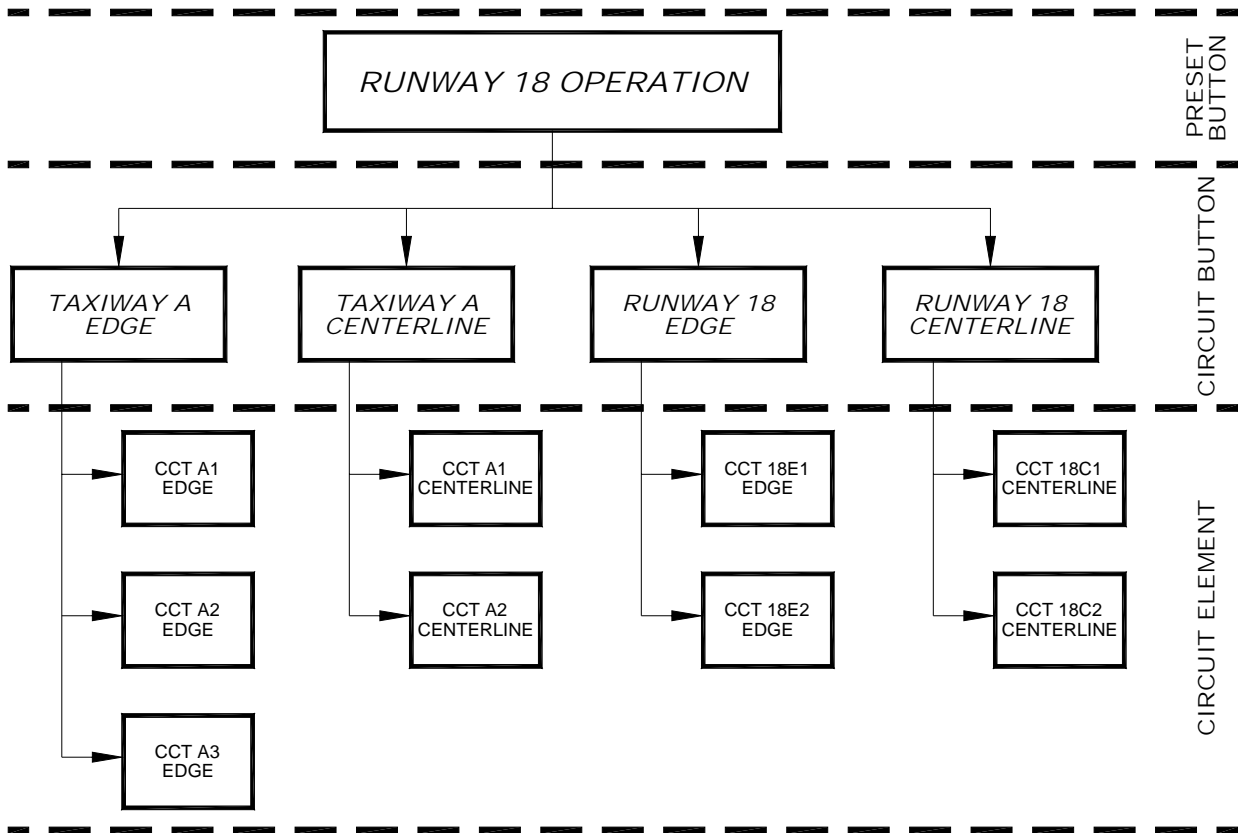
Figure 3. Control Methodology Overview
