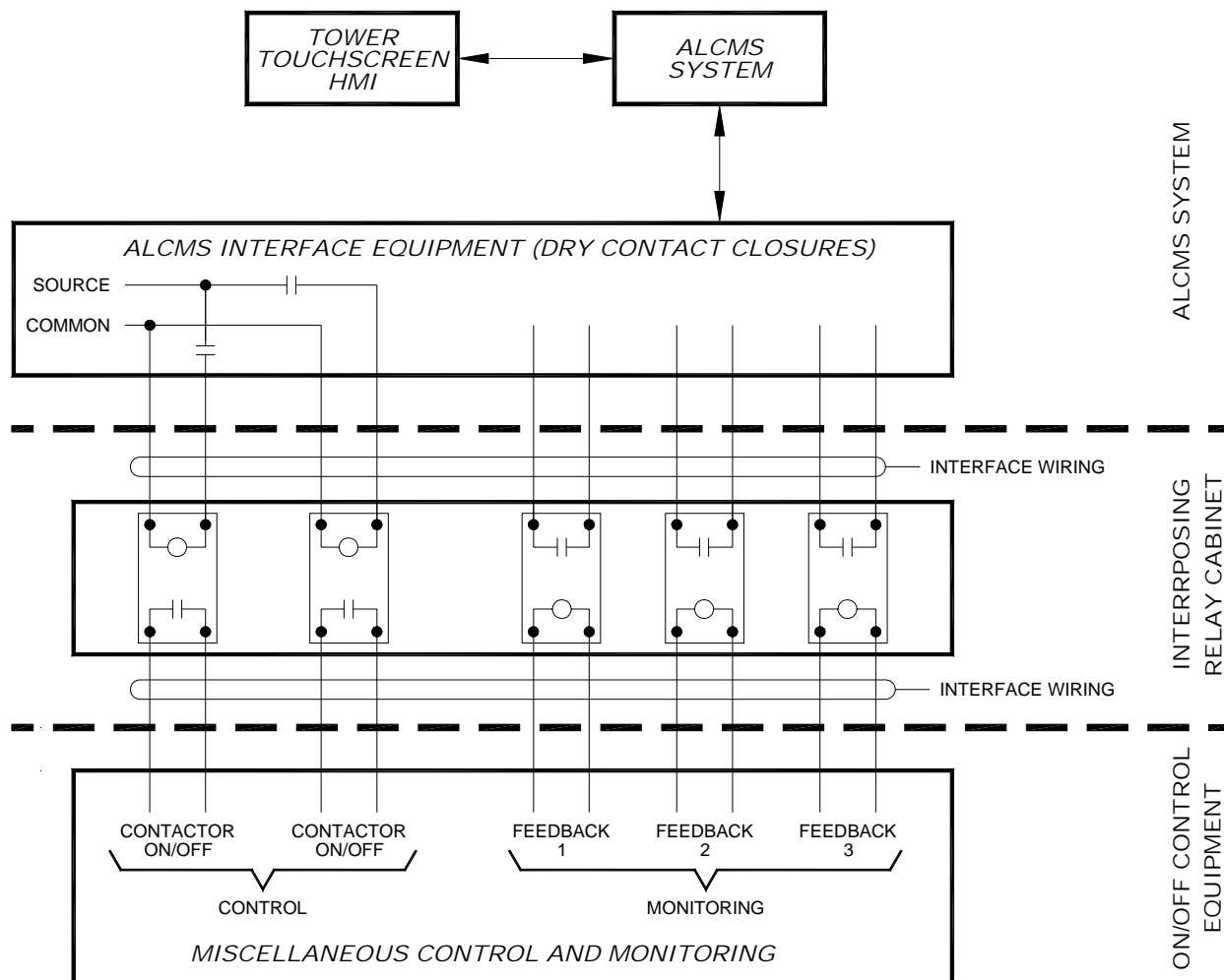
Figure 6. Contactor Interface Diagram
