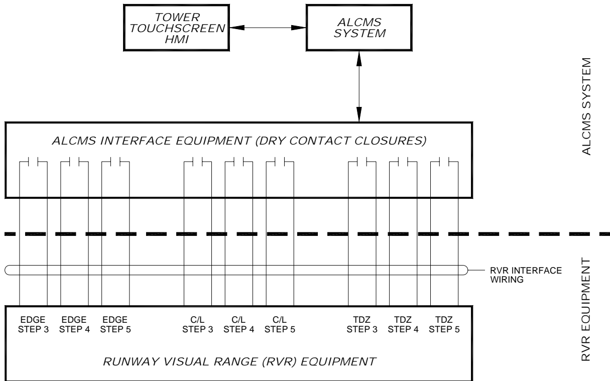
Figure 4. RVR Interface Diagram
