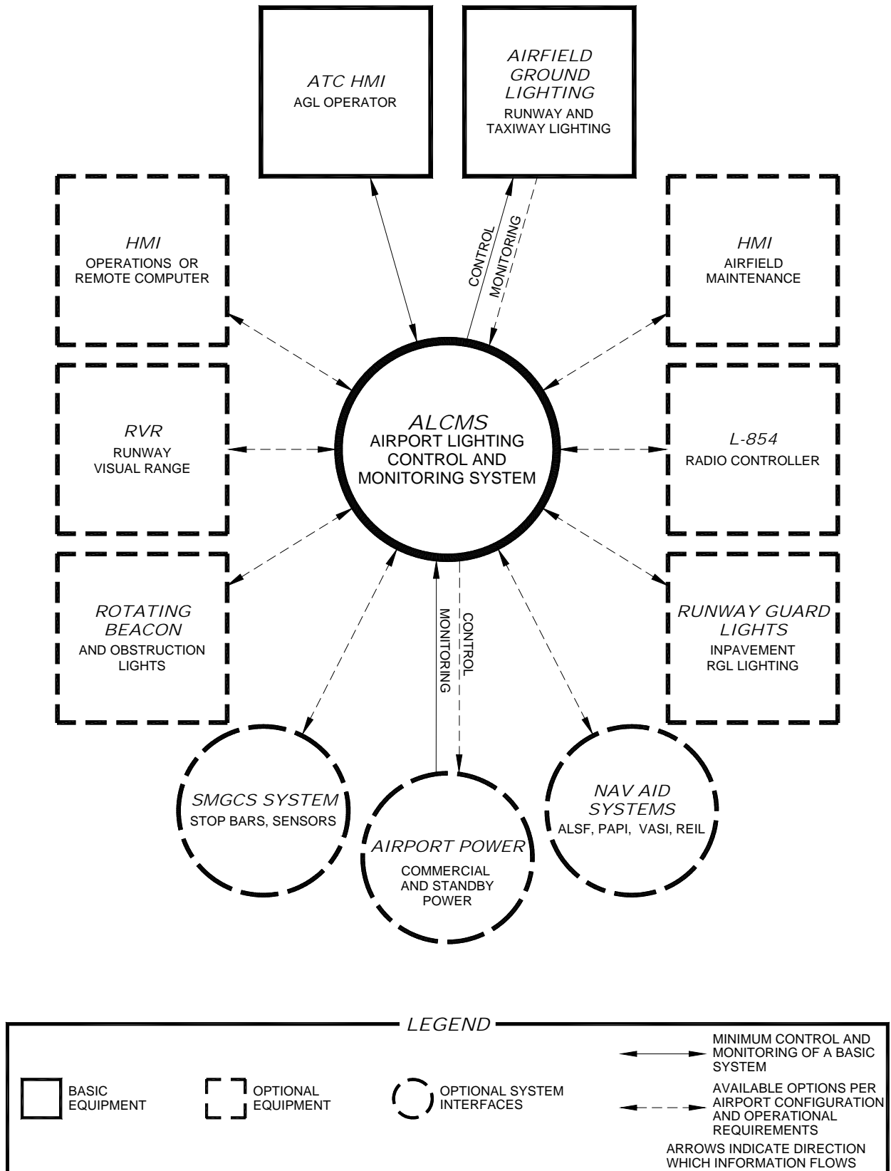
Figure 1. ALCMS Interface Overview
