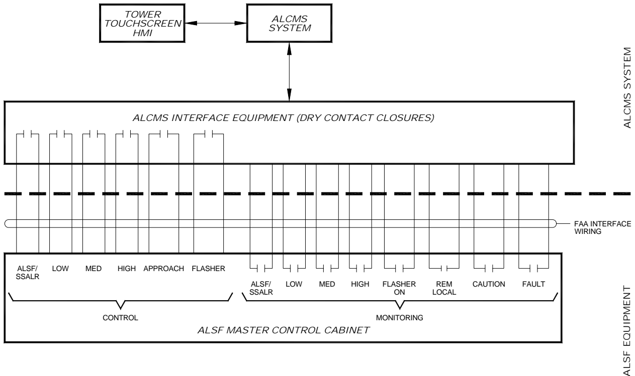
Figure 5. ALSF Interface Diagram
