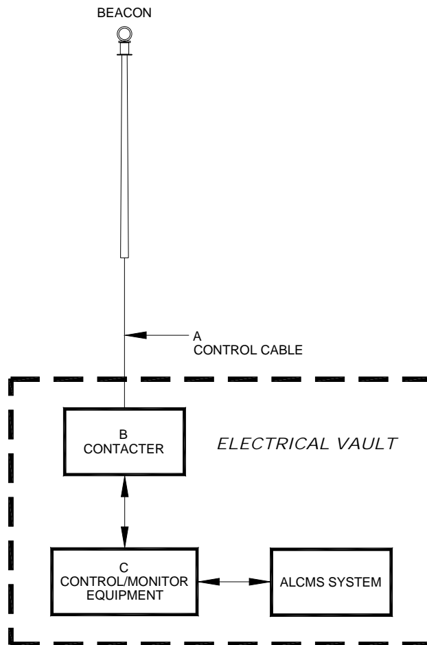
Figure 14. Beacon Installation Example
