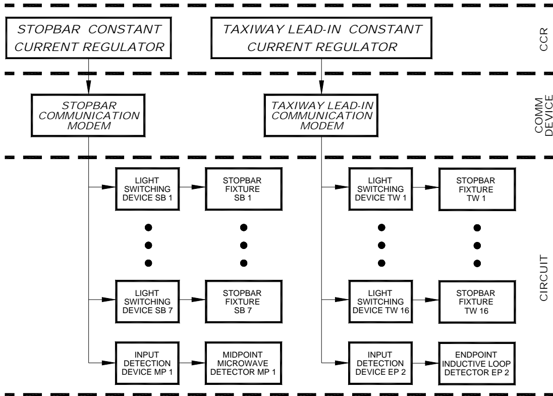
Figure 11. SMGCS Test System
