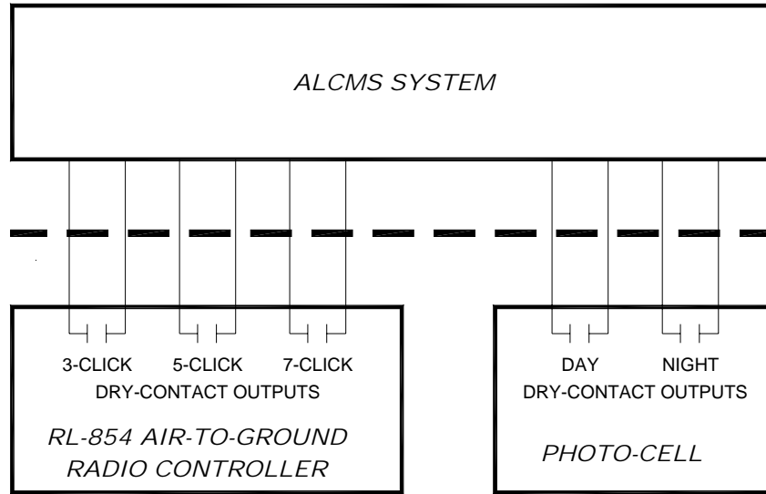
Figure 13. Radio Control and Photocell Interface Examples
