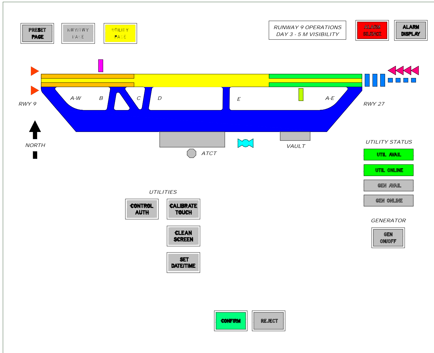
Figure 10. ALCMS Test System Touchscreen GUI: Utility Page
