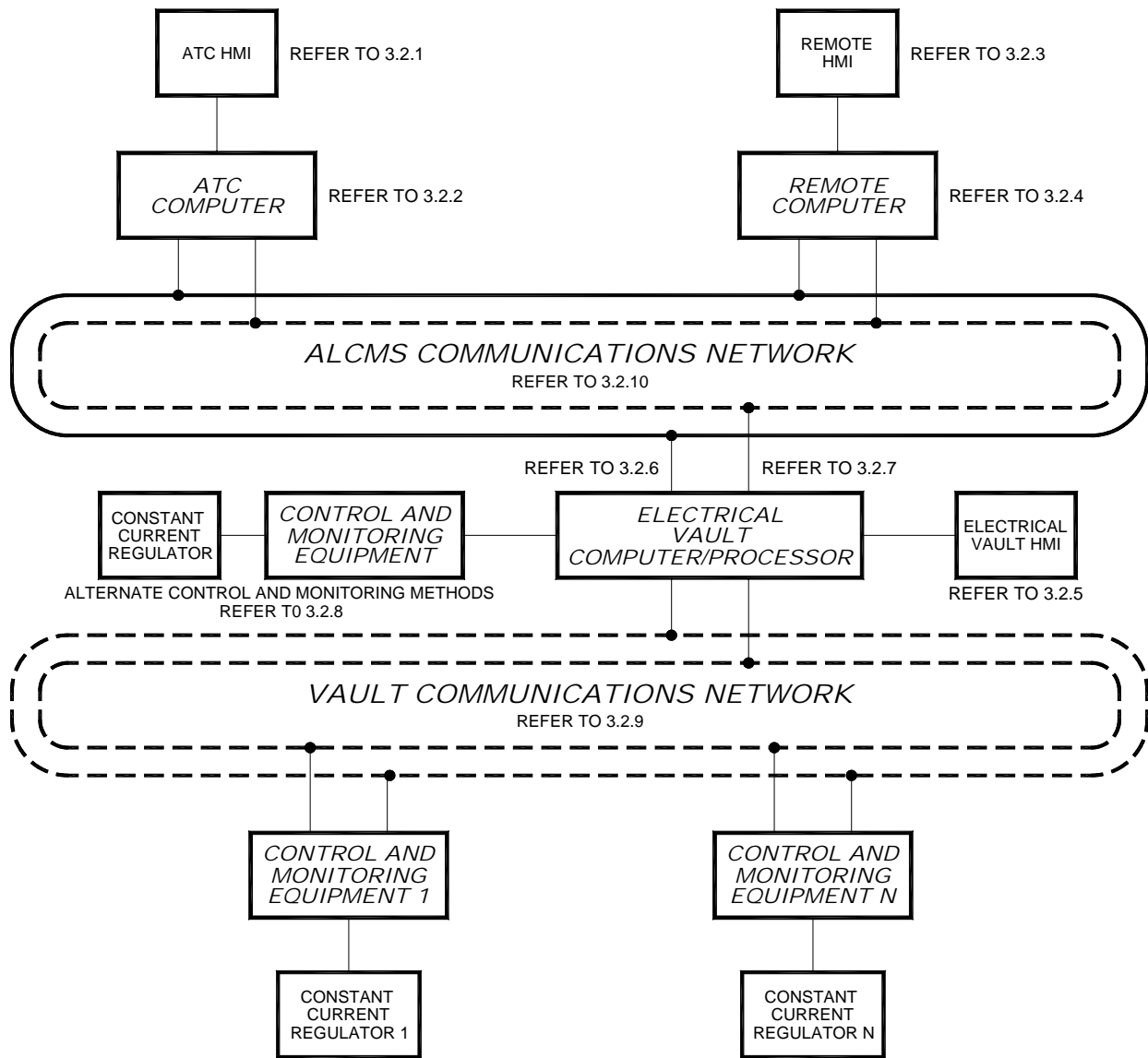
Figure 2. ALCMS Components Overview
