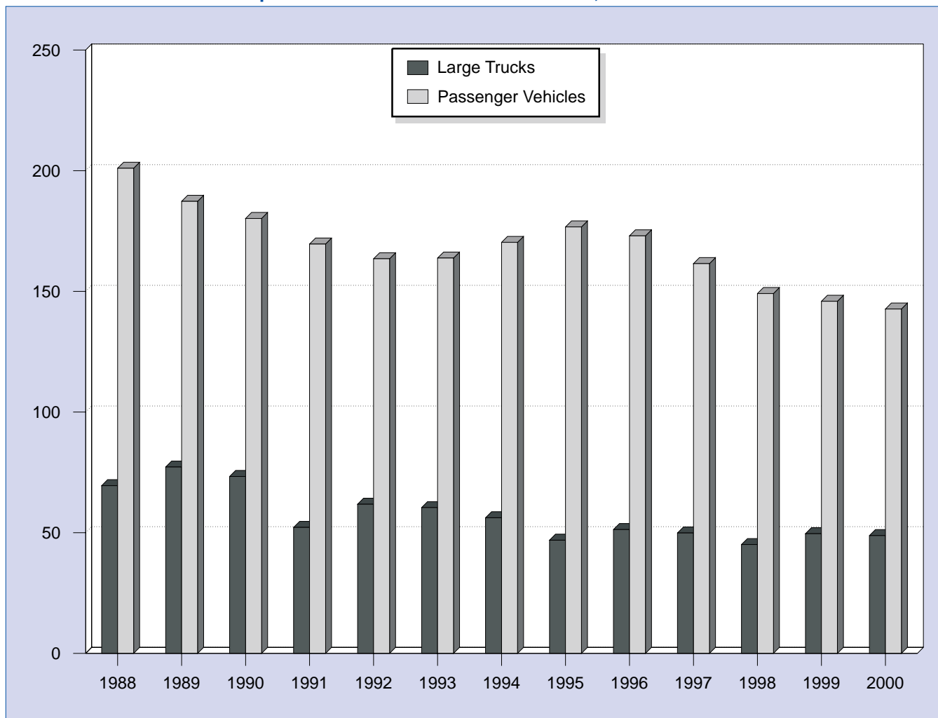
Figure 4. Large Trucks and Passenger Vehicles Involved in Injury Crashes per 100 Million Vehicle Miles Traveled, 1988-2000
