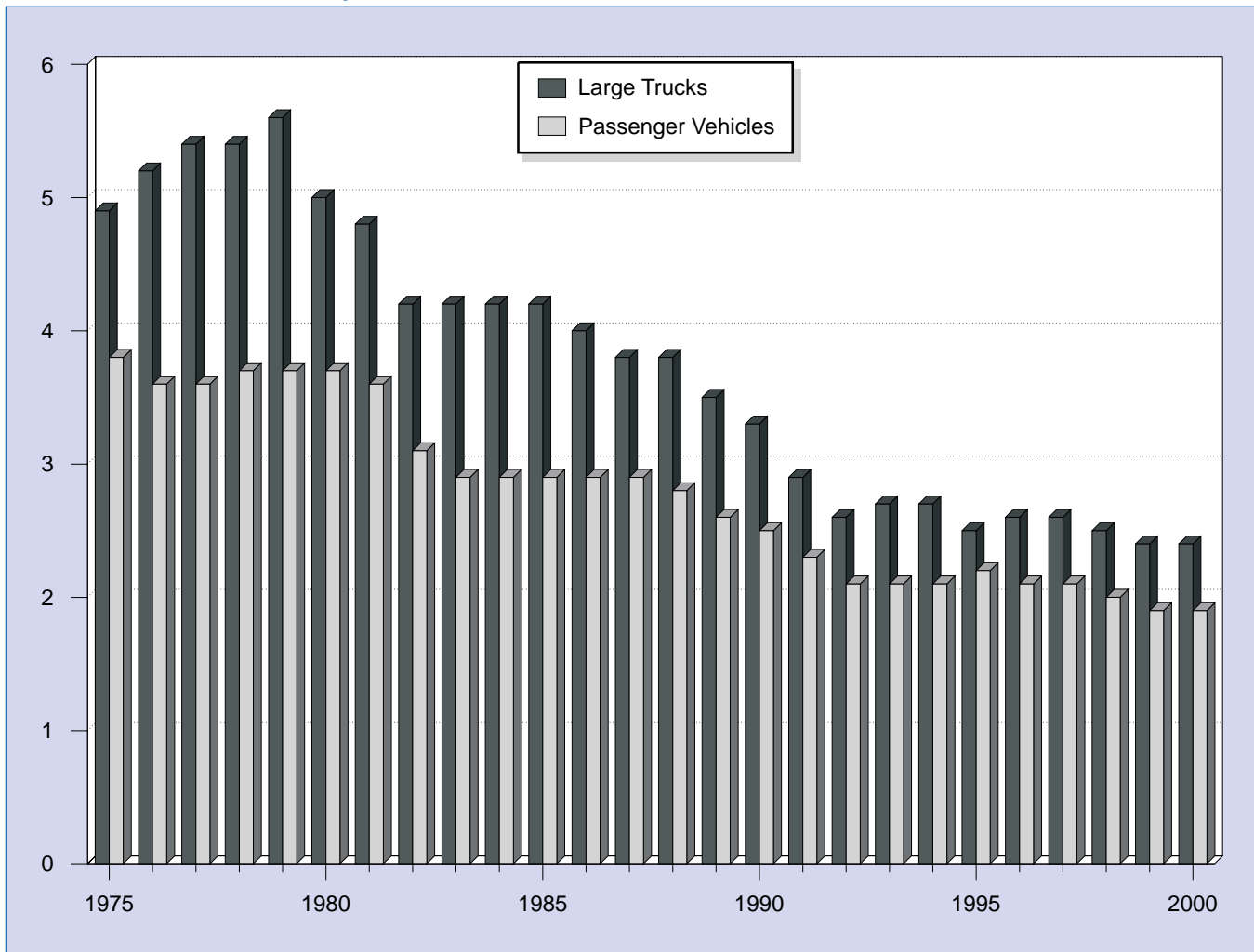
Figure 2. Large Trucks and Passenger Vehicles Involved in Fatal Crashes per 100 Million Vehicle Miles Traveled, 1975-2000
