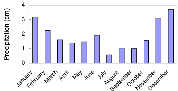
Average monthly precipitation: Wenatchee
