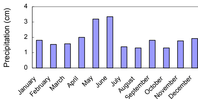
Average monthly precipitation: INEEL
