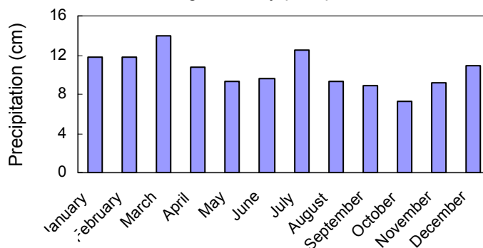
Average monthly precipitation: Atlanta
