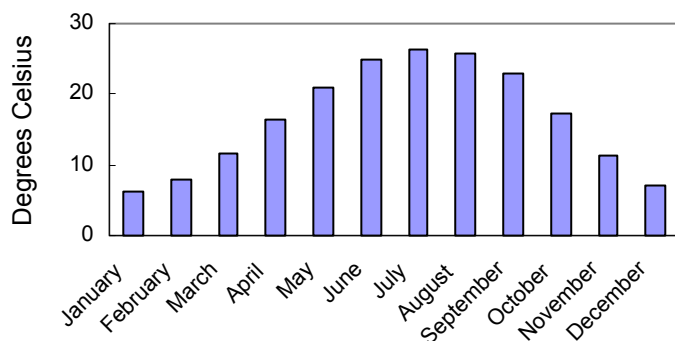
Average monthly temperature: Atlanta
