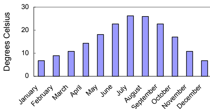
Average monthly temperature: Victorville
