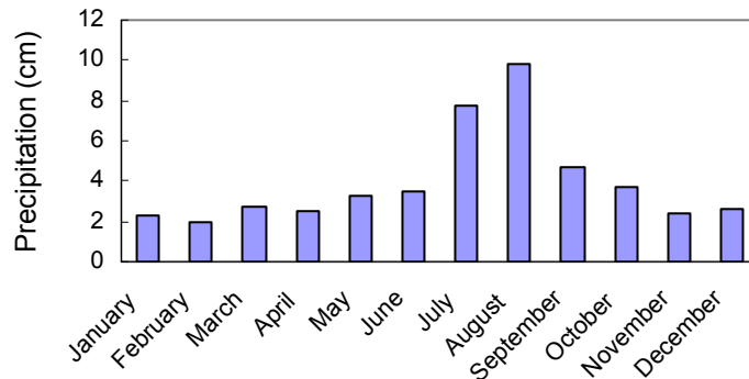
Average monthly precipitation: Los Alamos
