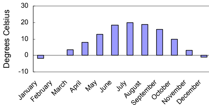
Average monthly temperature: Los Alamos
