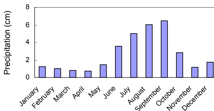
Average monthly precipitation: El Paso
