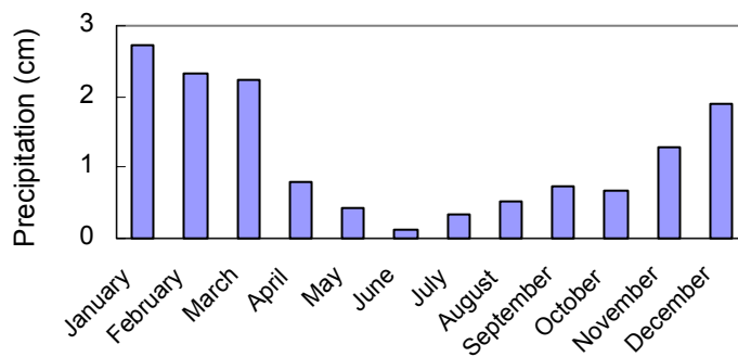
Average monthly precipitation: Victorville
