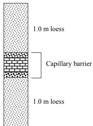
1.0 m biobarrier design
