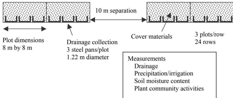
INEEL PC/BE Lysimeter Facility
