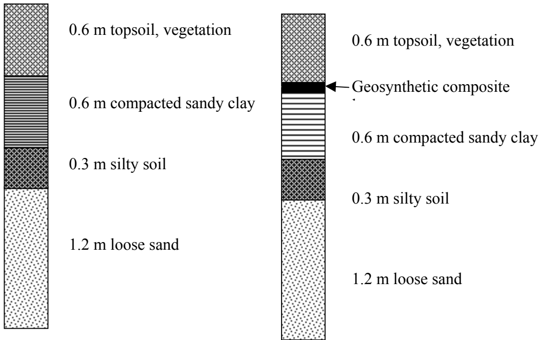
Cover design tested at the Savannah River Site Test Pad Facility
