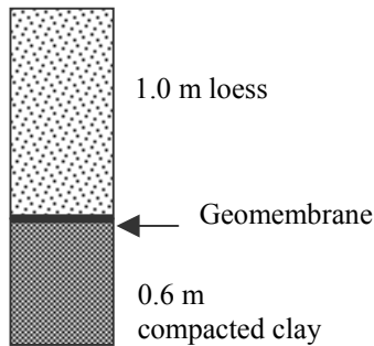
RCRA-type design
