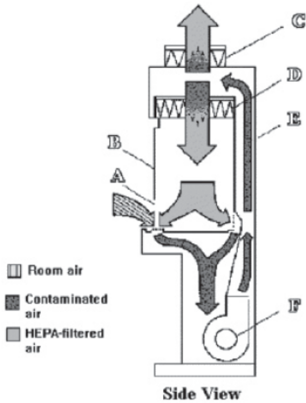
Figure 3. The Class II, Type A1 BSC. A. front opening, B. sash, C. exhaust HEPA filter, D. supply HEPA filter, E. common plenum, F. blower.
