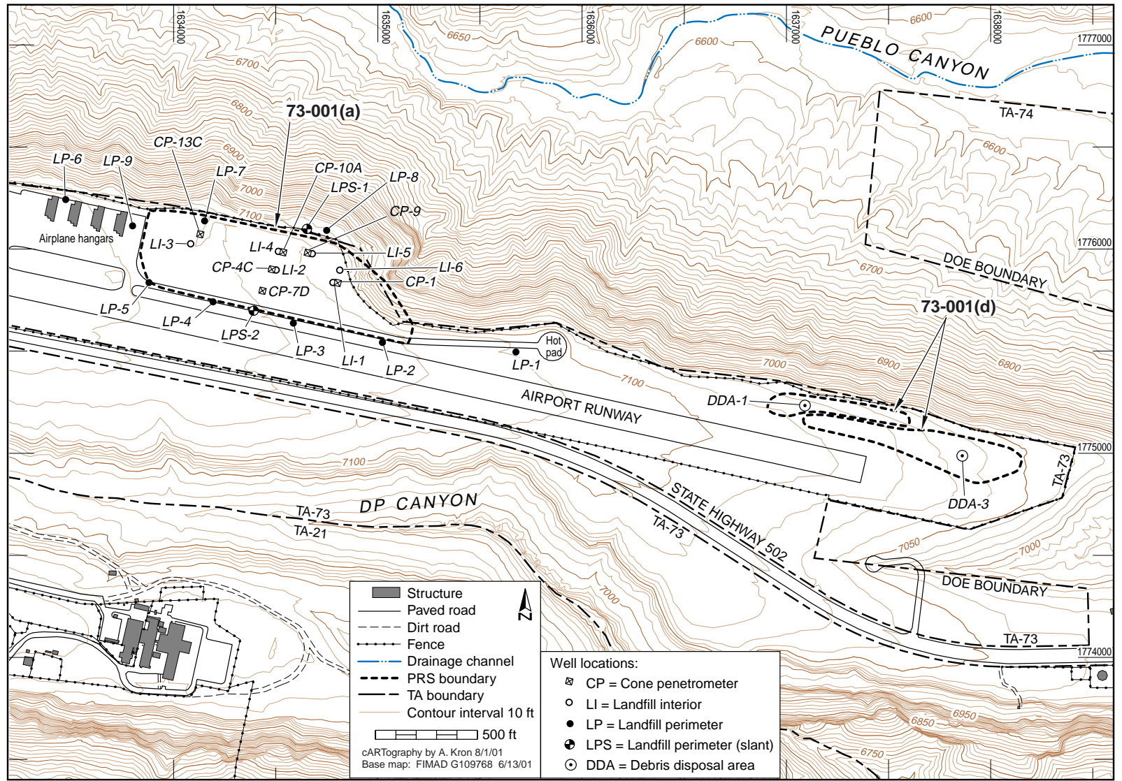
Figure 2.2-1. Locations of landfill interior and perimeter wells
