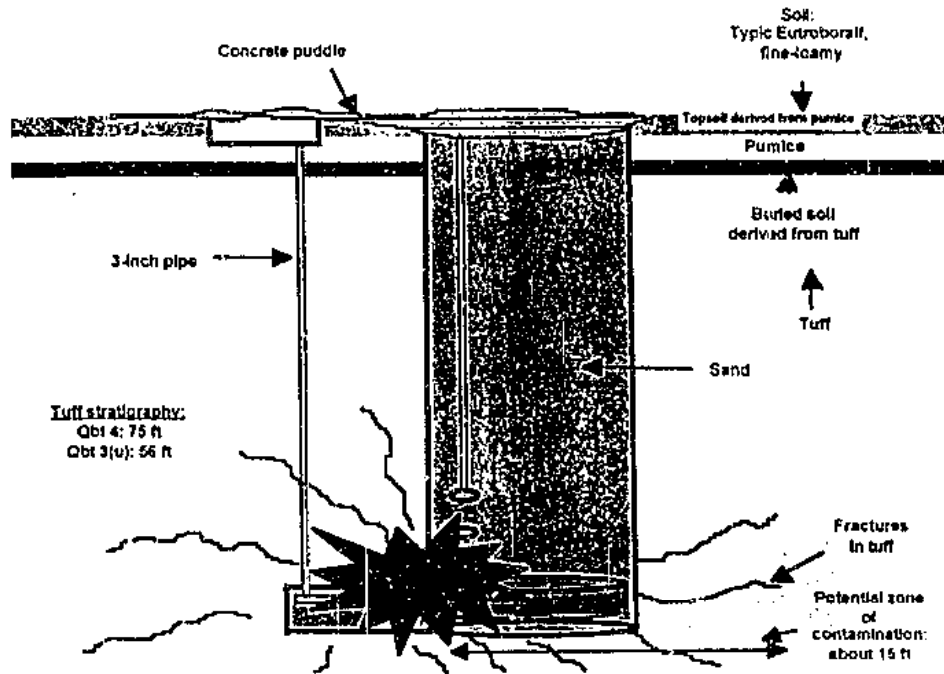
Figure 2-2. General configuration of test shaft and equipment at Areas 2, 2A, and 2B after detonation.
