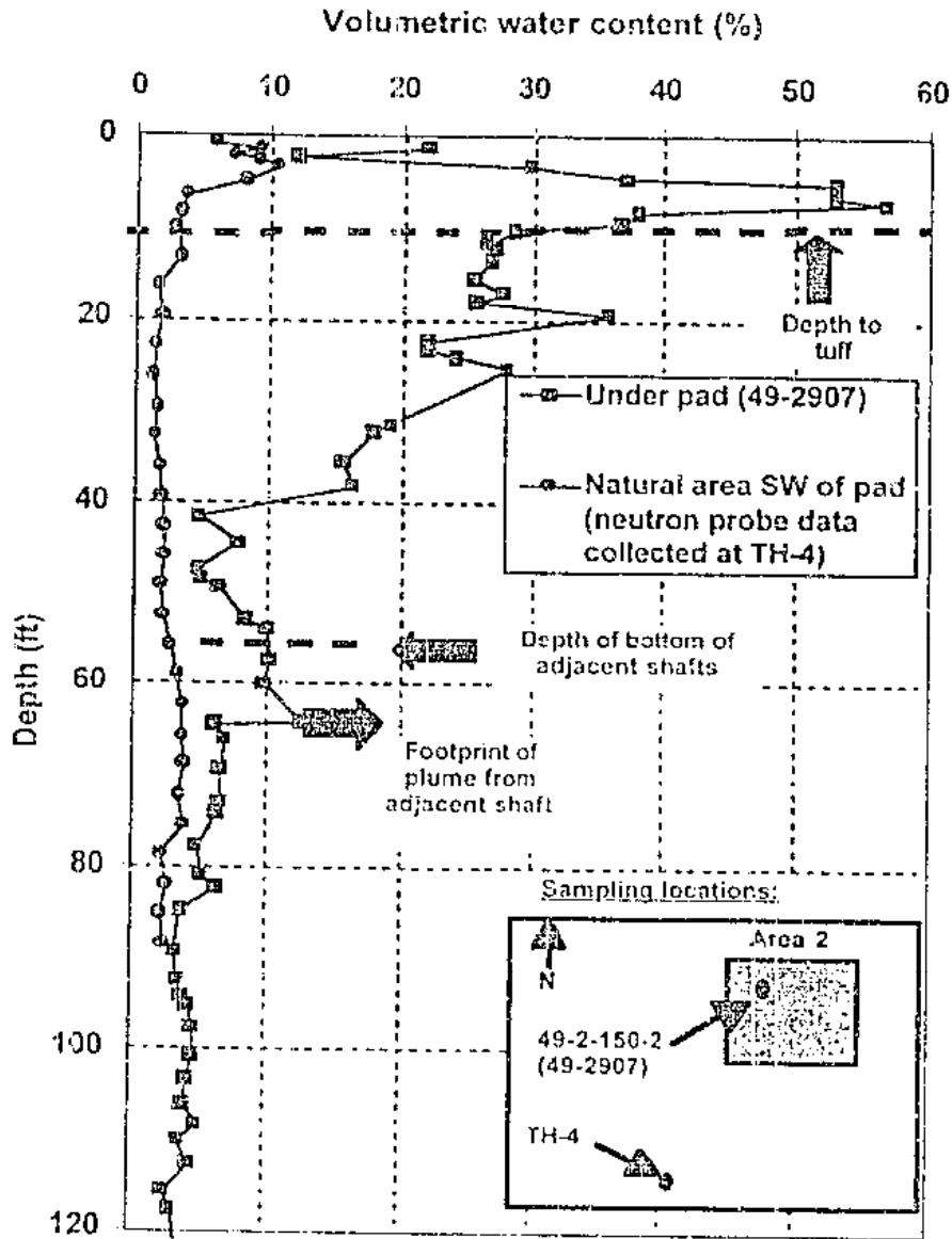
Figure 3-3. Subsurface moisture profiles at Area 2.
