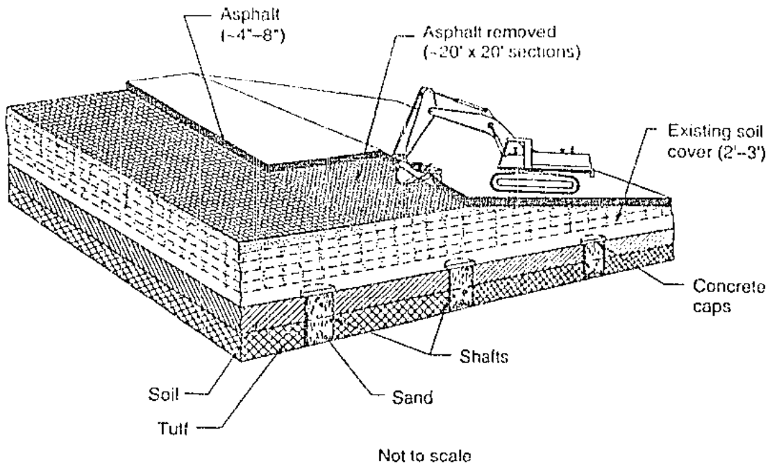
Figure 5-3. Illustration of asphalt pad and fill excavation methodology.
