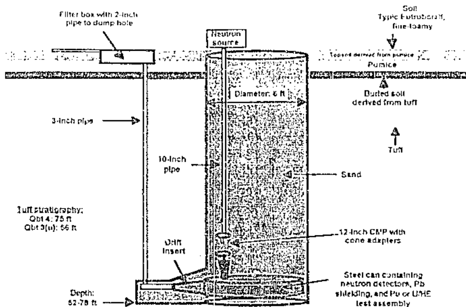
Figure 2-1. General configuration of test shaft and equipment at Areas 2, 2A, and 2B before detonation.
