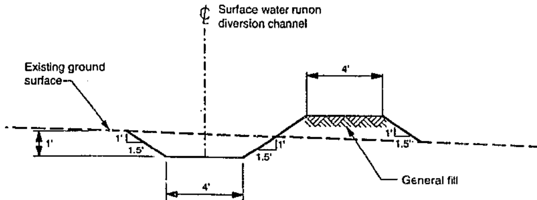
Figure 5-2. Schematic cross-section of surface water run-on diversion channel.
