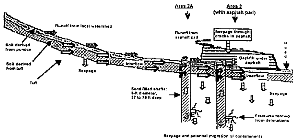
Figure 3-4. Conceptual hydrology of Areas 2 and 2A.
