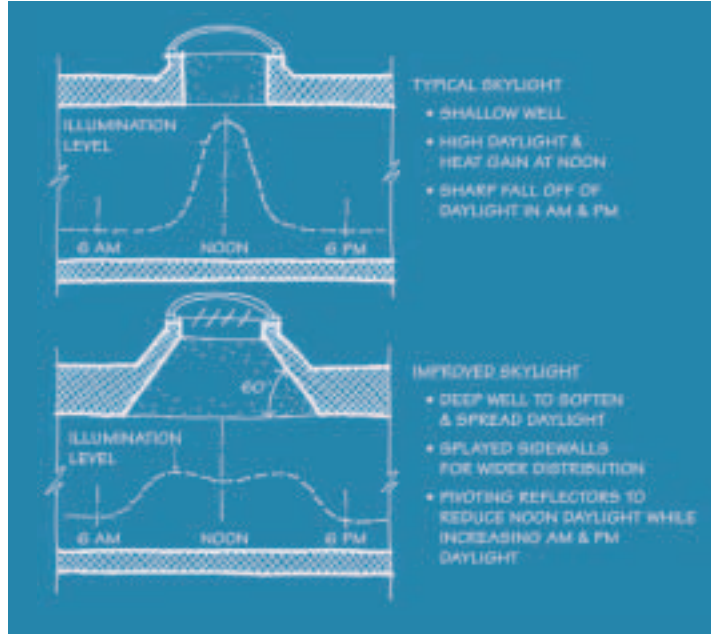
Skylight performance.
