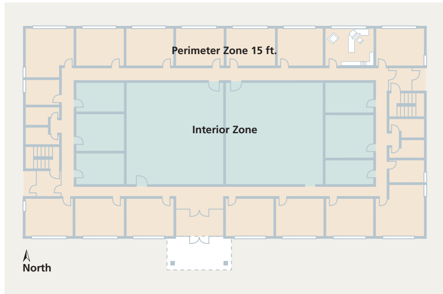
Typical HVAC zone design for a building with perimeter offices. Perimeter zones can extend from the exterior wall to the first interior wall, or for open floor plans, up to 15 feet from the exterior wall.
