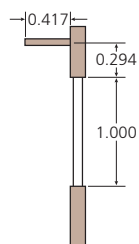
Shading Geometry in Dimensionless Units
