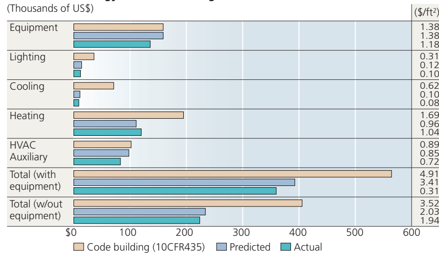
SERF Annual Energy Costs and Savings (Thousands of US$)
