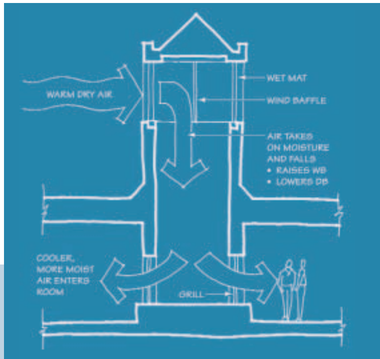
Cool moist air generated by air flowing through a wet medium at the top of the cooltower “drops” through large openings at the tower base to cool the space.
