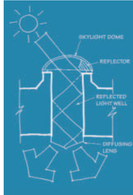
Lightpipe cross-section.
