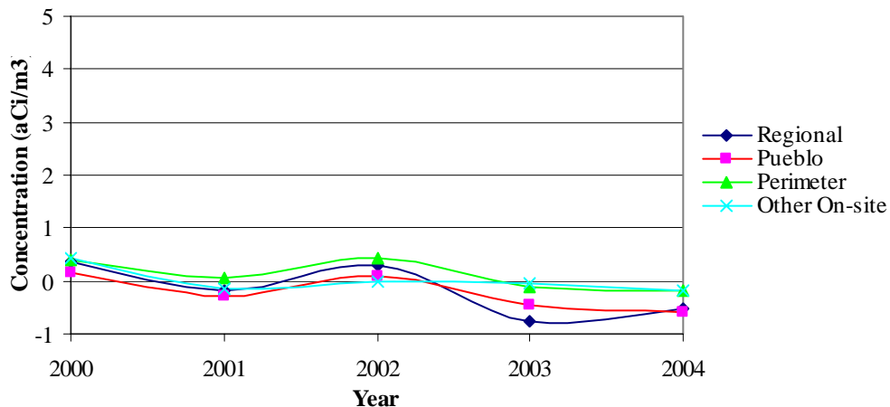
Figure 4-10. Am-241 concentration trends.
