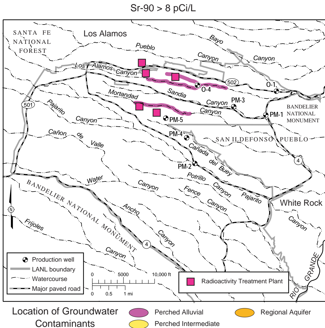
Figure 5-5. Location of groundwater contamination by strontium-90 above the 8 pCi/L EPA MCL. The maximum 2003 values in Mortandad and DP/Los Alamos Canyon alluvial groundwater were 10.2 and 7.6 times the MCL, respectively. Different colors indicate the affected groundwater zones. Along canyons, the extent of alluvial groundwater contamination lateral to the canyon is not to scale: contamination is confined to the alluvium within the canyon bottom and is narrow at the map scale.
