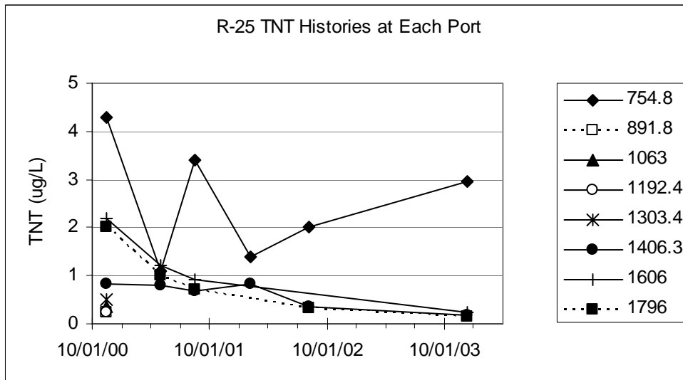
Figure 5-20. RDX and TNT histories at R-25 ports. The legend indicates the depth of the port in feet.
