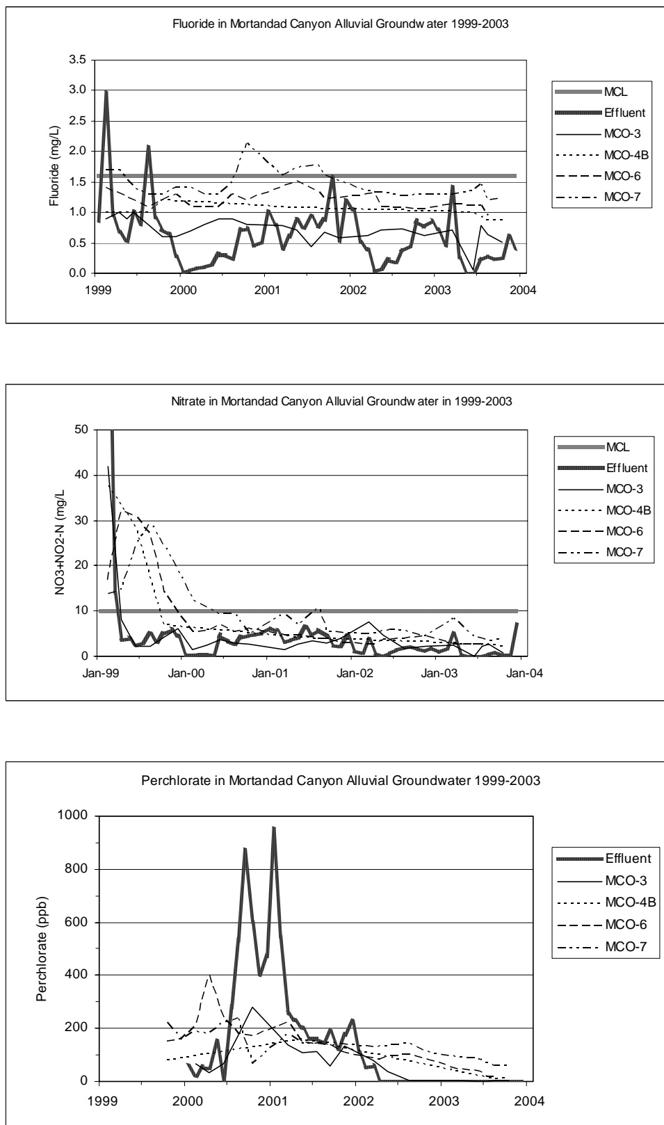
Figure 5-17. Fluoride, nitrate, and perchlorate in RLWTF effluent and Mortandad Canyon alluvial groundwater from 1999 through 2003.
