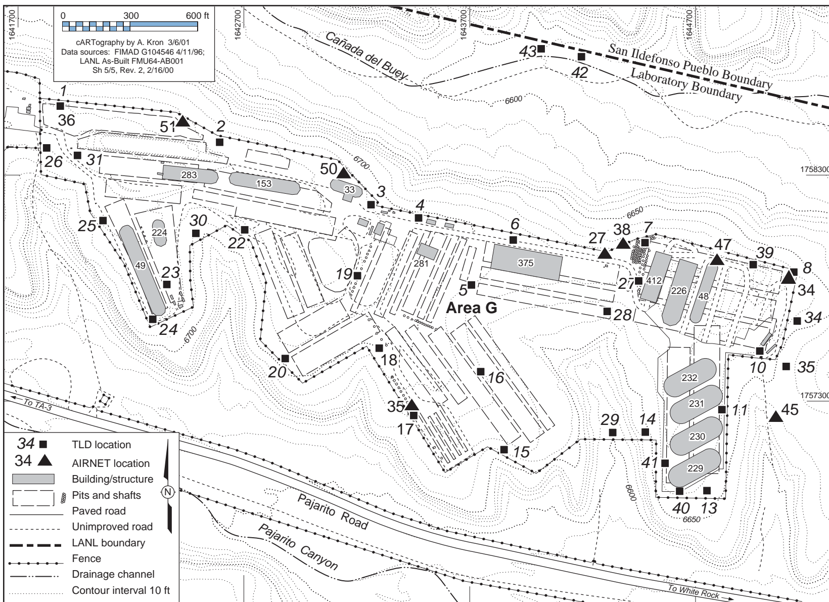
Figure 4-2. Technical Area 54, Area G, map of AIRNET and TLD locations.
