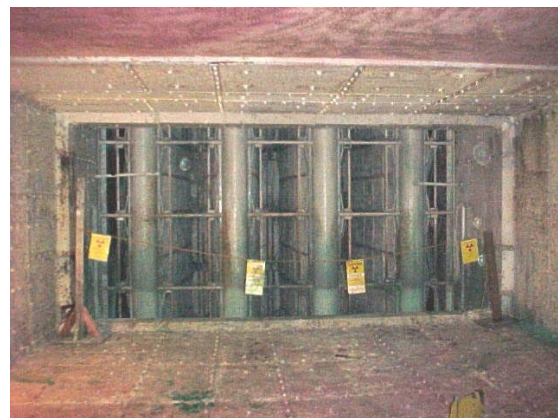
Exhibit 4-18: Filter Bank.
