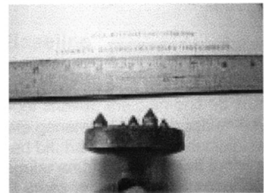
Piston head with bits for scabbler. Exhibit 3-38.
