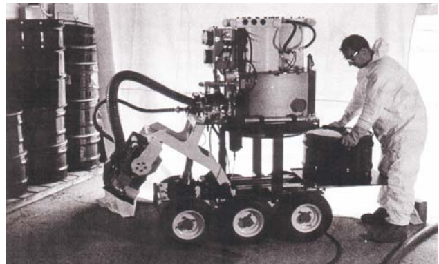
Pentek Vacuum System Exhibit 3-19
