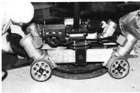
En-vac Robotic Wall Scabblers Exhibit 3-20.
