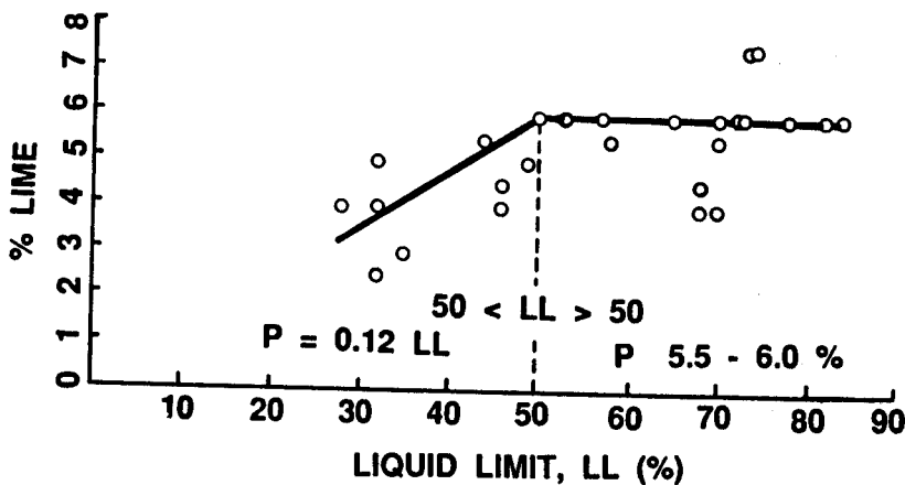
Percent of hydrated lime as a function of liquid limit
