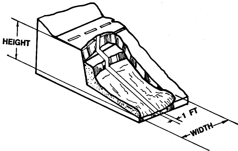
Dimensions of a slope failure required to estimate slope repair costs
