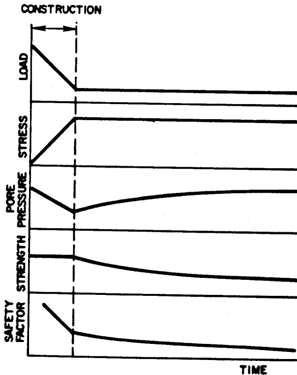
Long-term factor of safety of a highway cut section as function of time
