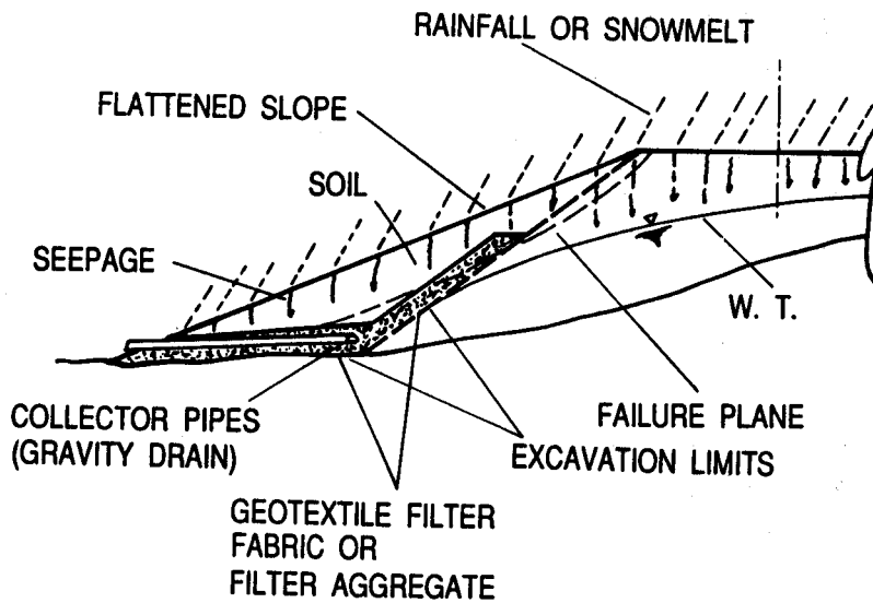
Use of a drainage blanket under a flattened slope to control surface seepage from rainfall and snowmelt and ground water seepage
