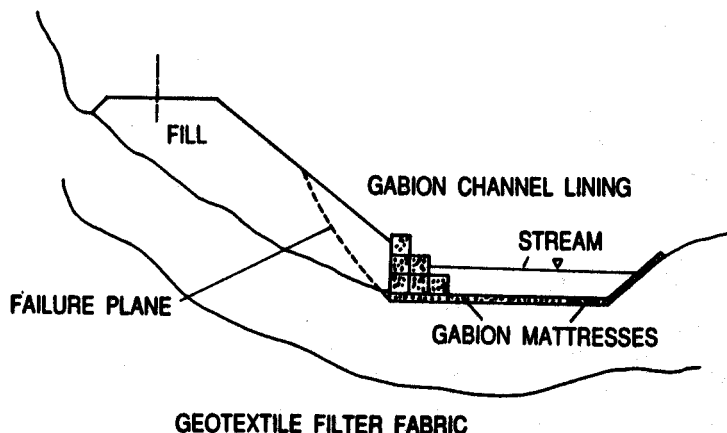
Lining channel of stream with gabion mattresses to prevent streambed erosion
