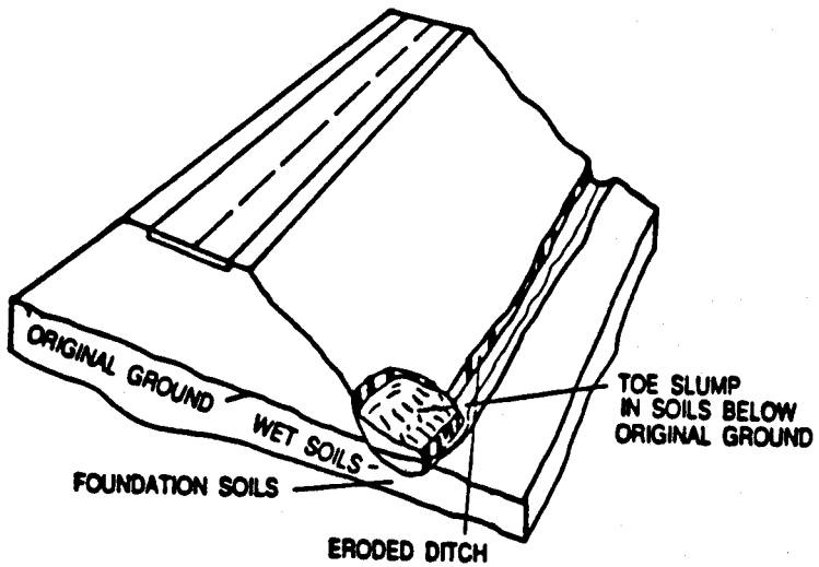
Toe slump in large fill and soils below original ground
