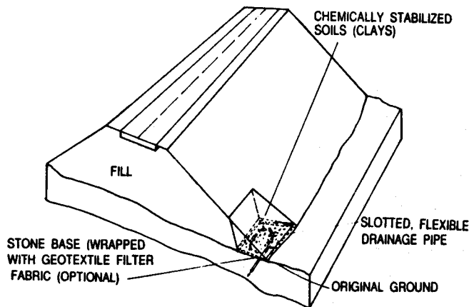
Repair of a toe slump using chemically stabilized soils
