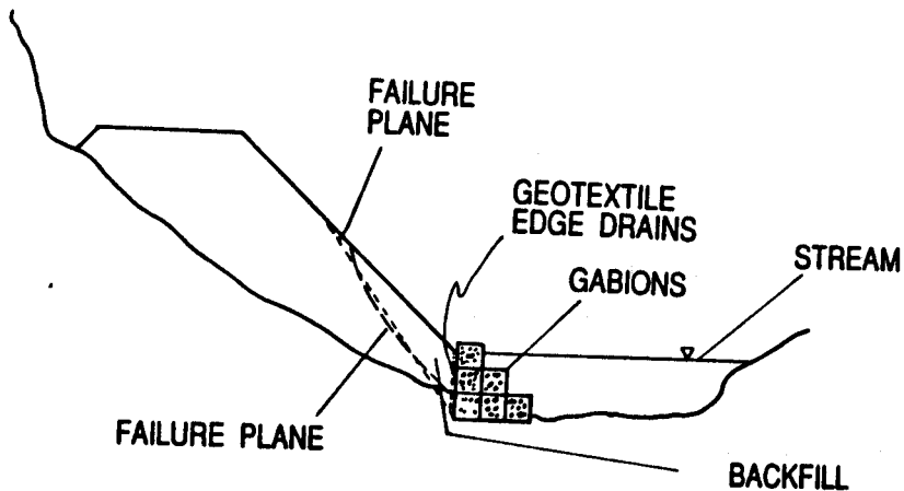
Portion of gabion wall buried below original ground
