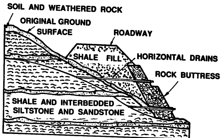
Rock buttress used to repair a highway slope failure
