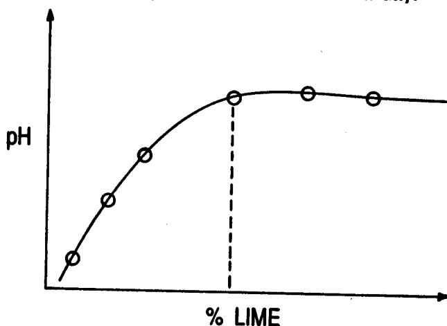
Relationship between pH and percent of hydrated lime
