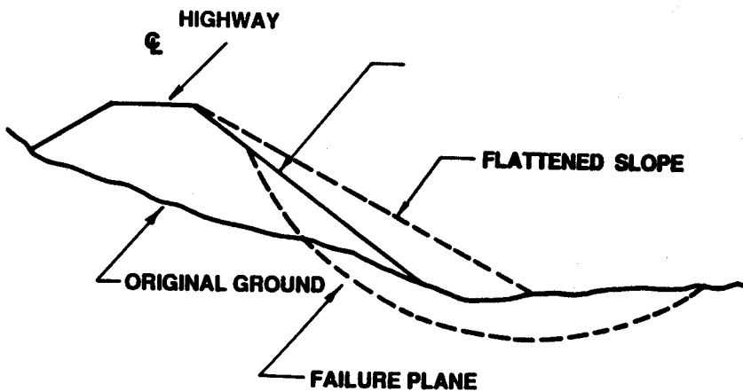
incorrect application of a flattened slope
