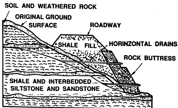
EMBANKMENT REPAIR I 75 (TN)
