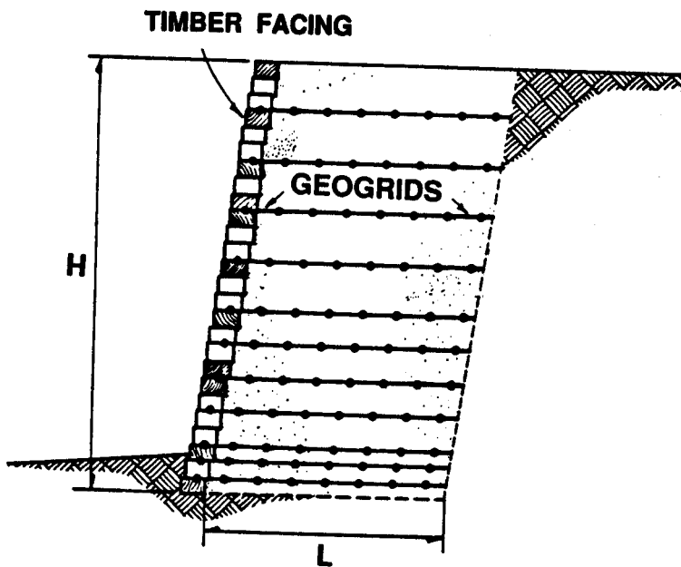
Use of timber facing to protect geotextile material
