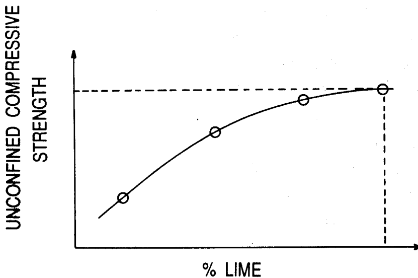
Unconfined compressive strength as a function of percent of hydrated lime
