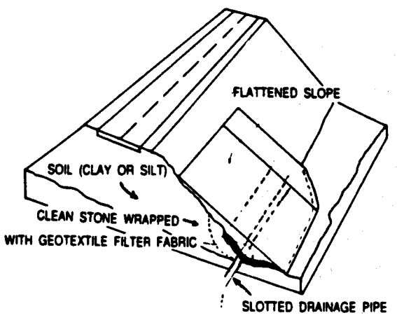
Toe slump in fill
