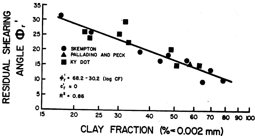
Residual angle of internal friction as a function clay fraction (percent finer than .002 mm)
