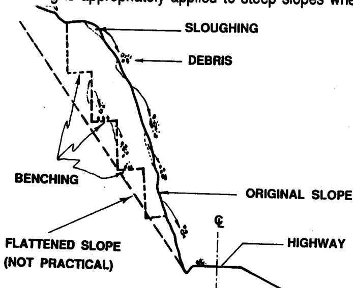
Benching of a problem slope
