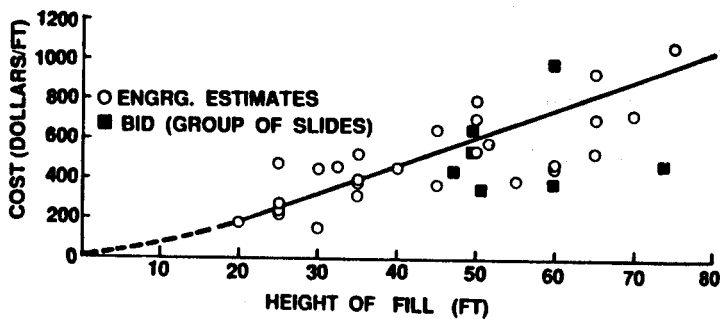
Repair cost of berm and / or flattened slope per linear foot of slope failure and height of fill ( or height of slope failure )
