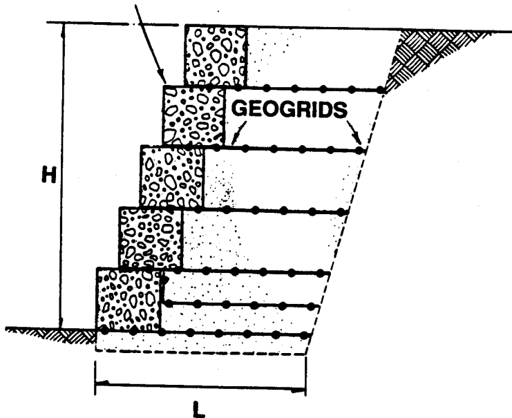
Use of gabion facing to protect geotextile material
