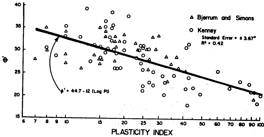
Peak effective stress value of the angle of internal friction as a function of plasticity index
