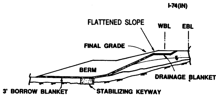
Use of a keyway shear trench combined with a flattened slope and berm to stabilize a slope failure
