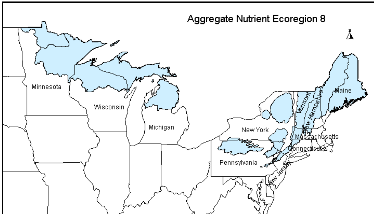
Figure 1. Aggregate Ecoregion VIII
