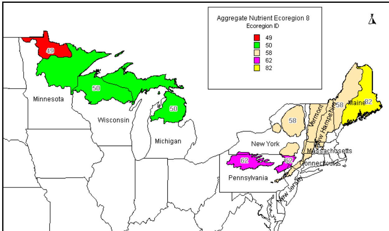
Figure 2. Aggregate Ecoregion VIII with level III ecoregions shown
