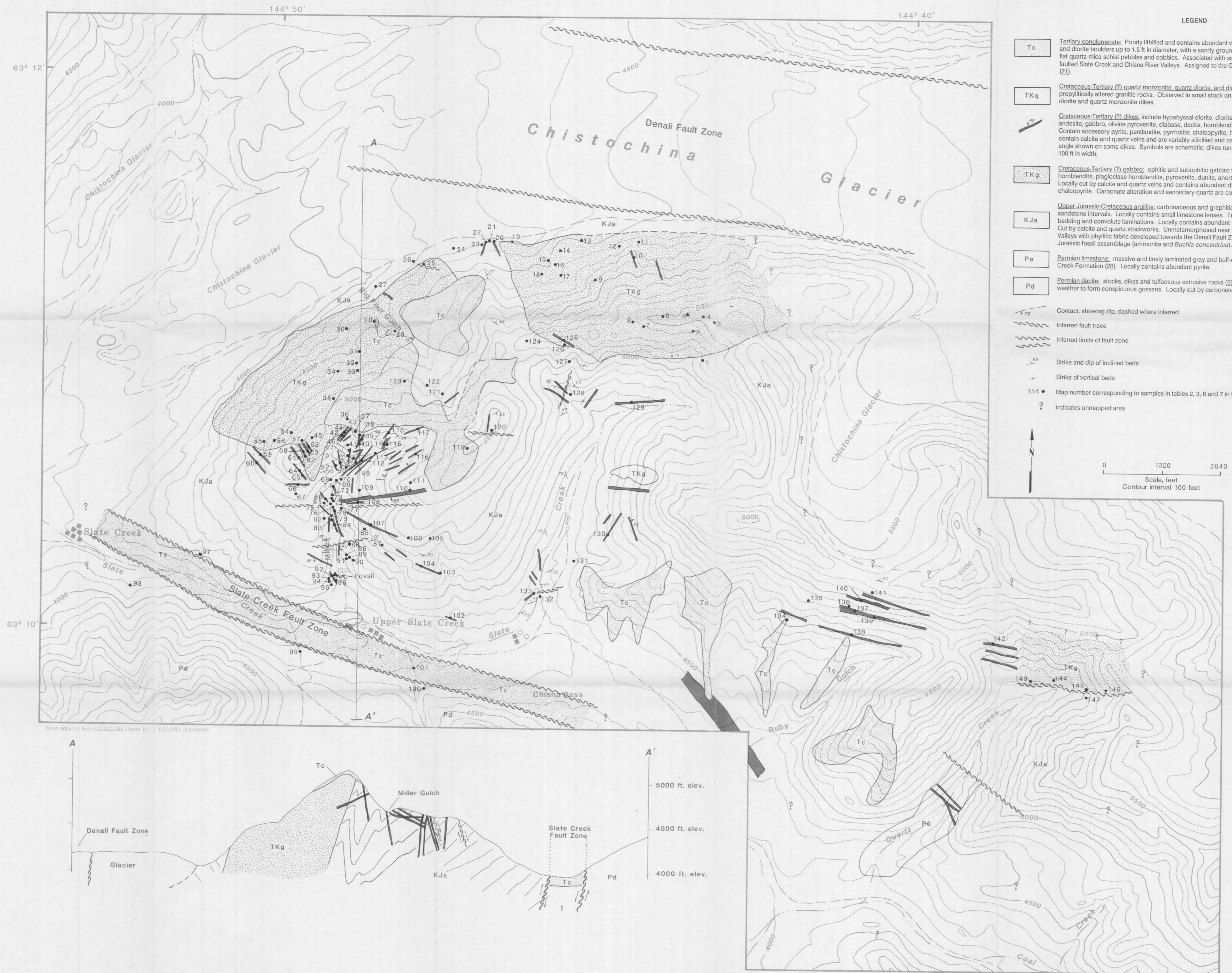
Figure 2. - Geologic map of the Slate Creek area, showing sample localities and cross section.
