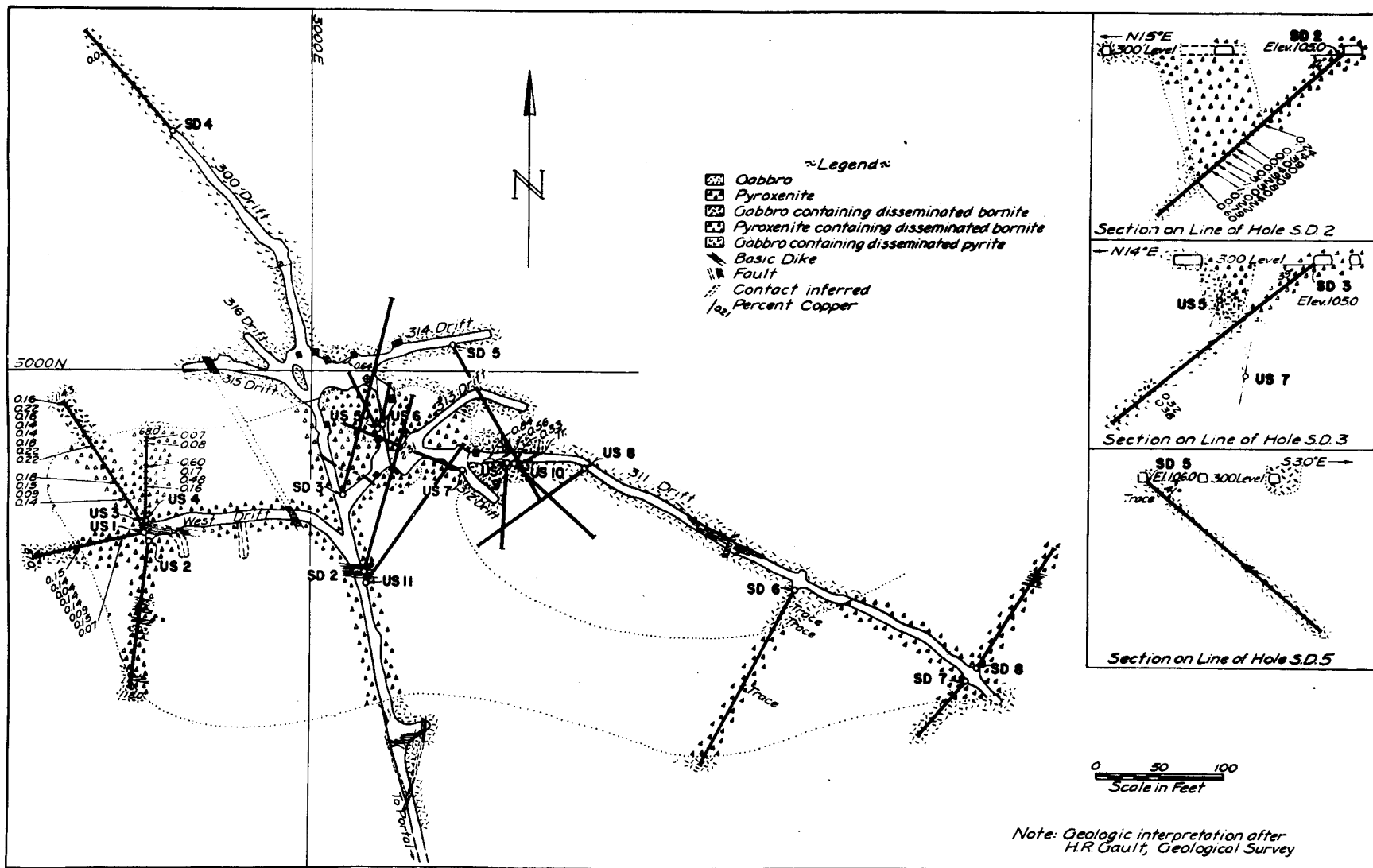
Figure 4. - 300 level, Salt Chuck mine.
