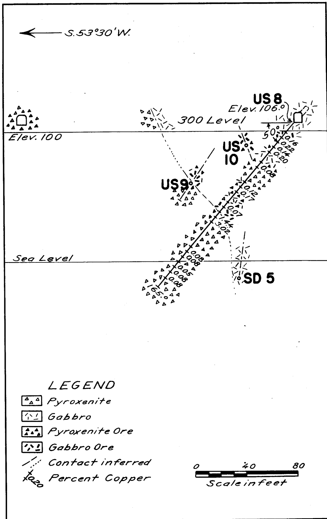
Figure 11. - Section on line of hole U.S. 8.
