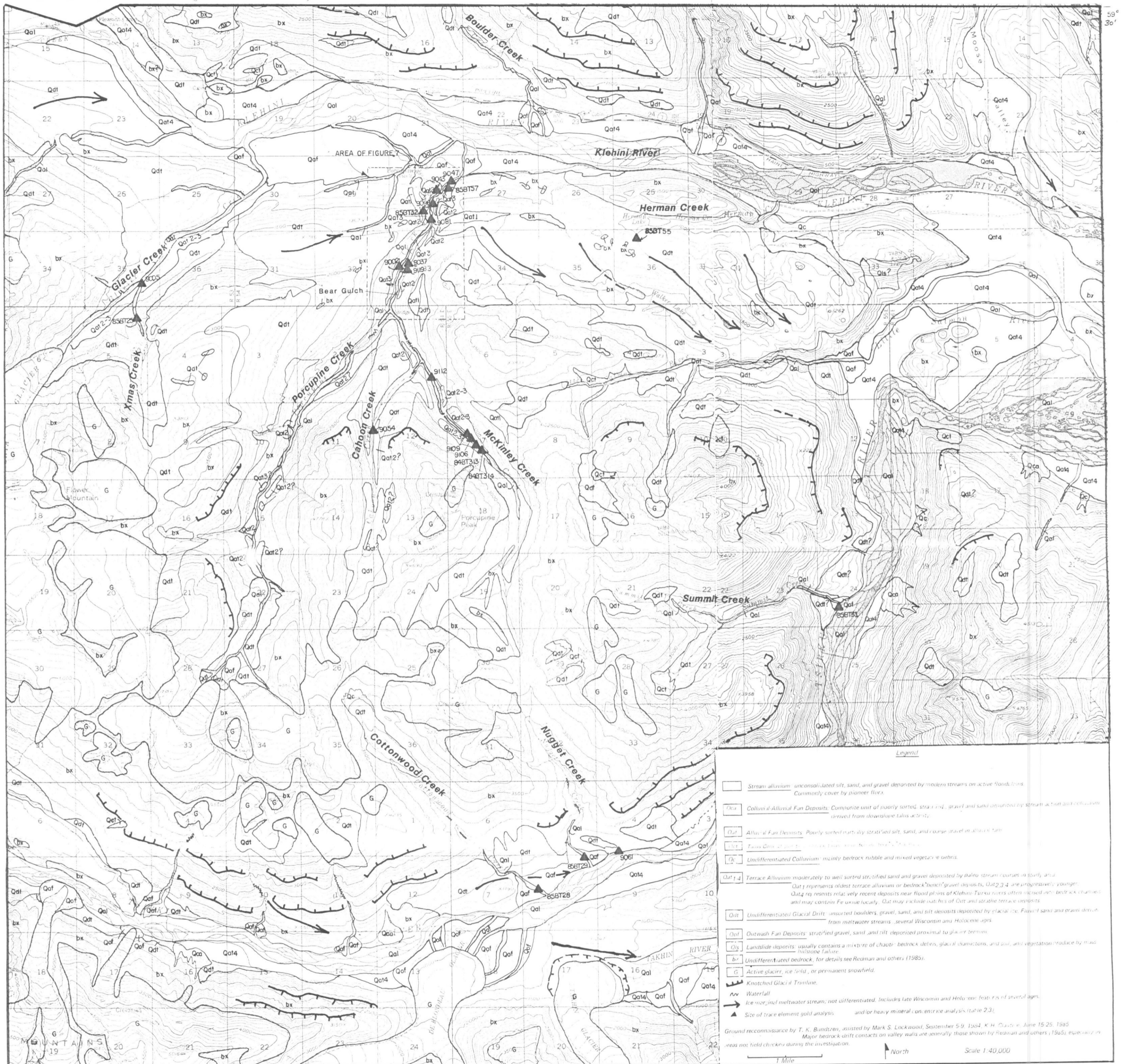
QUATERNARY-PLACER GEOLOGY OF PORCUPINE DISTRICT, ALASKA
