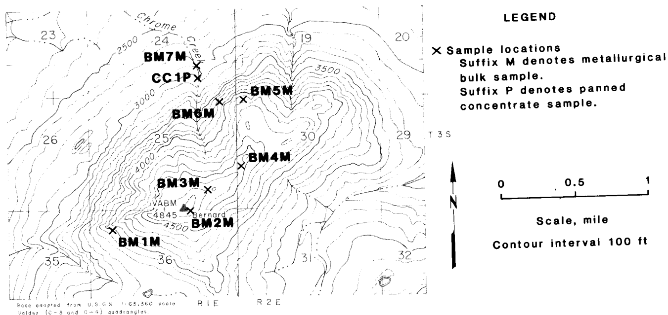
FIGURE 8. - Sample locations at Bernard Mountain.
