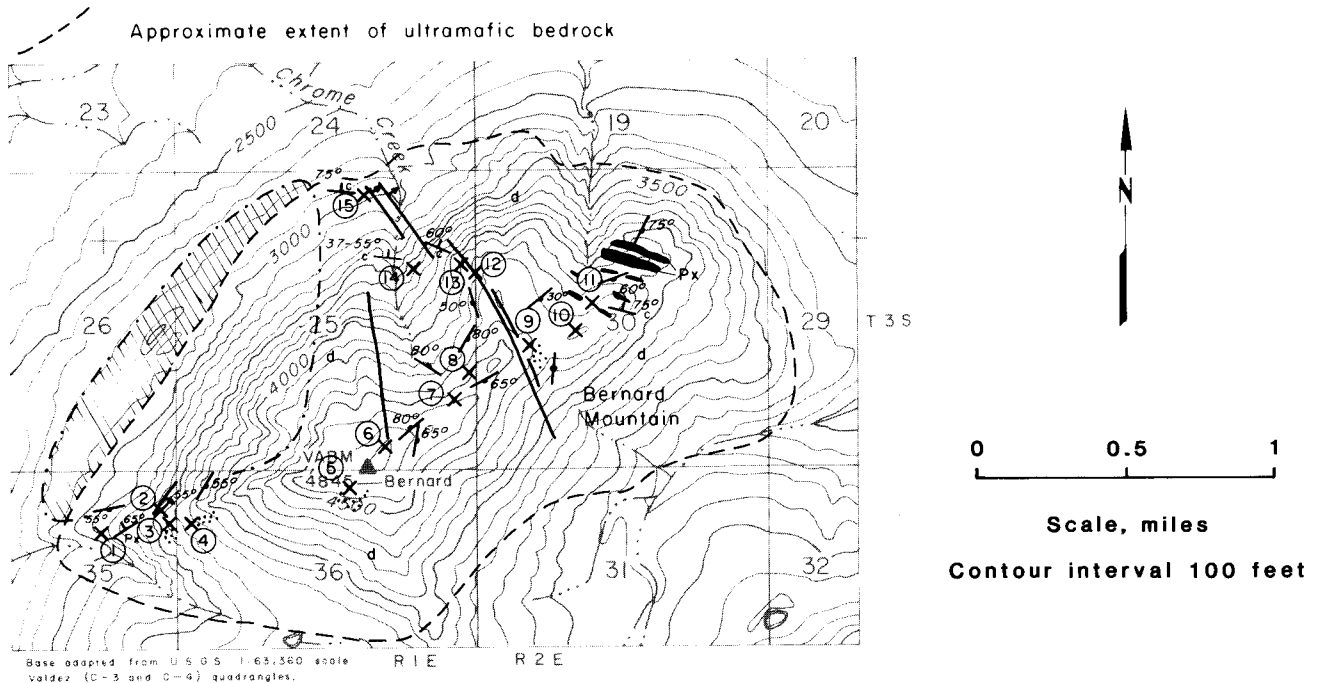
FIGURE 7. - Simplified geologic map and locations of chromite occurrences at Bernard Mountain.
