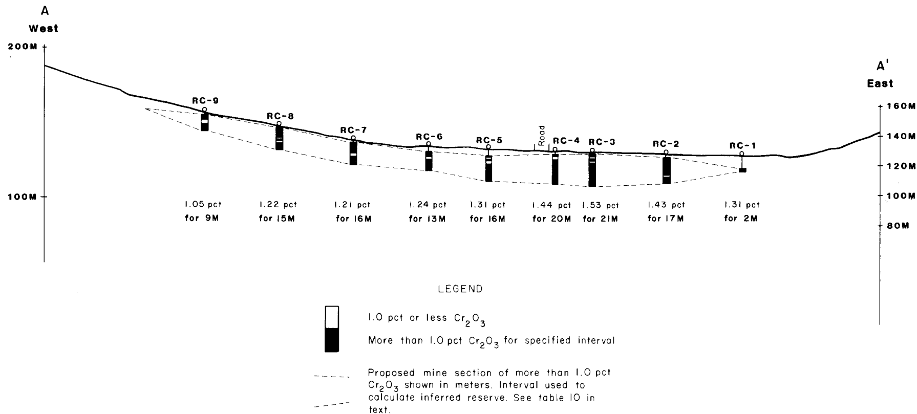
FIGURE 22. - Drill hole profile of Windy River Valley (looking north). (Adapted from Anaconda Minerals Co. data compiled by W. T. Ellis, 1983)
