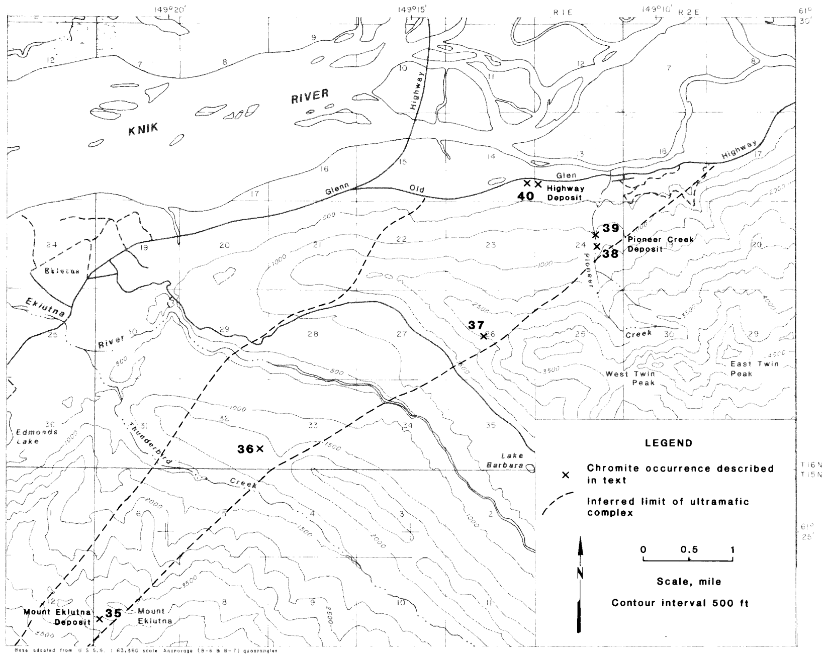
FIGURE 16. - Location of chromite deposits at the Eklutna complex. (After Rose (42), fig. 2))
