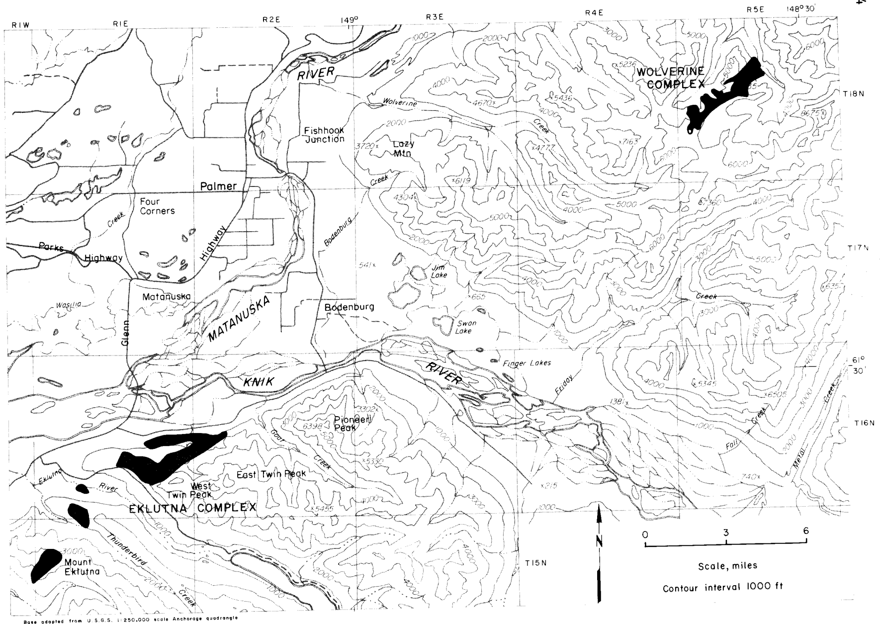
FIGURE 13. - Mafic-ultramafic complexes near Palmer.
