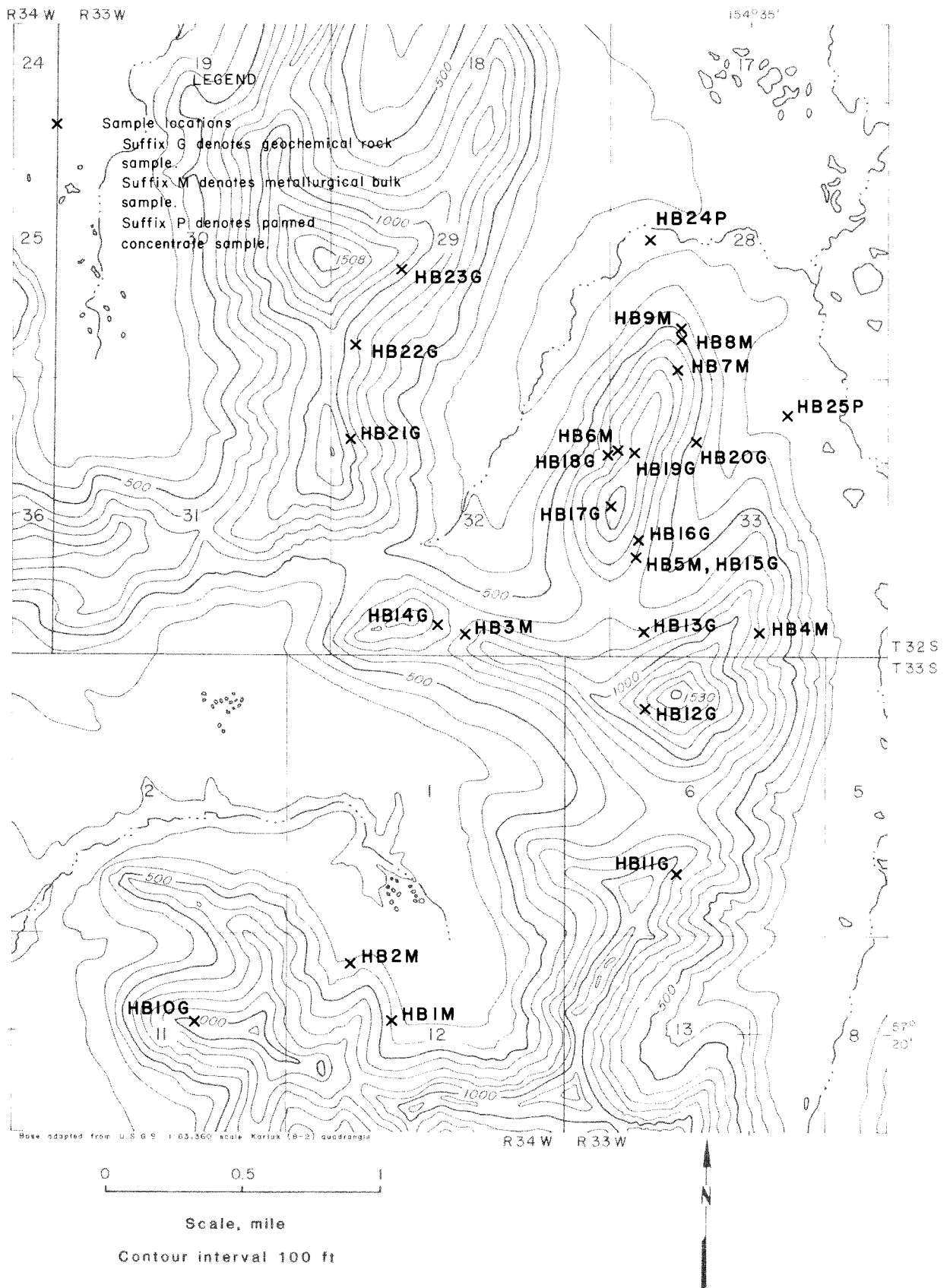
FIGURE 26. - Sample locations at the Halibut Bay complex.
