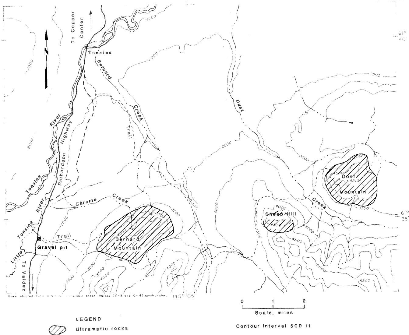
FIGURE 5. - Ultramafic complexes near Tonsina.
