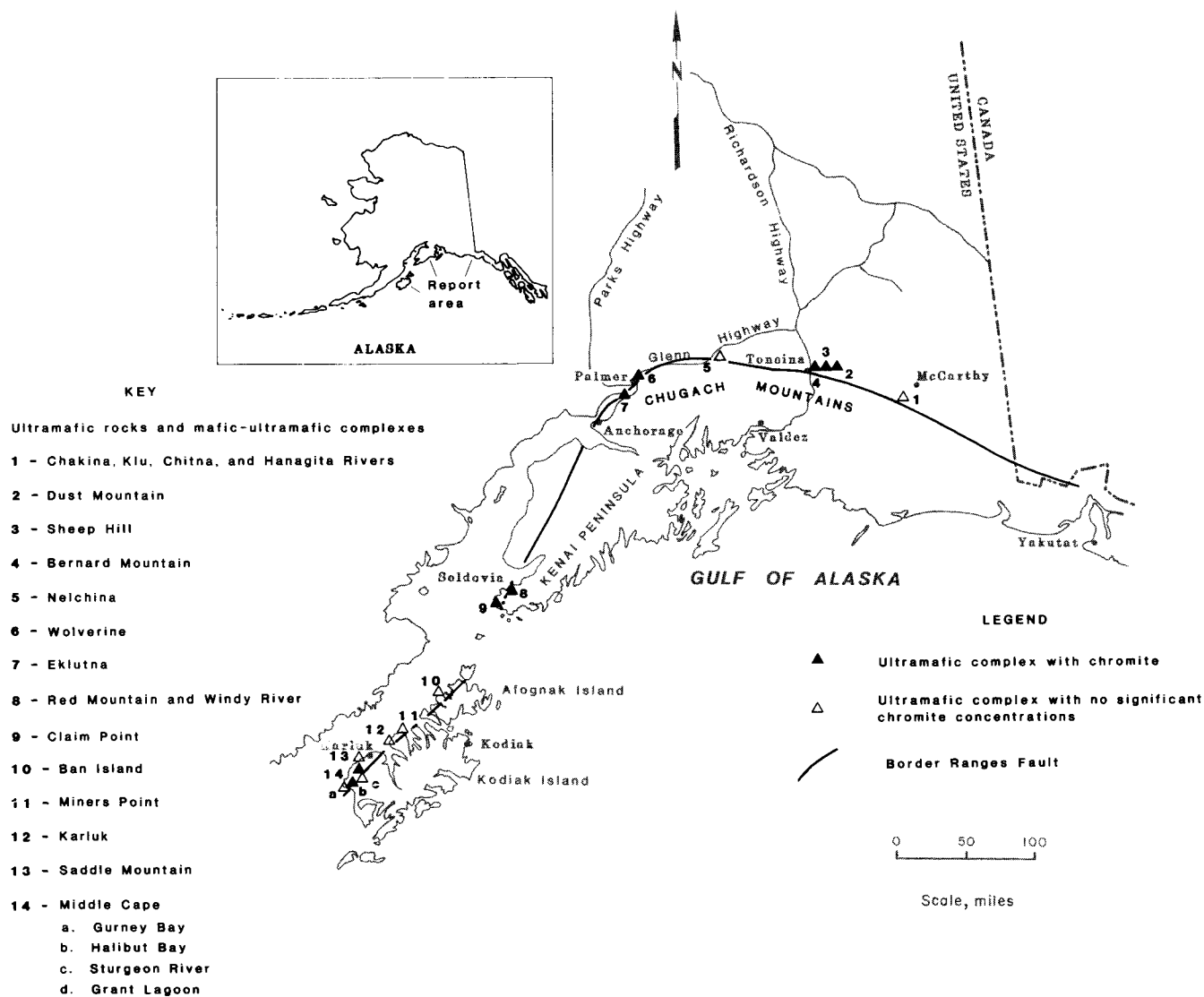
FIGURE 1. - Map of southern Alaska showing ultramafic and mafic-ultramafic complexes along the Border Ranges Fault.
