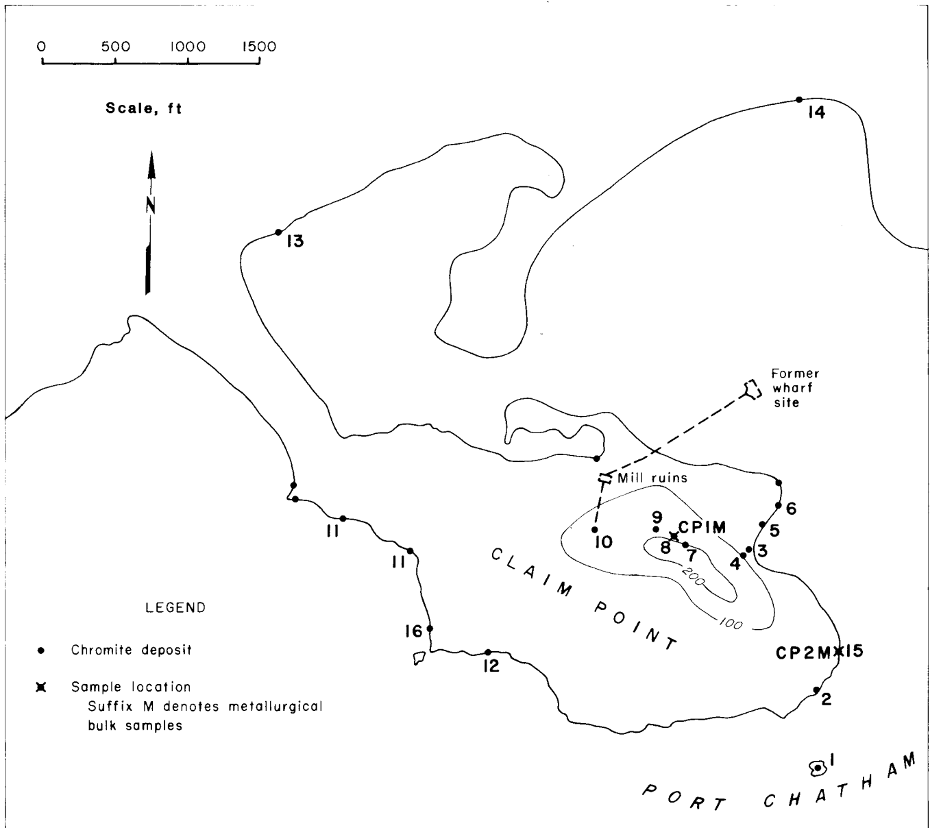
FIGURE 23. - Chromite deposits and sample locations at Claim Point. (After Guild (17, plate III) and Sanford and Cole (44, fig. 3))
