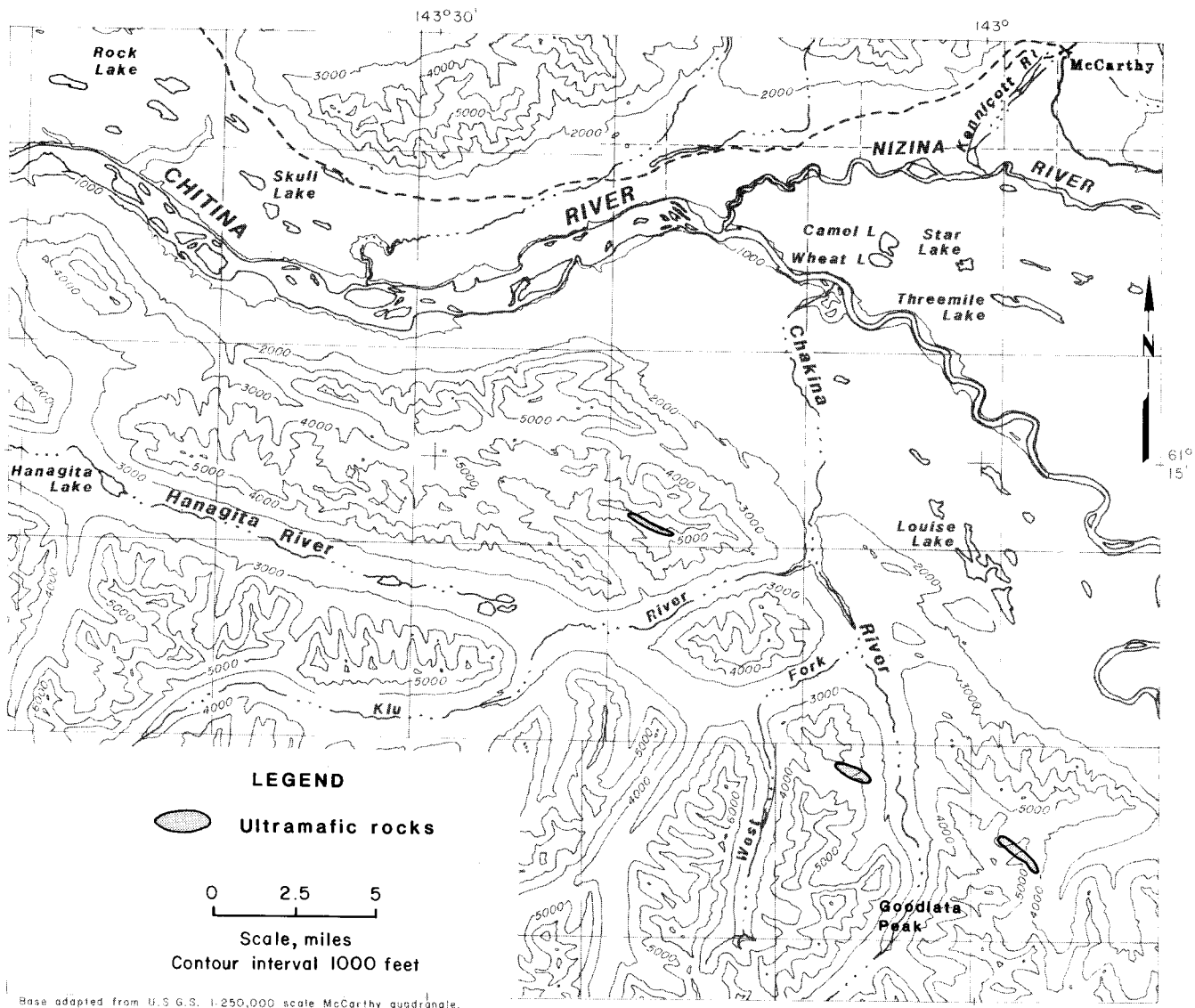
FIGURE 4. - Ultramafic rocks near McCarthy. (After MacKevett (25))
