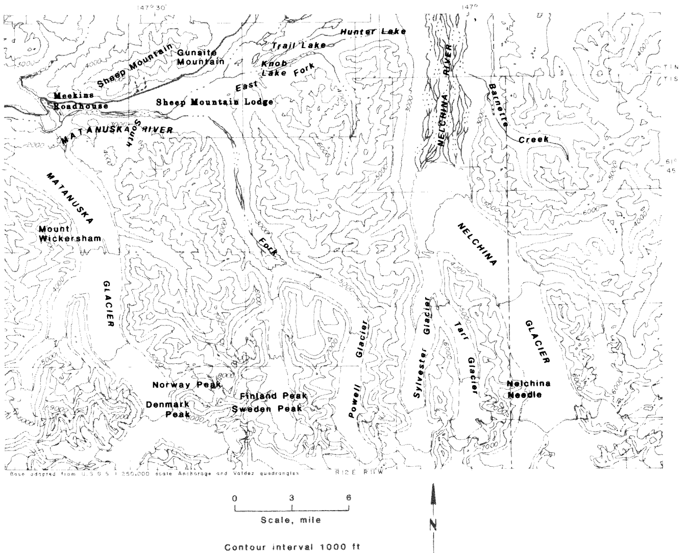
FIGURE 12. - Map of Nelchina Glacier and Matanuska River areas.
