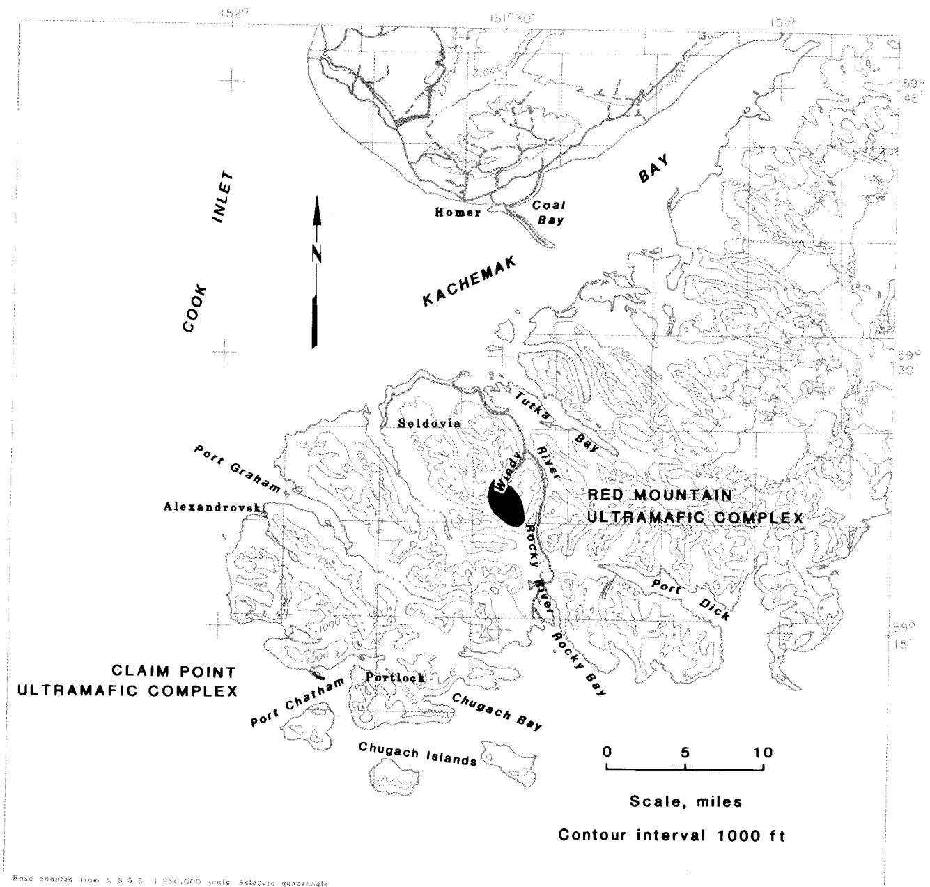
FIGURE 17. - Locations of Red Mountain and Claim Point ultramafic complexes on Kenai Peninsula. (After Gill (16, plate I) and Sanford and Cole (44, fig. 2))
