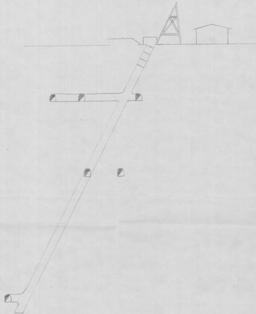
Section New Shaft
