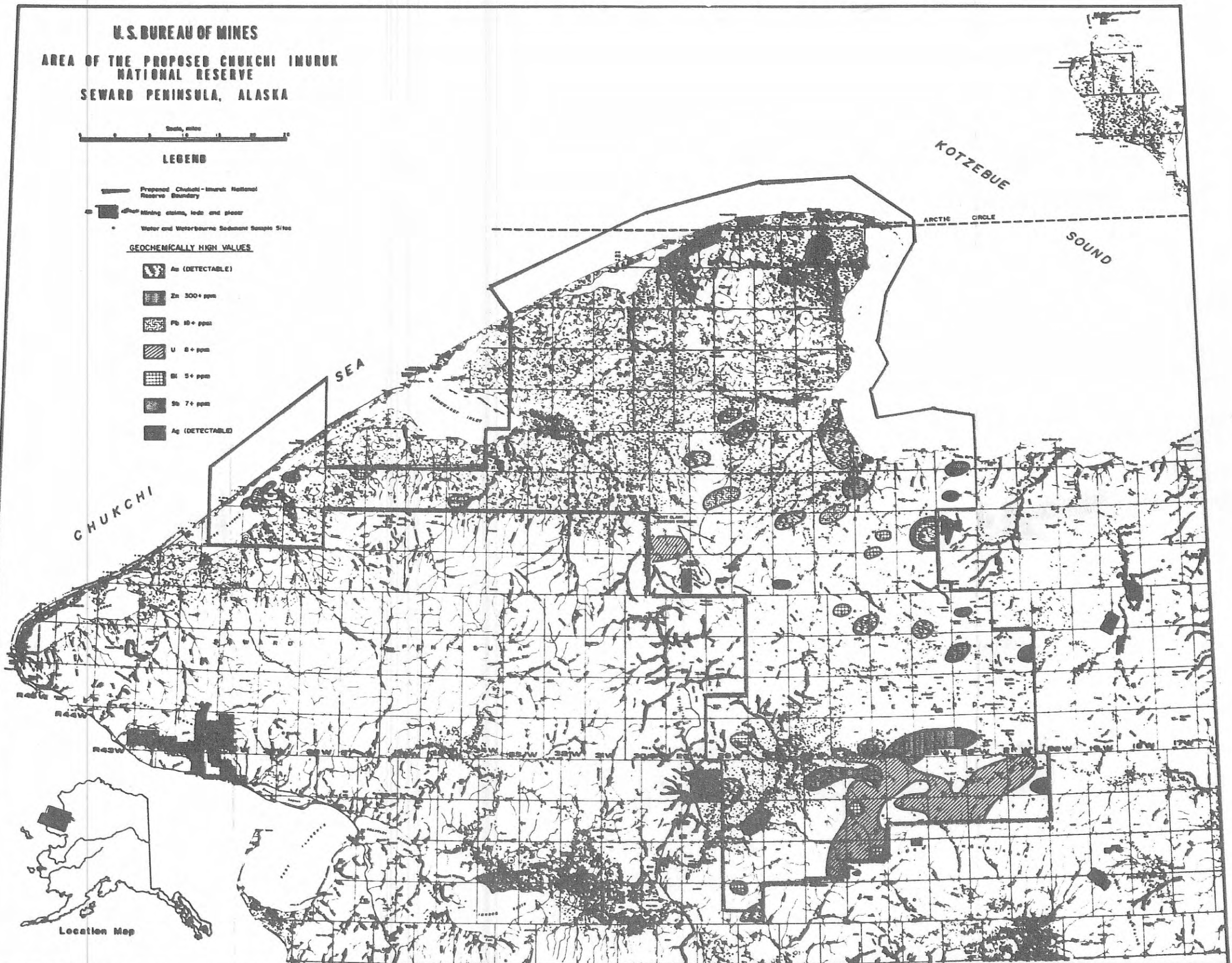
FIGURE 2 GEOCHEMICAL ANOMALIES AND MINING CLAIMS MAP, NORTHWESTERN SEWARD PENINSULA, ALASKA
