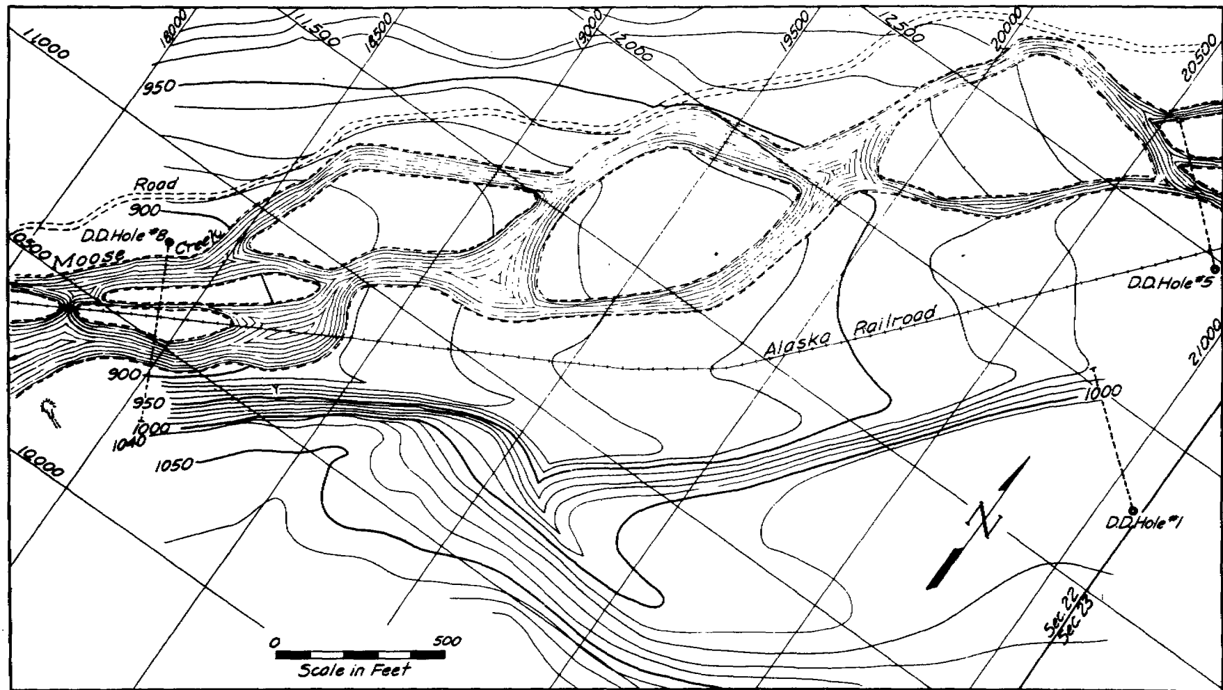
FIGURE 7.- Topographic map of region between Buffalo and Baxter mine areas.
