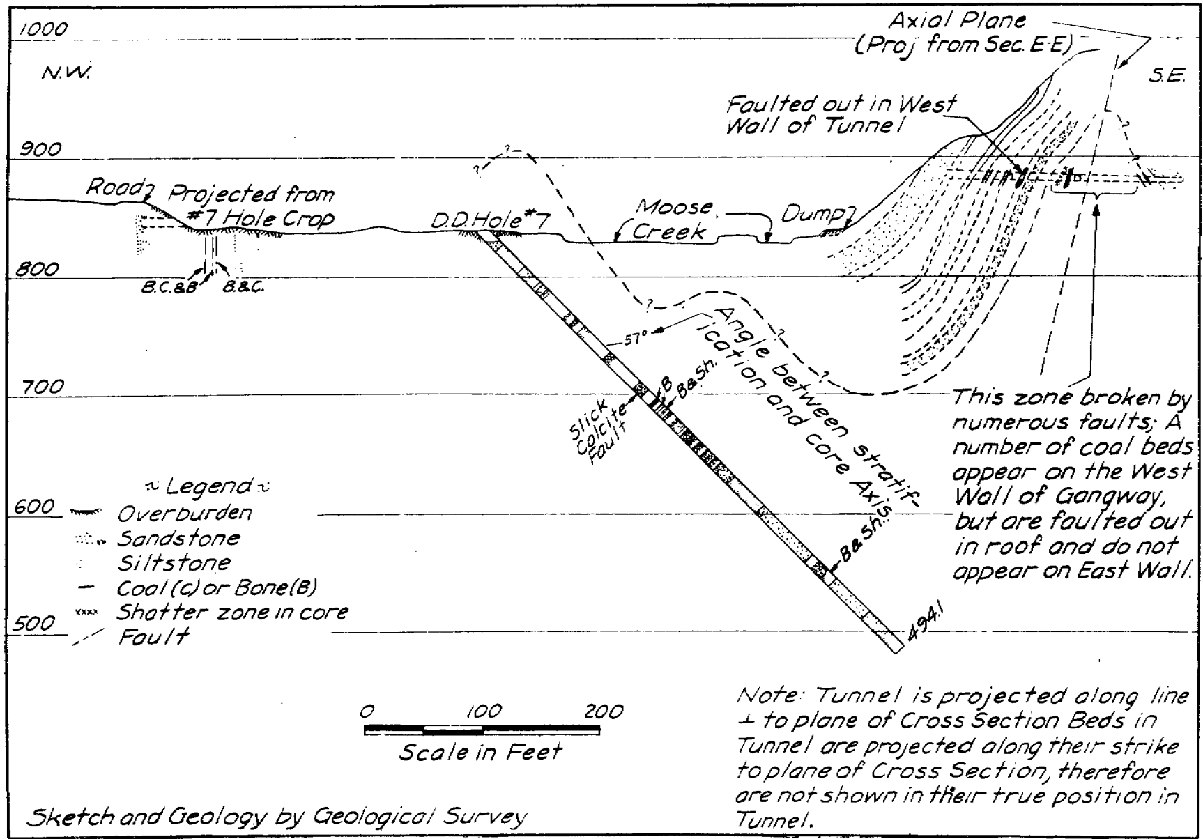
FIGURE 18.- Geologic section B-B through diamond drill hole 7.
