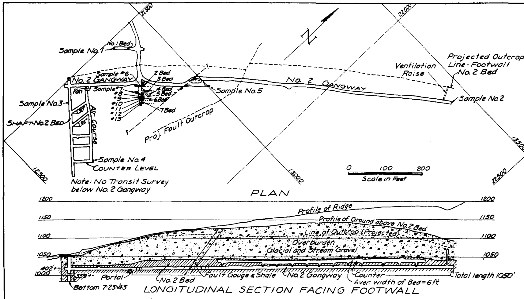
FIGURE 13.- Plan and section of Buffalo mine.
