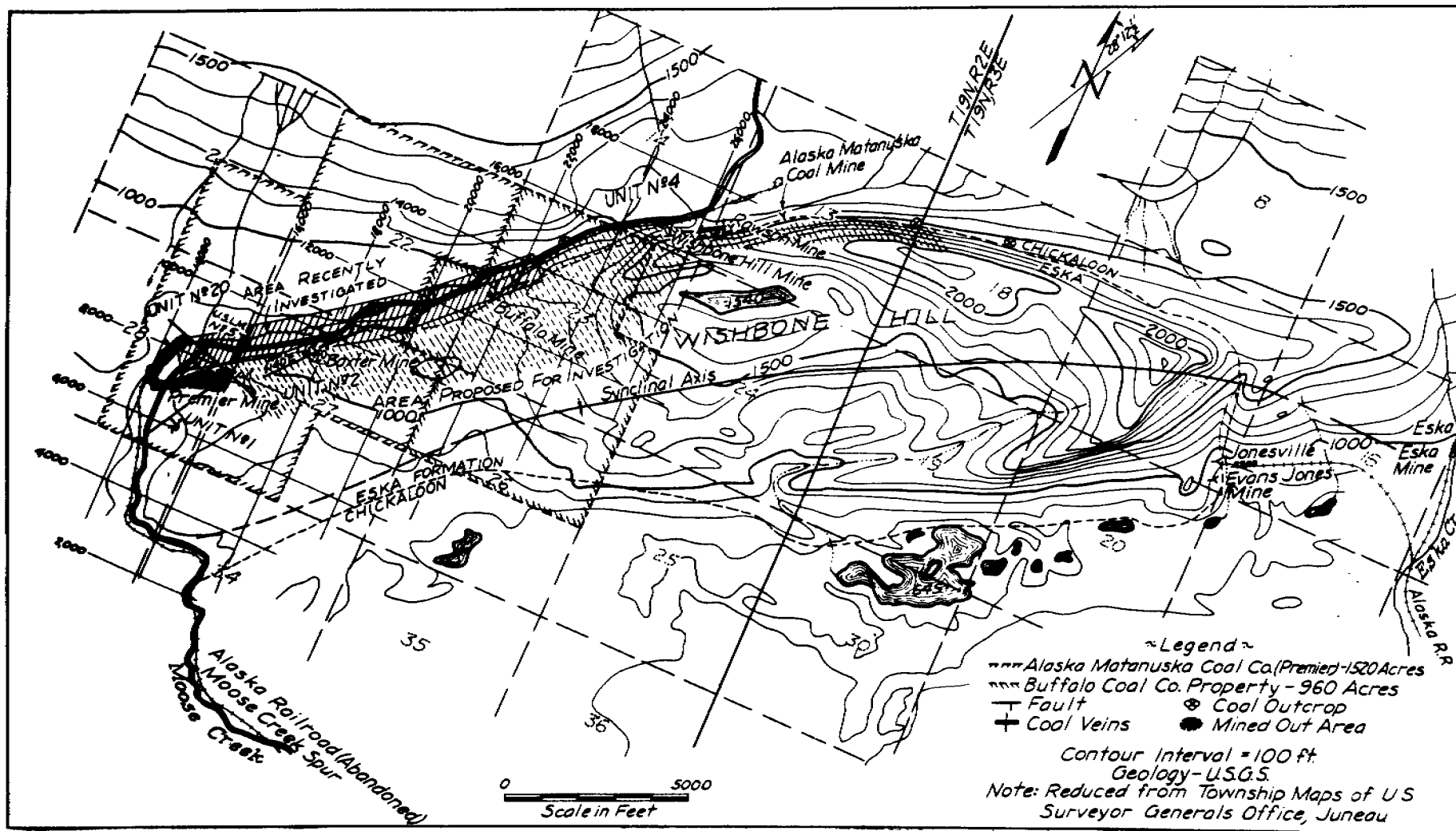
FIGURE 2.- Matanuska coal field, Moose Creek coal mines.
