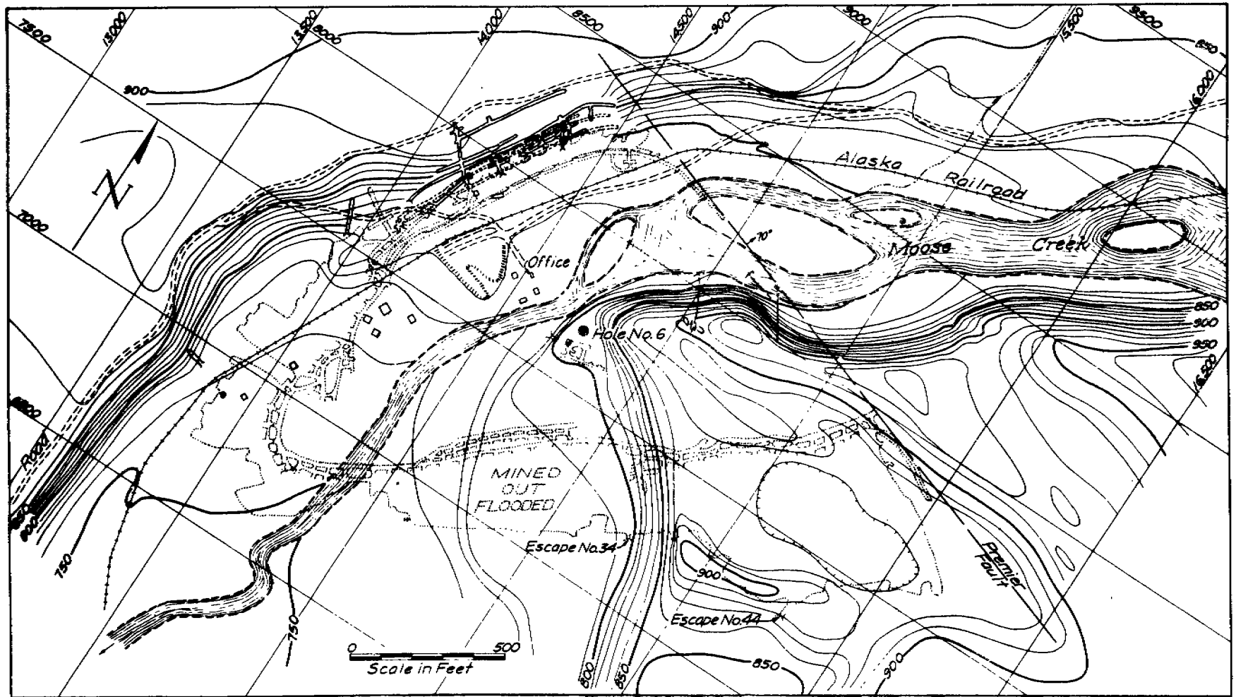
FIGURE 9.- Topographic map of Premier mine area.
