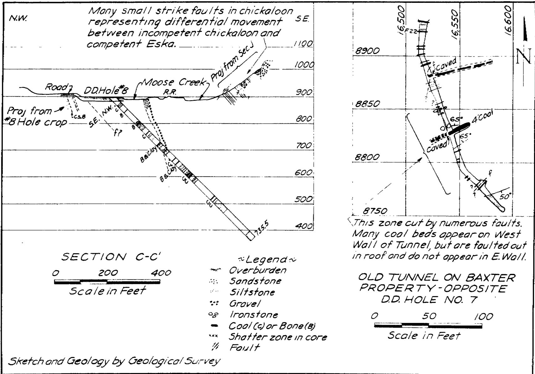
FIGURE 19.- Geologic section C-C through diamond drill hole 8, and plan of tunnel opposite hole 7.
