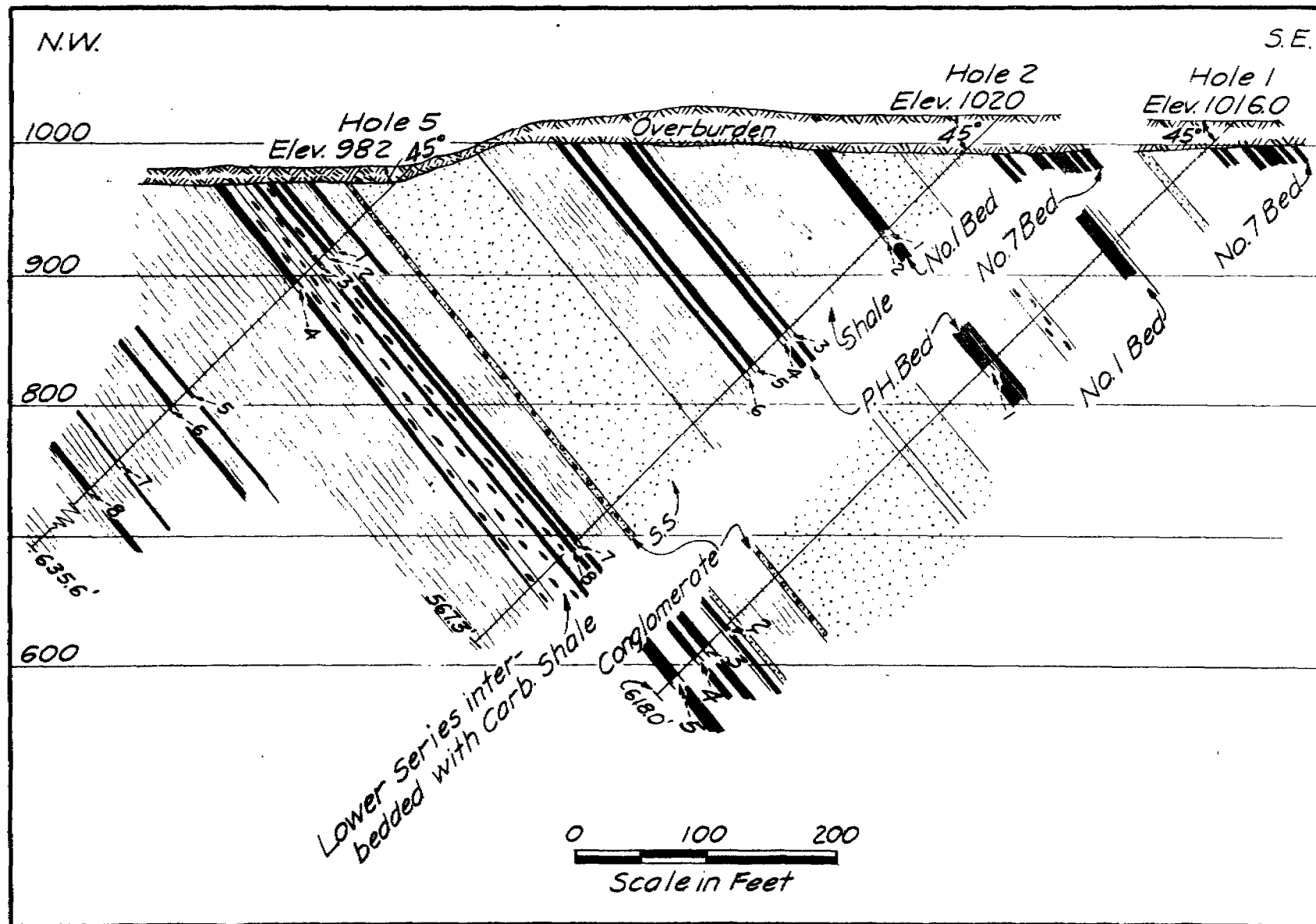
FIGURE 15.- Sections through diamond drill holes 1, 2, and 5.
