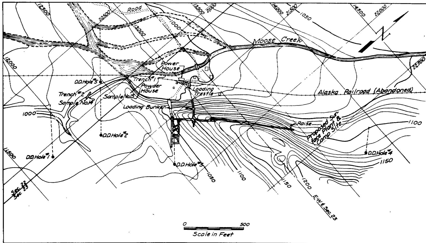
FIGURE 6.- Topographic map of Buffalo mine.
