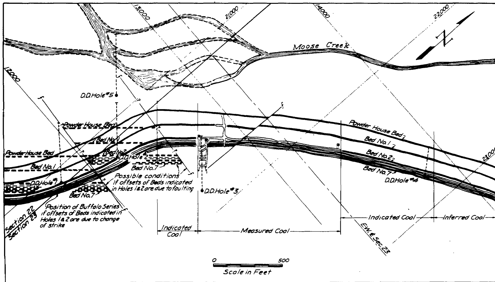
FIGURE 16.- Diagrammatic sketch, Buffalo series.
