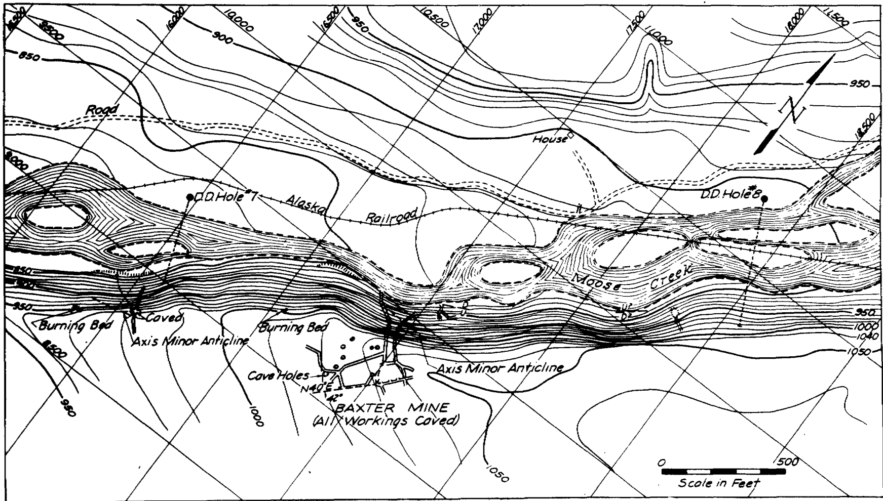
FIGURE 8.- Topographic map of Baxter mine area.
