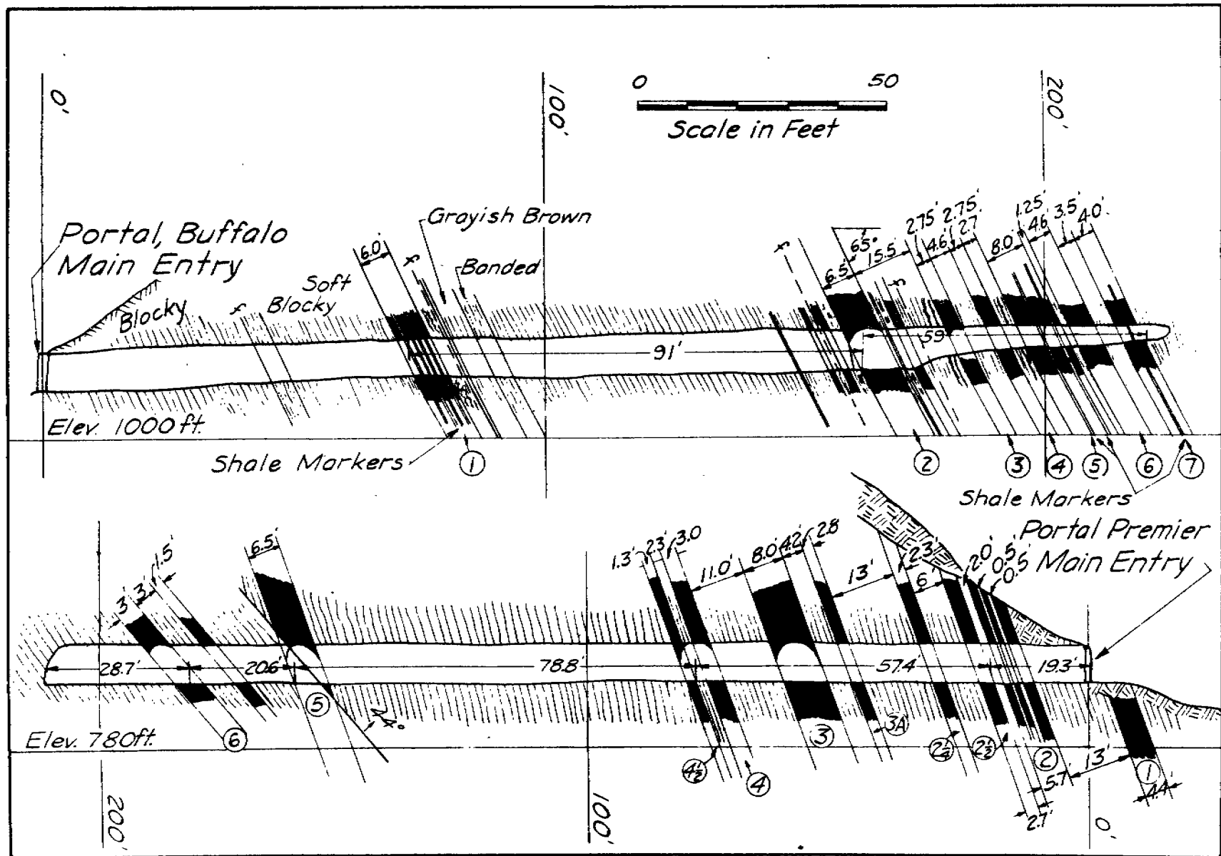
FIGURE 17.- Sections through Buffalo and Premier beds.
