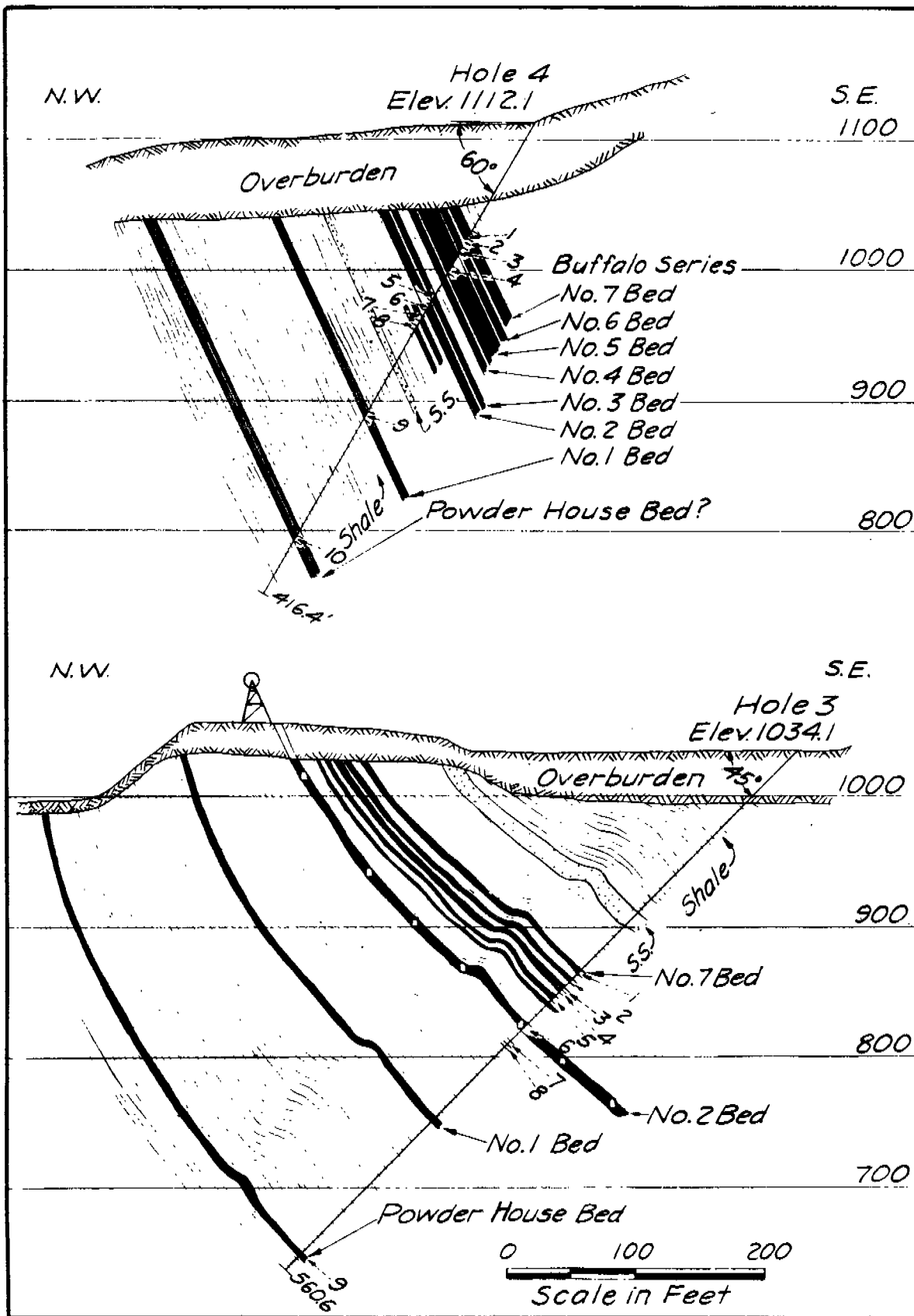
FIGURE 14.- Sections through diamond drill holes 3 and 4.
