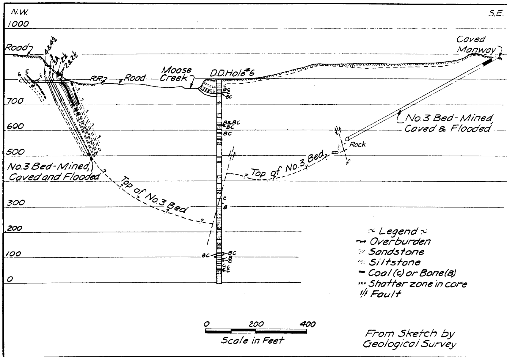
FIGURE 22.- Geologic section A-A' through diamond drill hole 6.
