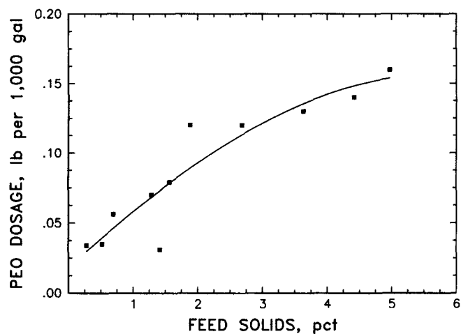
Figure 5.—Relationship between feed solids and PEO dosage, in pounds per 1,000 gal, at Olive Creek.
