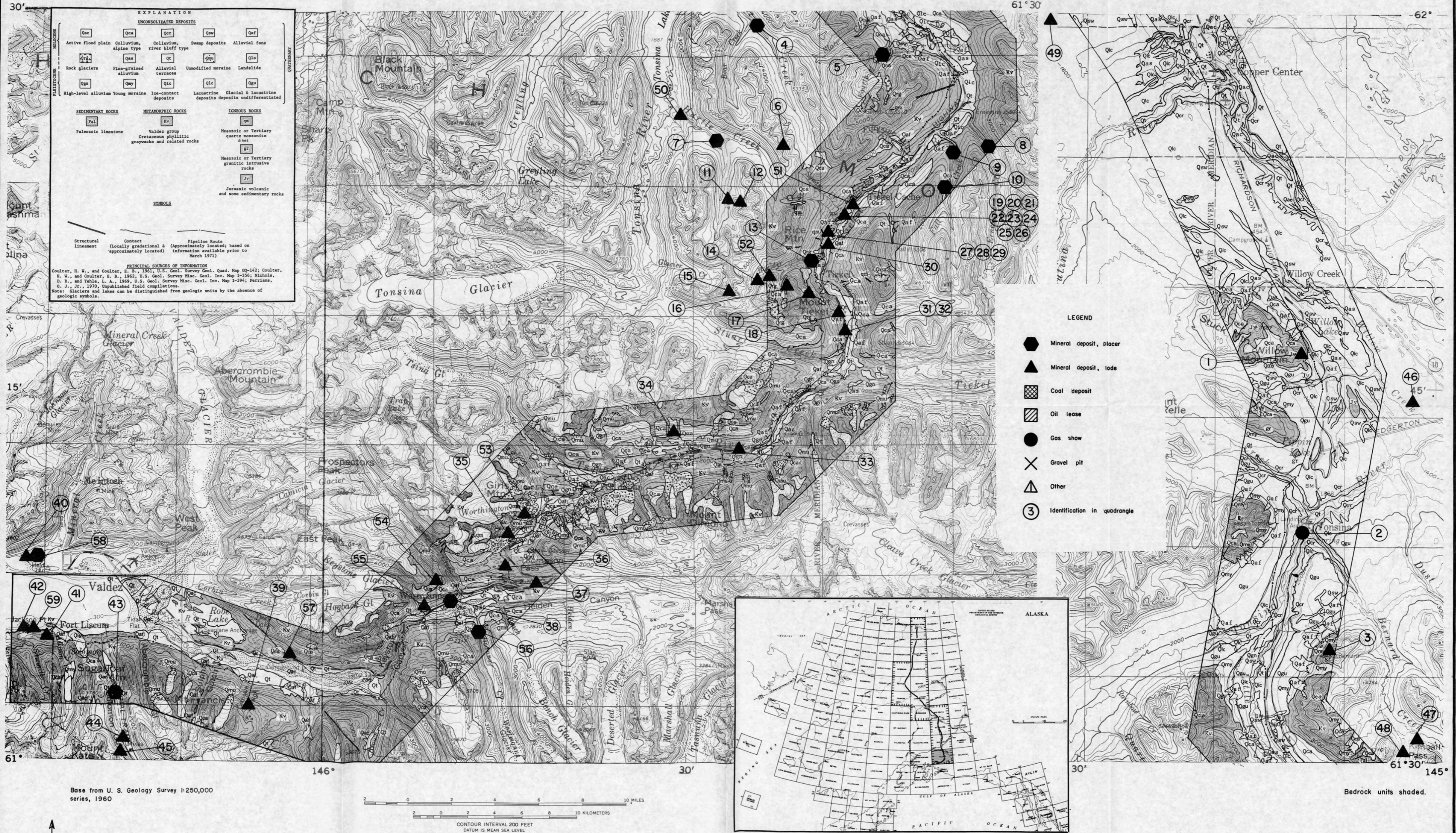
FIGURE 9. - Preliminary engineering geologic maps of the proposed Trans-Alaska Pipeline route, Valdez Quadrangle.
