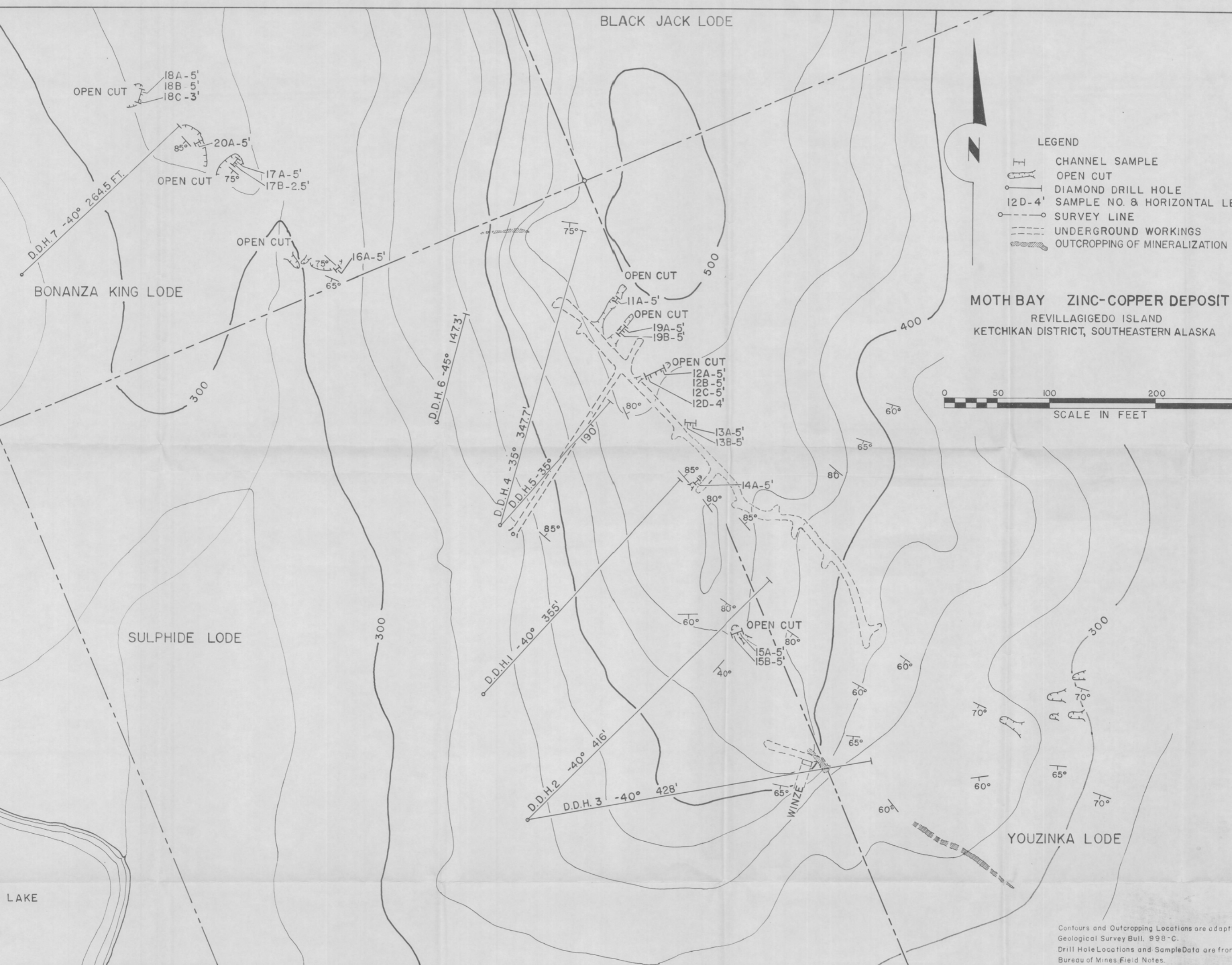
FIGURE 3.-TOPOGRAPHIC MAP SHOWING LOCATION OF DRILL HOLES, SURFACE SAMPLES, SECTIONS, CLAIMS AND UNDERGROUND WORKINGS
