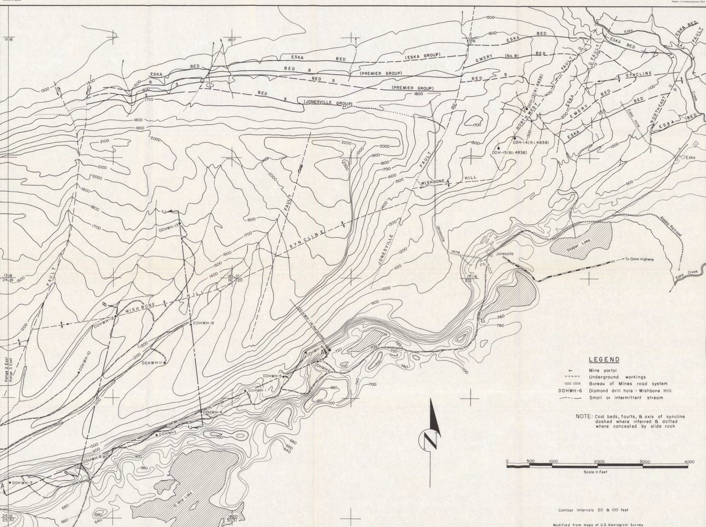
FIGURE 3. - Plan, Central Part of Wishbone Hill District.
