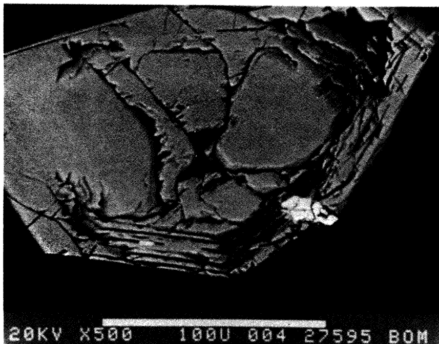
Figure 12. - SEM backscatter electron photomicrographs of heavy mineral concentrate from upper No Name Creek. Top photograph shows ilmenite (A) as light gray, cassiterite (B) as white , zircon (C) exhibits an inclusion of monazite (E), and xenotime (D) shows as cream color. Other darkcolored grains are silicate gangue minerals. The bottom photograph is an enlargement of the zircon grain with monazite inclusions.
