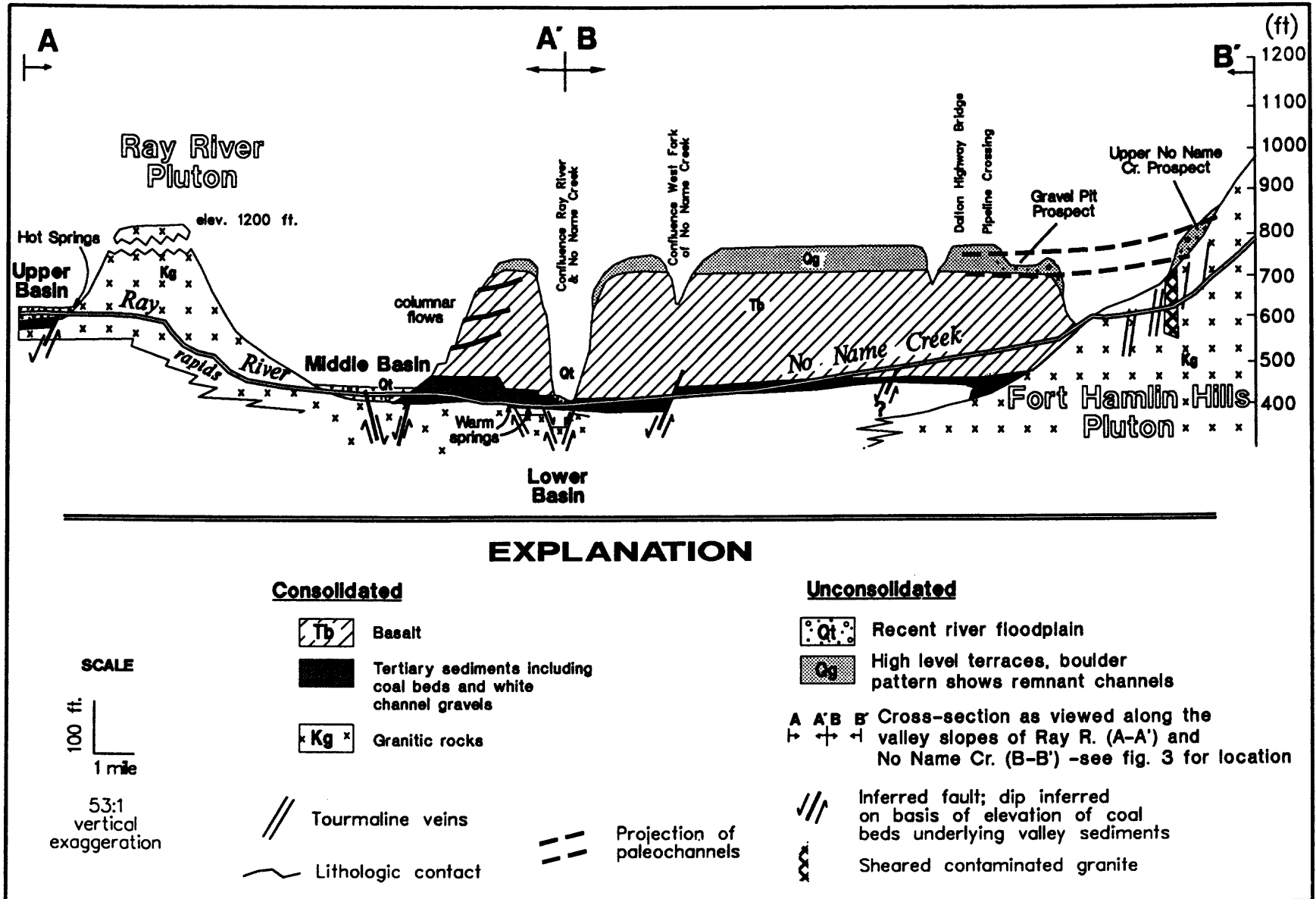
Figure 5. - Interpretive valley floor profile of No Name Creek and Ray River.
