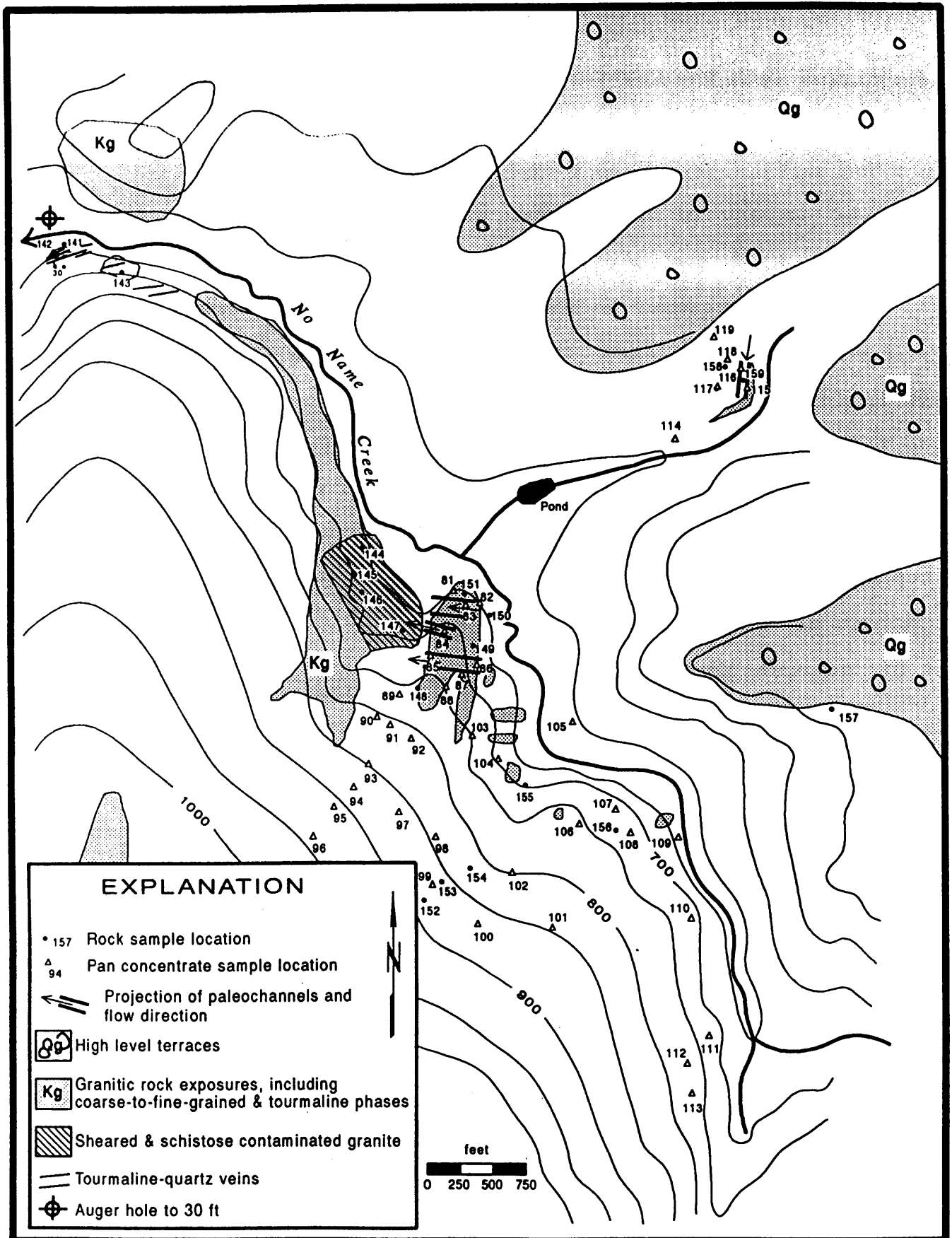
Figure 9. - Upper No Name Creek prospect.
