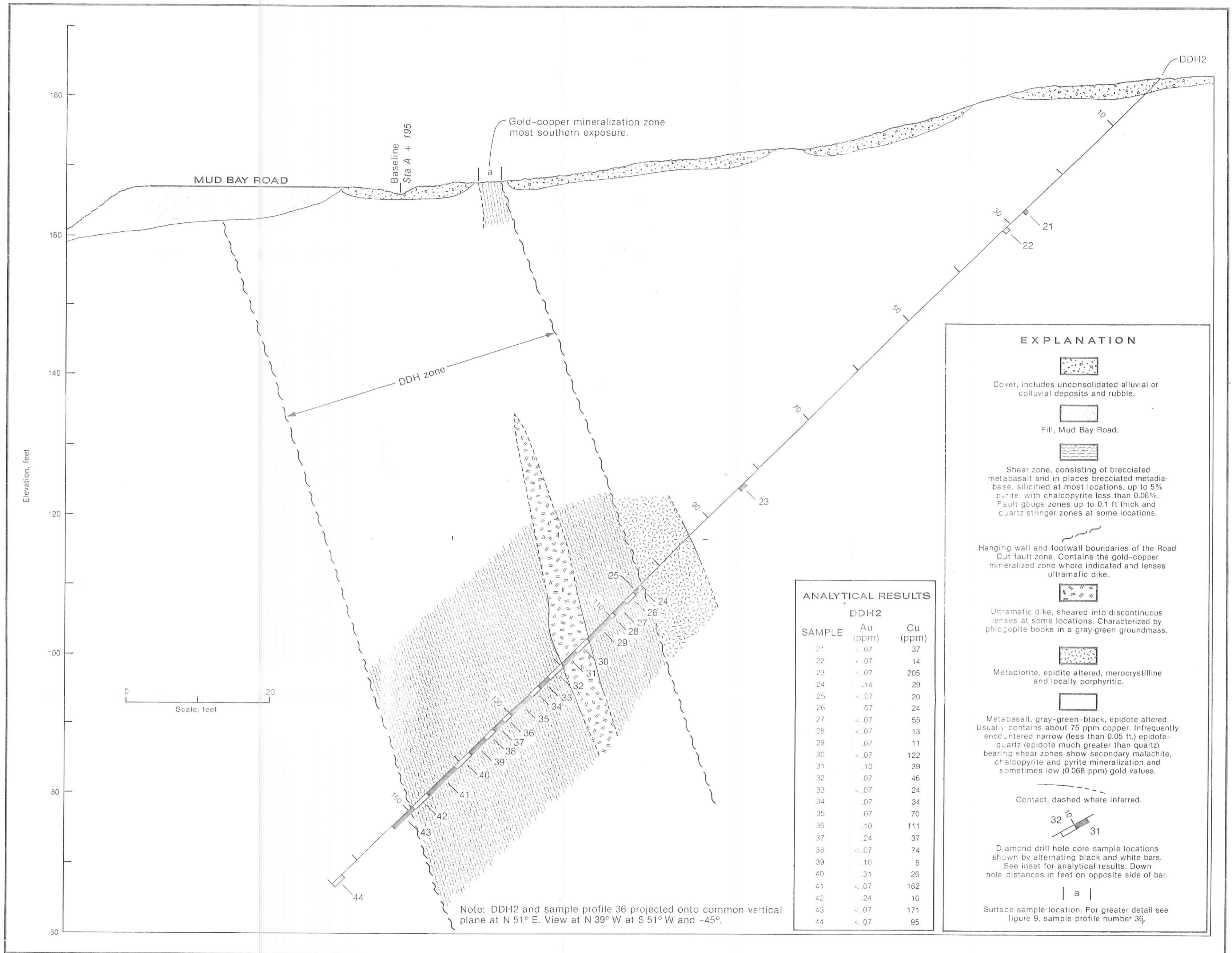
Figure 13.— Road Cut prospect vertical cross-section XS4, showing DDH2 and surface sample profile 36.
