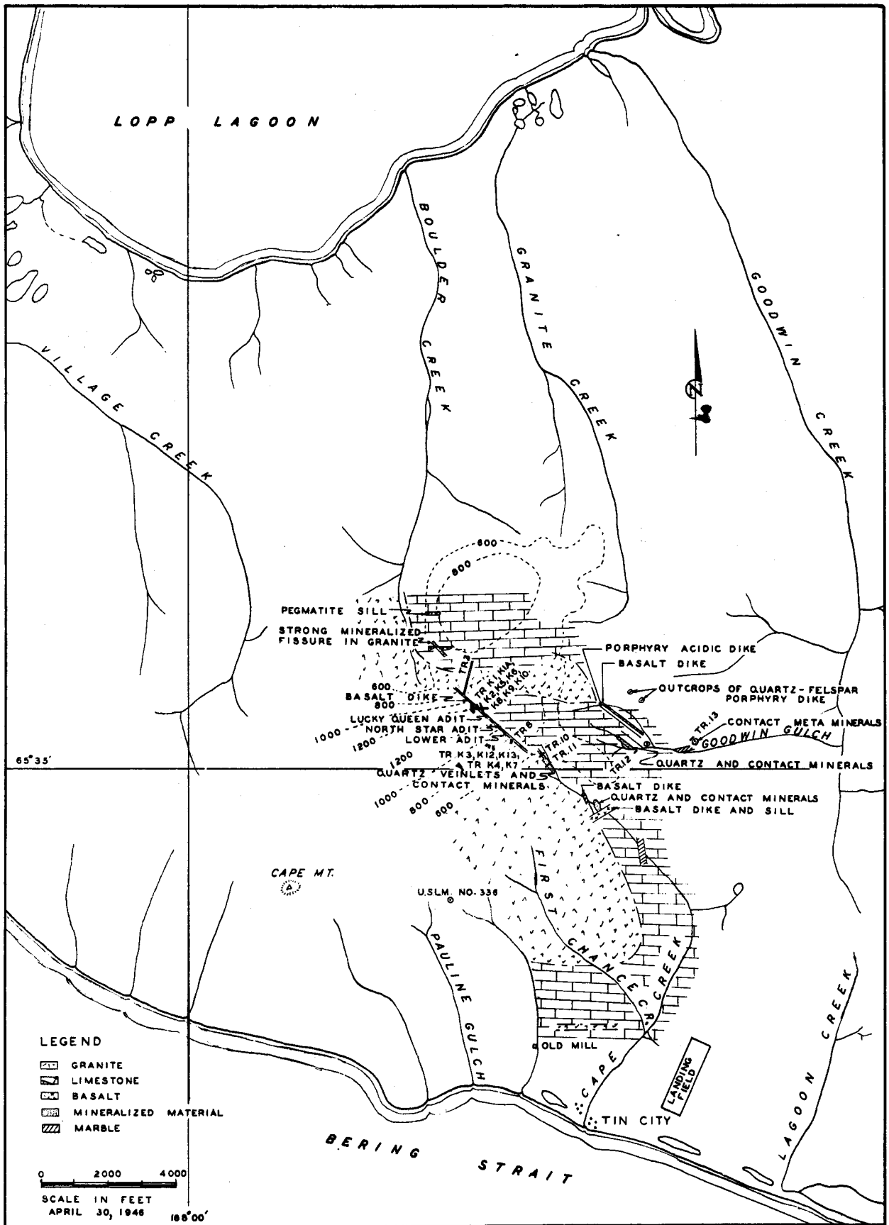
FIG. 2.— CAPE MOUNTAIN LODE-TIN DEPOSIT, SEWARD PENINSULA.
