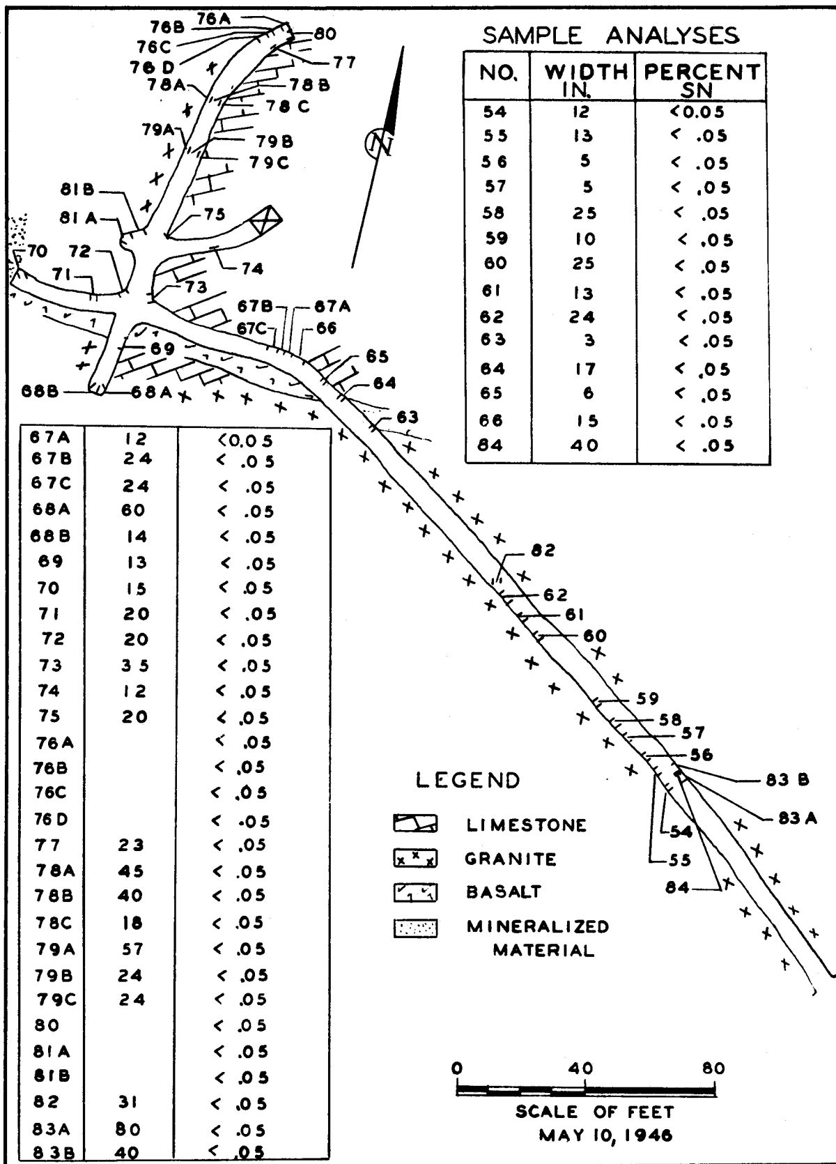
FIG. 7.- LOWEST ADIT, BARTELL MINE, SEWARD PENINSULA.
