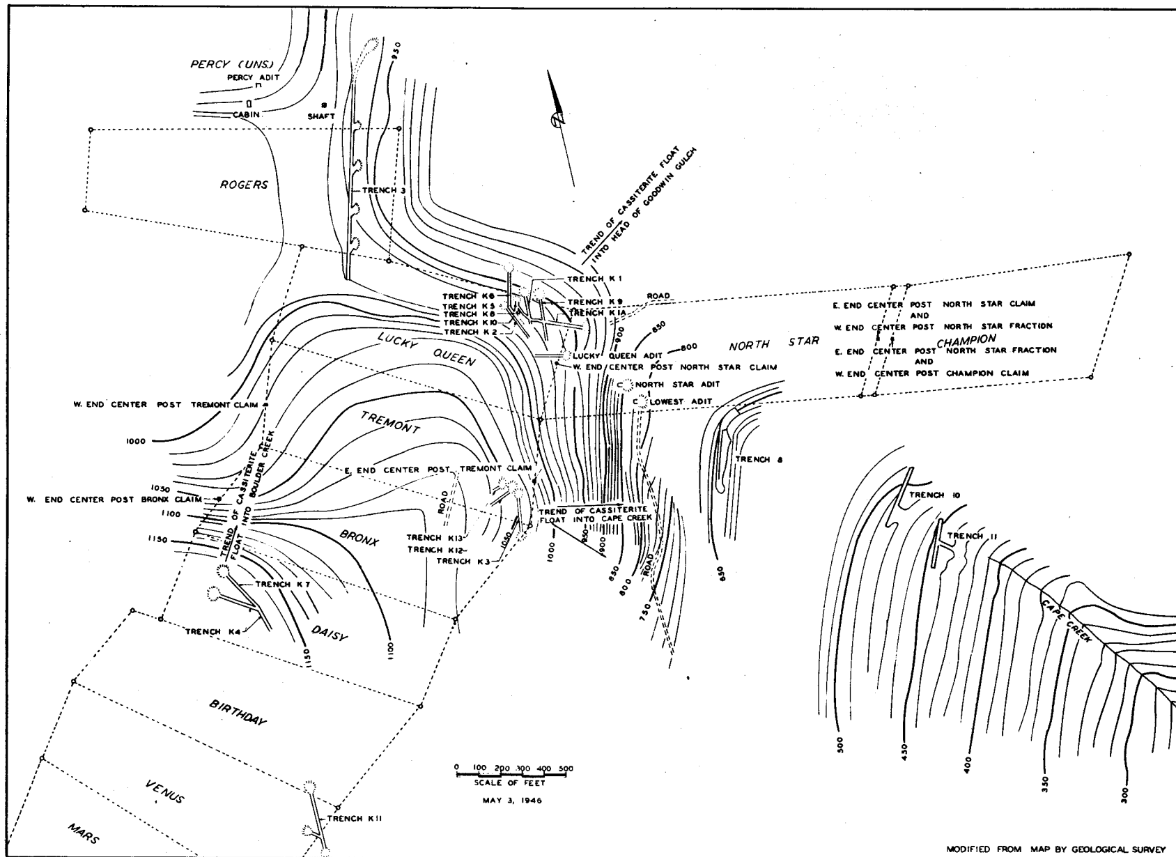
FIG. 3.— LOCATION OF TRENCHES AND ADITS AT CAPE MOUNTAIN LODE-TIN DEPOSITS, SEWARD PENINSULA, ALASKA.
