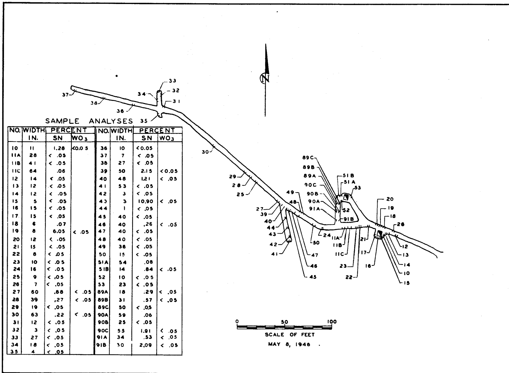
FIG.5-LOCATION AND ANALYSES OF SAMPLES IN BARTELL MINE -NORTH STAR ADIT
