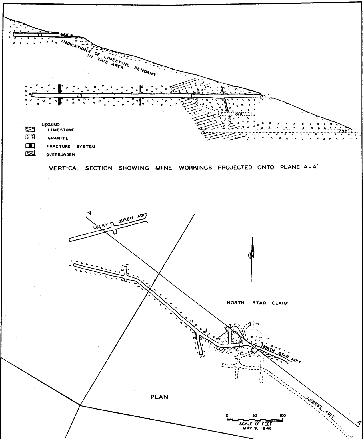
FIG. 4.-PLAN AND SECTIONAL VIEW, BARTELL MINE, CAPE MOUNTAIN, SEWARD PENINSULA, ALASKA.
