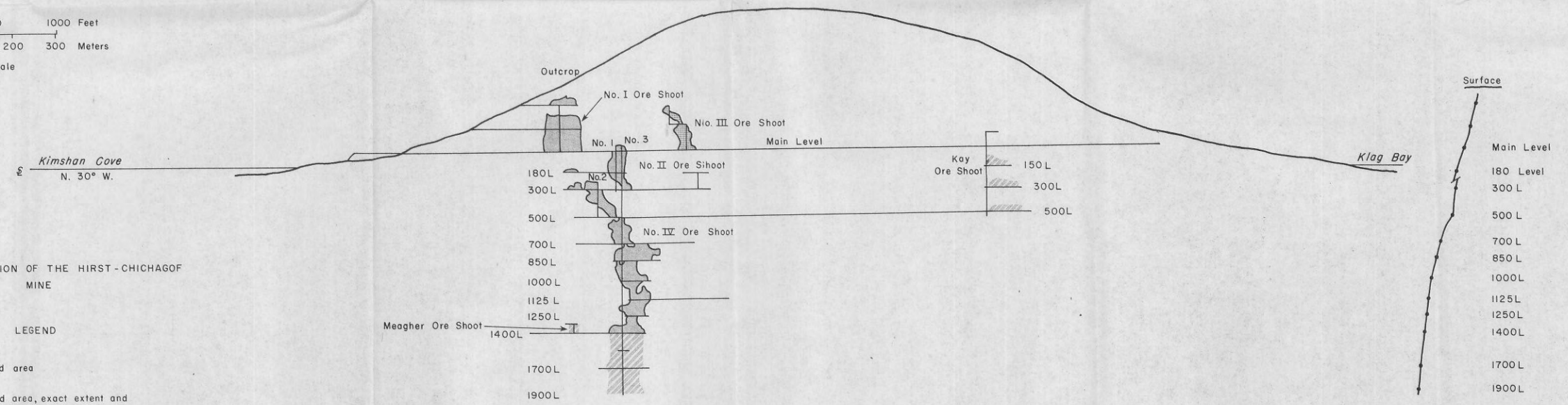
Cross Section At No. 3 Shaft And Through Ore Shoot No. I Raise. Looking NW
