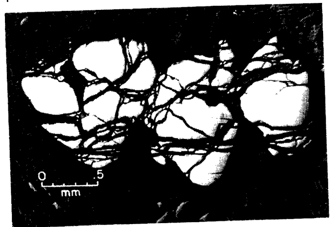
FIGURE 6. - Photomicrograph of polished section showing well-developed lineation defined by alignment of chromite grains and parallel internal fractures.
