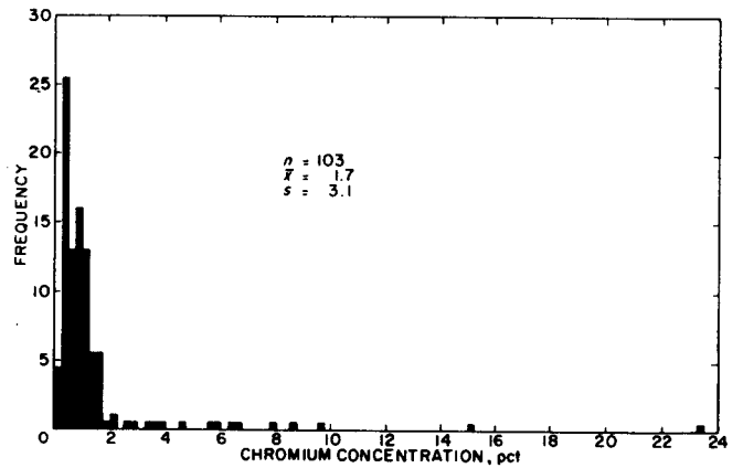
FIGURE 16. - Histogram for chromium in 103 rock samples.
