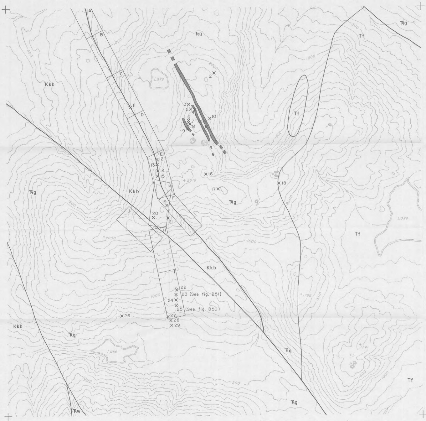
Plate 12.—Slocum Arm molybdenum prospect, sample locations.
