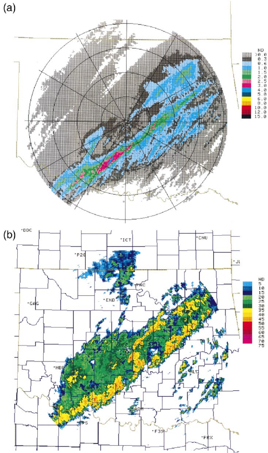
FIG. 1. (a) Oklahoma City, OK, WSR-88D storm total precipitation and (b) base reflectivity products on 4 Nov 1994 for range coverage of 124 n mi (230 km). (a) 1136–1757 UTC. Resolution is 1.1 n mi \times 1.1 n mi (2 km \times 2 km). Maps displayed are range rings at 30 n mi (55.65 km) intervals, radial sector
