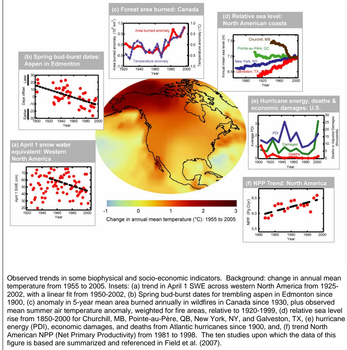
Figure 14.1: North American Observations (Field et al., 2007)
