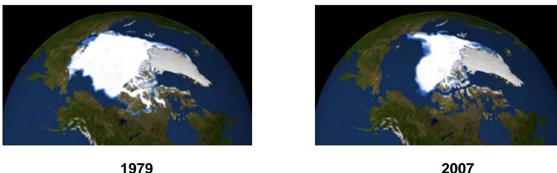
Figure 4.6 Arctic Sea Ice Concentrations Comparisons
