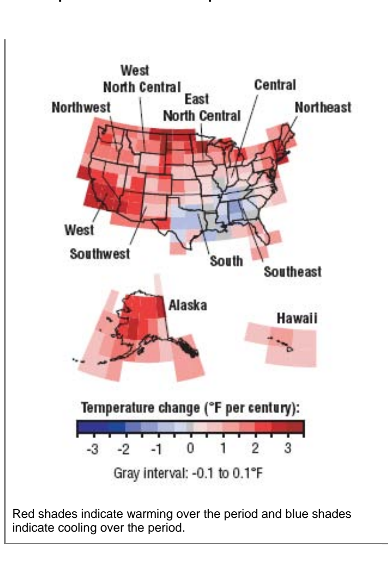
Figure 4.4: Map of the United States, depicting regional U.S. temperature trends for the period 1901 to 2006.
