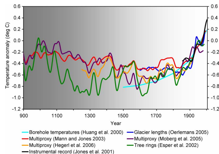
Figure 4.3: Reconstructions of (Northern Hemisphere average or global average) surface temperature variations from six research teams
