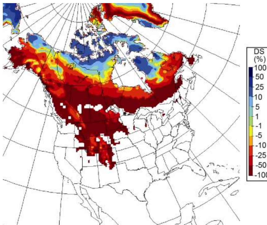
Figure 6.11 Percent Snow Depth Changes in March
