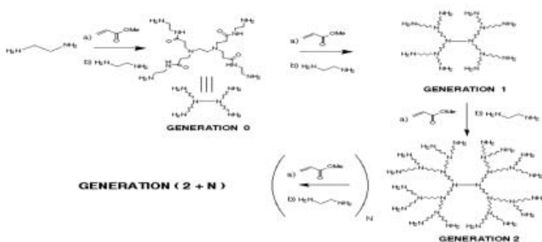
Figure 1. Structures of PAMAM dendrimers with ethylene diamine core and terminal \text{NH}_2 groups.
