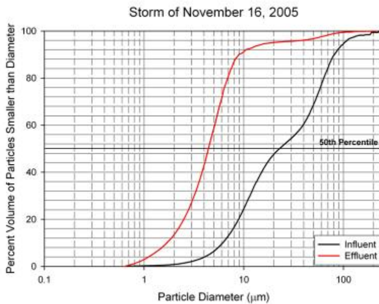
Figure 5-2. Coulter analysis comparison by volume of the Terre Kleen™ influent and effluent particle volume for Event 8.
