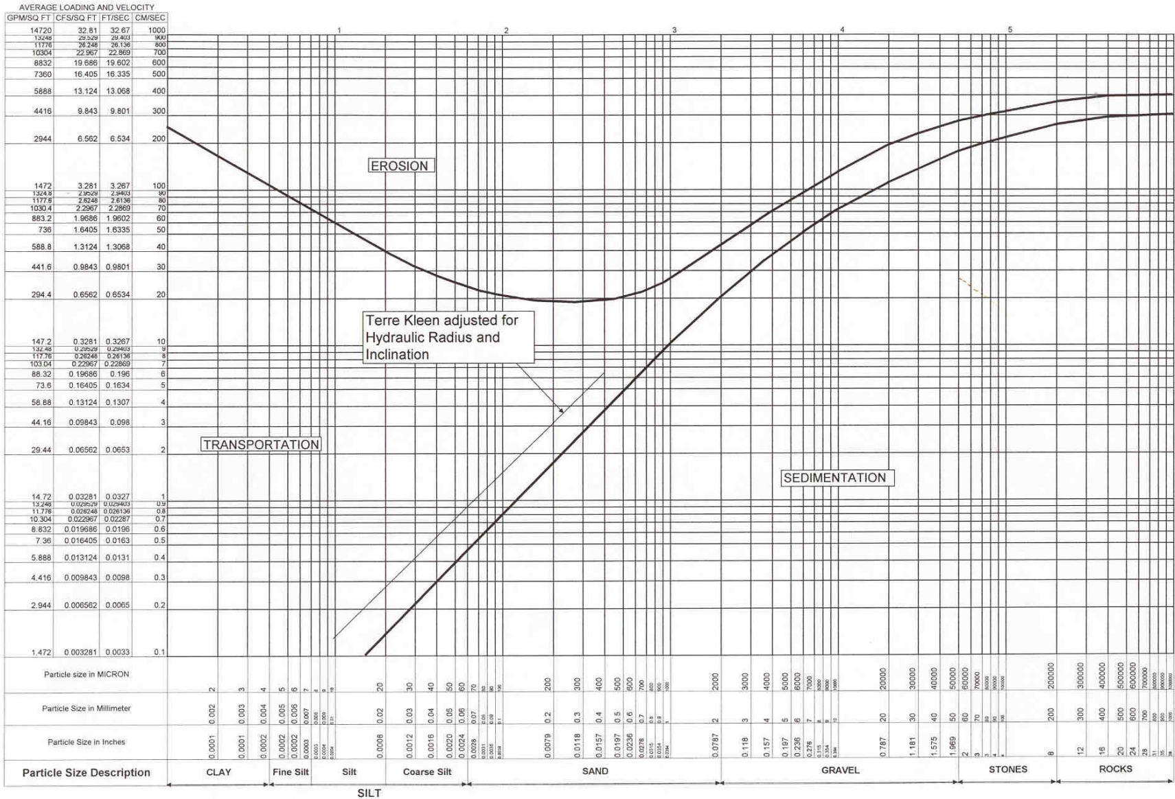
Figure 2-2. Adjusted Hjulstrom diagram (provided by vendor).
