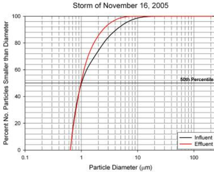
Figure 5-1. Coulter analysis comparison by count of the Terre Kleen™ influent and effluent total particle count for Event 8.
