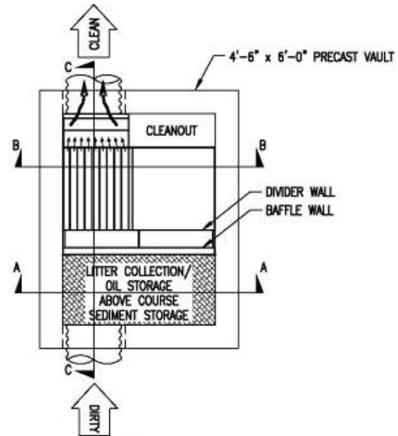
PLAN VIEW WITHOUT LID
