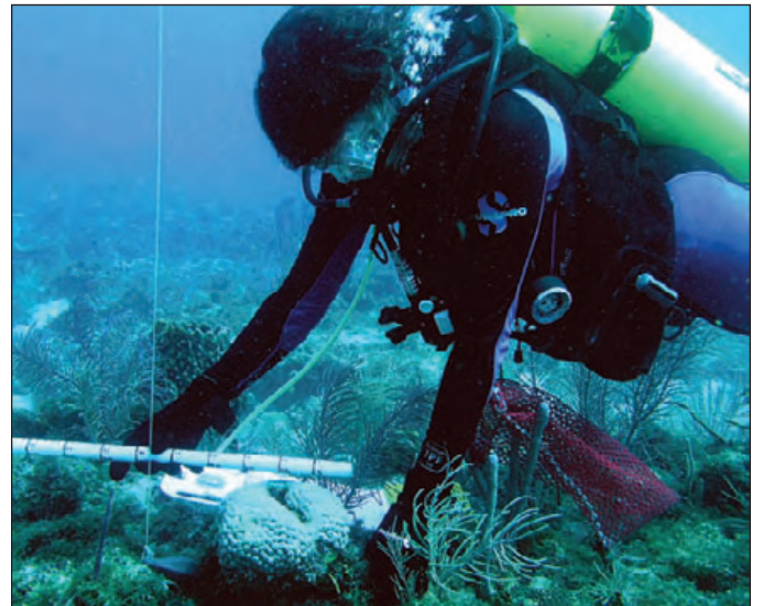
Figure 3-1. Colony size has been quantified by visual grading into volumetric size classes (left). In this example colony ( Diploria strigosa ), volume was better approximated by the larger 10L cube than the 1L cube. The surface area assigned to this colony (five sides of the 10L cube) was 2,311.3 cm 2 . Colony size can also be quantified by actual field measurement of height (h), diameter (d), and width (w) from an aerial view (right). When analyzed photographically (Appendix A) this colony measured h = 22.9 cm d = 36.1 cm and w = 29.8 cm, with a surface area of 1,976.9 cm 2 .
