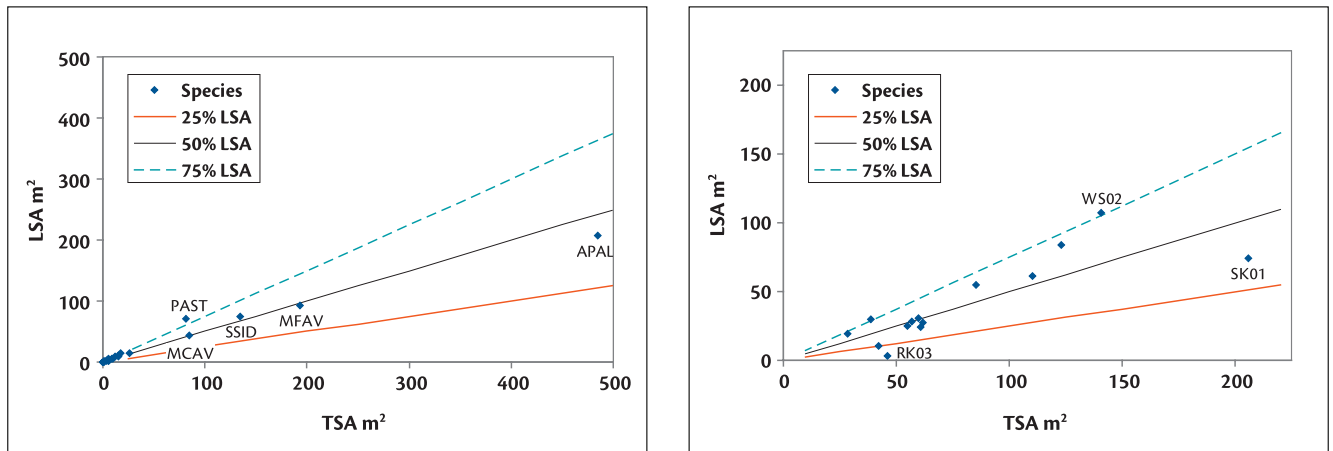
Figure 4-3. Comparison of TSA and LSA ( m^2 ) documented for different species (left) and stations (right) from surveys performed at 14 stations near Key West, Florida. Lines represent 25%, 50% and 75% values for %LSA. Elkhorn coral, Acropora palmata (APAL) had the greatest TSA of all species encountered at these stations, but %LSA was less than 50%. Other species, including Montastraea faveolata (MFAV), Siderastrea siderea (SSID), M. cavernosa (MCAV) and Porites astreoides (PAST) provided substantial surface area to the reef. The PAST population retained a %LSA greater than 75%. Station SK01 had the highest TSA but less LSA than station WS02. Percent LSA was less than 25% for station RK03 and greater than 75% for WS02. Source: Fisher et al. (2007b).
