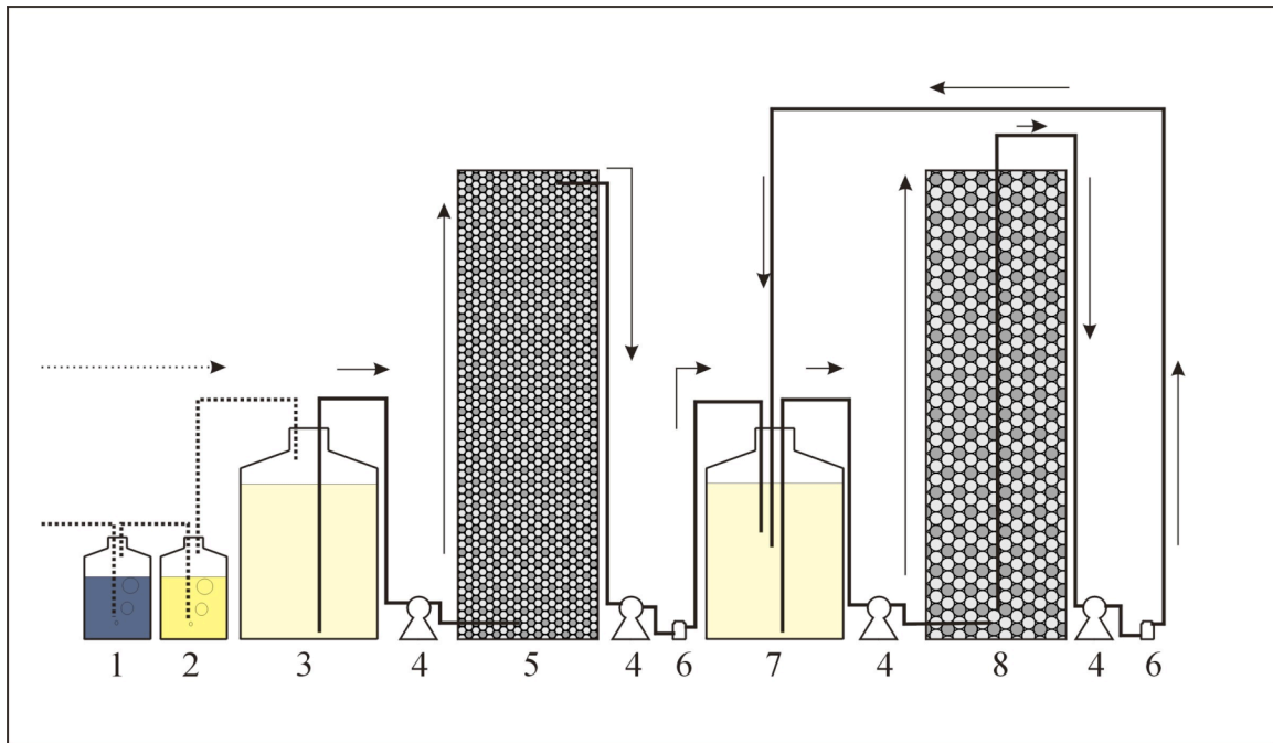
Figure 9.1. Water flow diagram for column studies. Acrilic tubing was used to make the columns. (1) Pyrogallol 6 % under KOH 30 % alkaline solution medium for absorbing oxygen, (2) 15 % ascorbic acid solution for absorbing oxidants, (3) Raw ground water tank, (4) Peristaltic pump, (5) Pre-treatment column, (6) Effluent bottle for sampling and measuring, (7) Storage container, (8) Main test columns comprised of two water level fluctuation simulation columns and one continuous flow column, Two types of flow direction were tested (see Figure 9.2.) for main columns. (9) Outside nitrogen shielding box to keep air out. The inner diameter of column is about 5 in. Dotted arrow line indicates air flow, and solid arrow lines indicate water flow.
