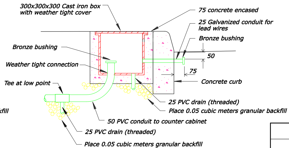
SPLICE BOX - WITH CURB
