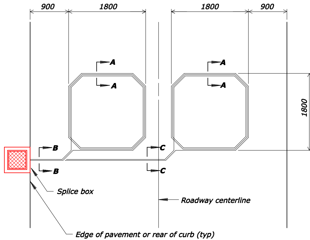
SCHMATIC OF VEHICLE LOOP DETECTORS
