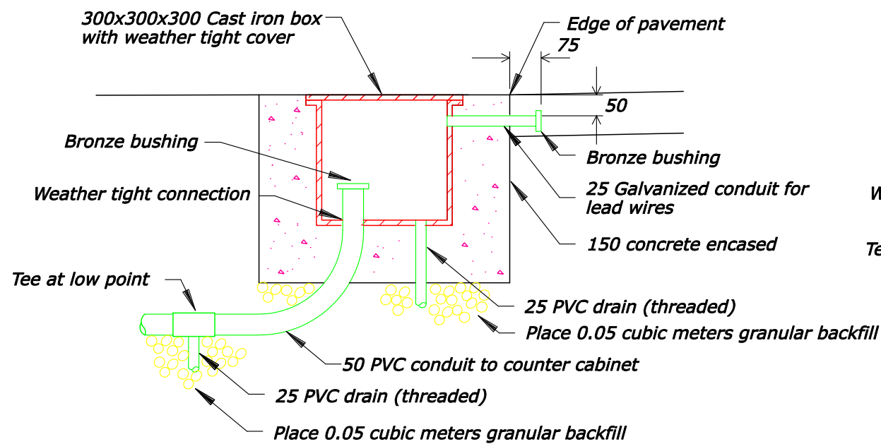
SPLICE BOX - WITHOUT CURB
