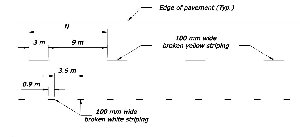
BROKEN SINGLE YELLOW AND DOTTED WHITE STRIPING
