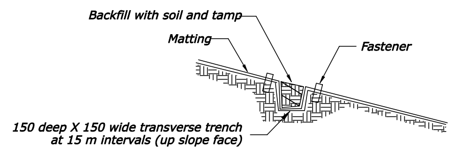
SECTION A-A Erosion Stop (Check Slot) Detail
