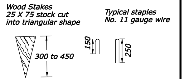
DETAIL A Typical Ground Fasteners
