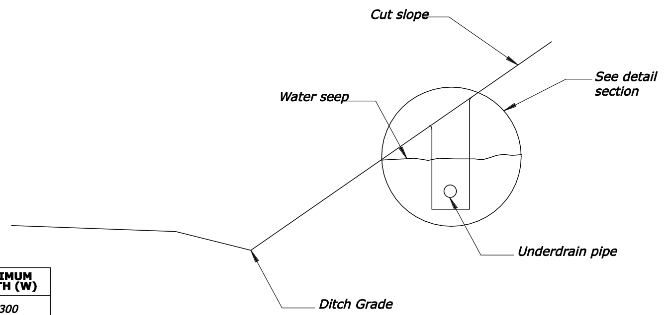
CROSS SECTION
