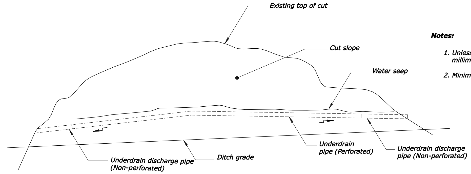
PROFILE VIEW
