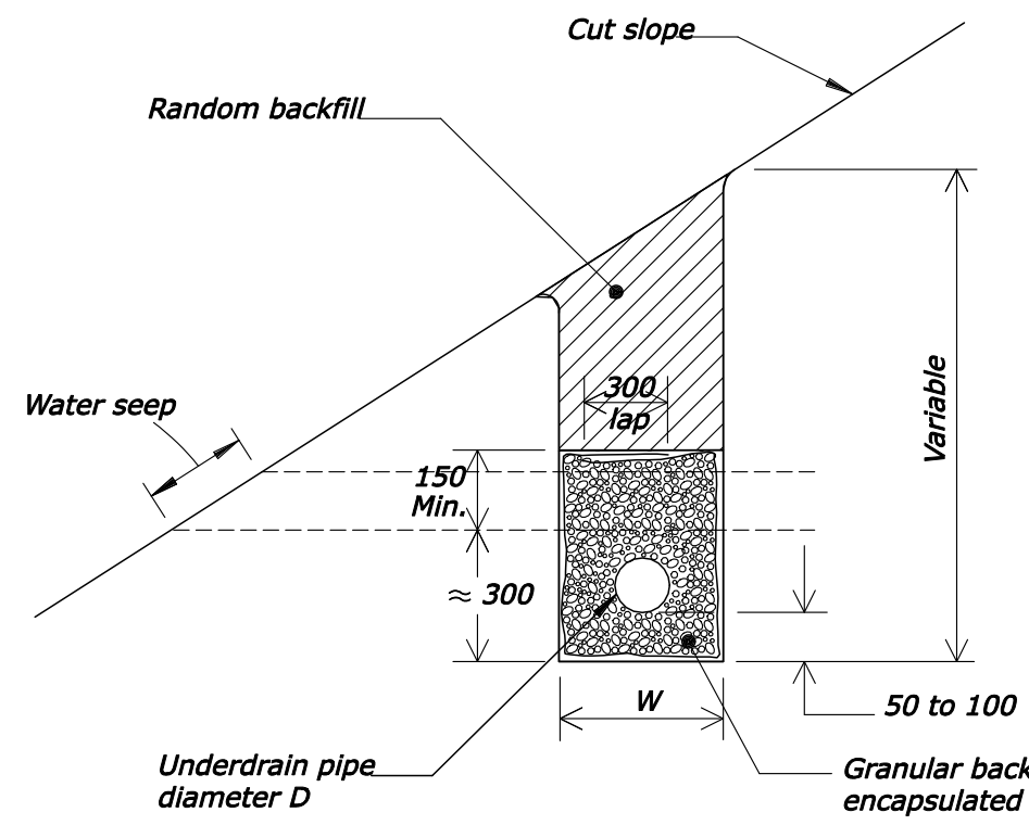
DETAIL SECTION
